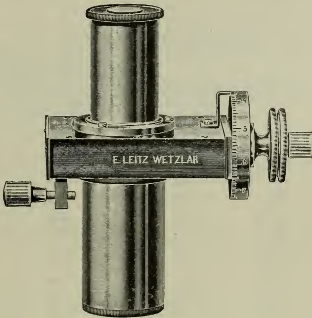
FIG. 207.—Screw micrometer eyepiece (Filar micrometer).
