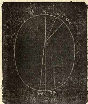
FIG. 68.—Diagram for Kepler's Laws.
