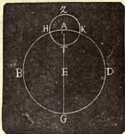
FIG. 67.—The Circle and the Epicycle.
