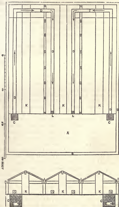
Fig. 13.—GREEN-HOUSE HEATED BY FLUES.
