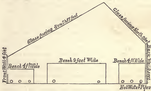
Fig. 44.—END SECTION OF ROSE-HOUSE.
