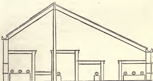
Fig. 19.—INTERIOR OF FORCING HOUSE.
