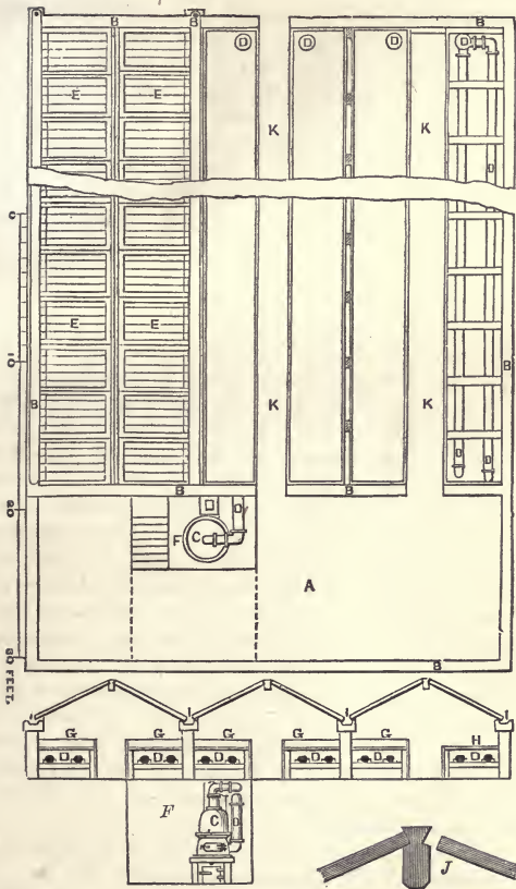
Fig. 12.—GREEN-HOUSE HEATED BY HOT WATER PIPES.
