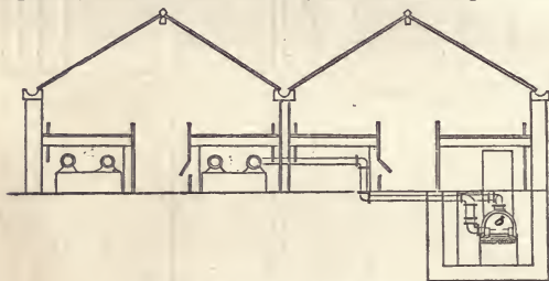
Fig. 15.—END VIEW OF FIGURE 14.
