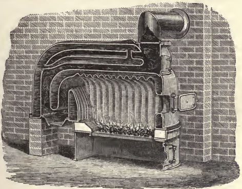
B.—Longitudinal Section of Boiler.
