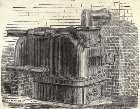
A.—Elevation of Boiler.
