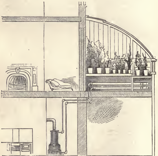
Fig. 24.—SECTION OF HOUSE AND CONSERVATORY.
