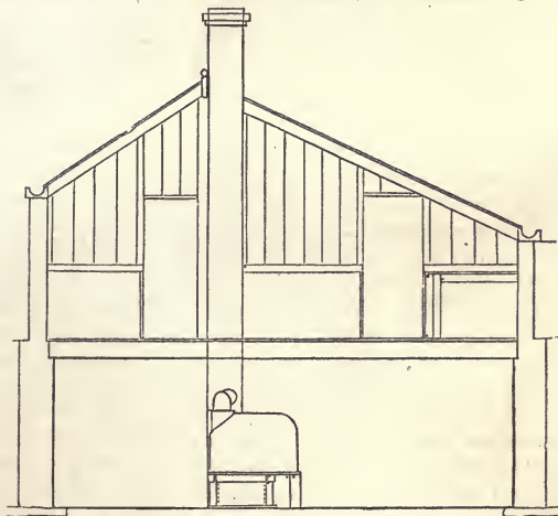
Fig. 16.—END VIEW OF FORCING HOUSE.
