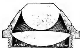
FIG. 47.—Optical part of Abbé illuminator.
