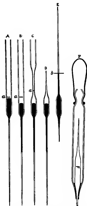
FIG. 19.—Making throttle pipettes—large capacity
