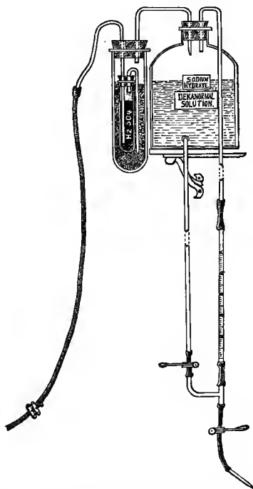
FIG. 99.—Stock bottle for deka-normal soda solution.
