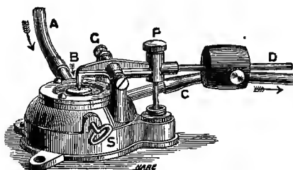
FIG. 116.—Capsule thermo-regulator.
