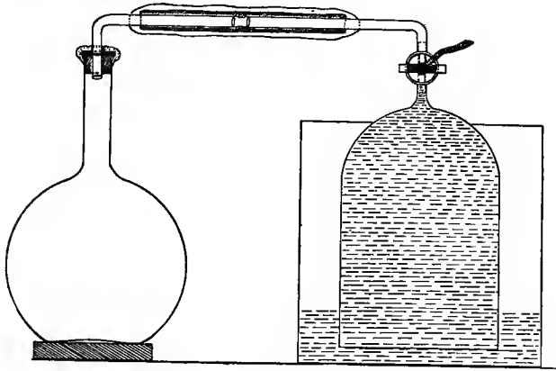
FIG. 153.—Gas-collecting apparatus.
