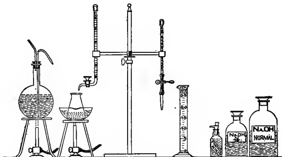
FIG. 97.—Arrangement of apparatus for titrating media.
