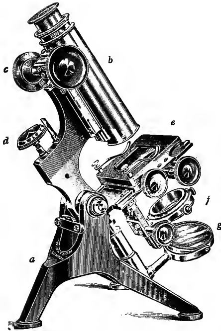
FIG. 40.—Microscope stand.
