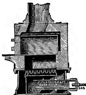
FIG. 25.—Muffle furnace.
