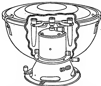
FIG. 162.—Small electrical centrifuge.
