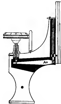
FIG. 43.—Fine adjustment.
