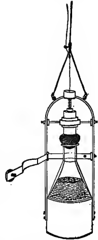
FIG. 203.—Esmarch's collecting bottle for water samples.
