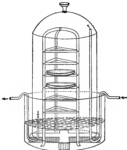
FIG. 134.—Botkin's apparatus.
