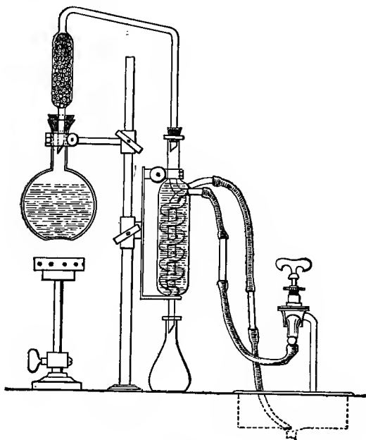
FIG. 152.—Arrangement of distillation apparatus for acids, etc.
