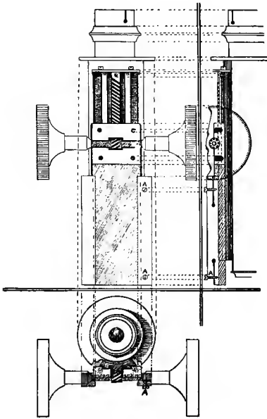
FIG. 42.—Coarse adjustment.
