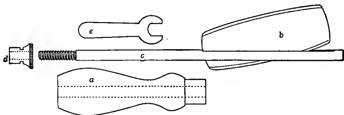
FIG. 11.—Glass-cutting knife. a . handle. b . double edged blade. c . shaft. d . locking nut. e . spanner for nut.
