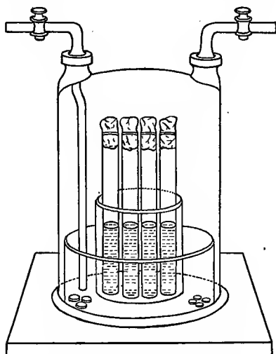
FIG. 137.—Bulloch's jar.
