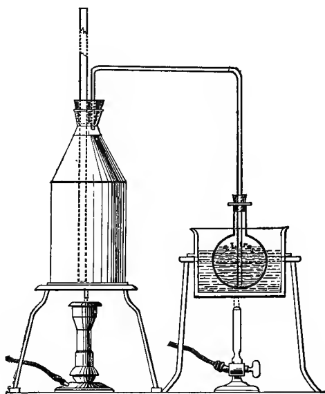
FIG. 108.—Arrangement of steam can and water-bath for the preparation of media.
