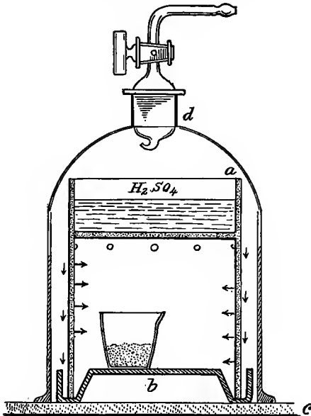
FIG. 157.—Mueller's desiccator.
