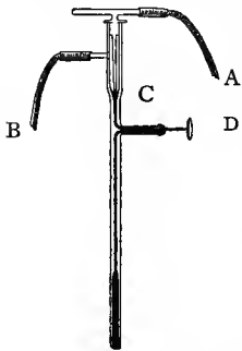
FIG. 115.—Reichert's thermo-regulator.
