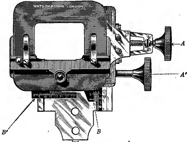
FIG. 45.—Mechanical stage.
