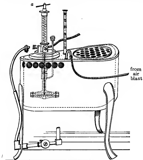
FIG. 155.—Hearson's water-bath.
