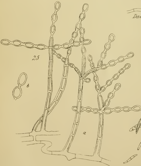
Penicillium subtile.
