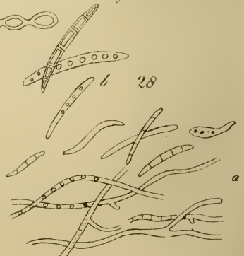
Fusisporium nudum.
