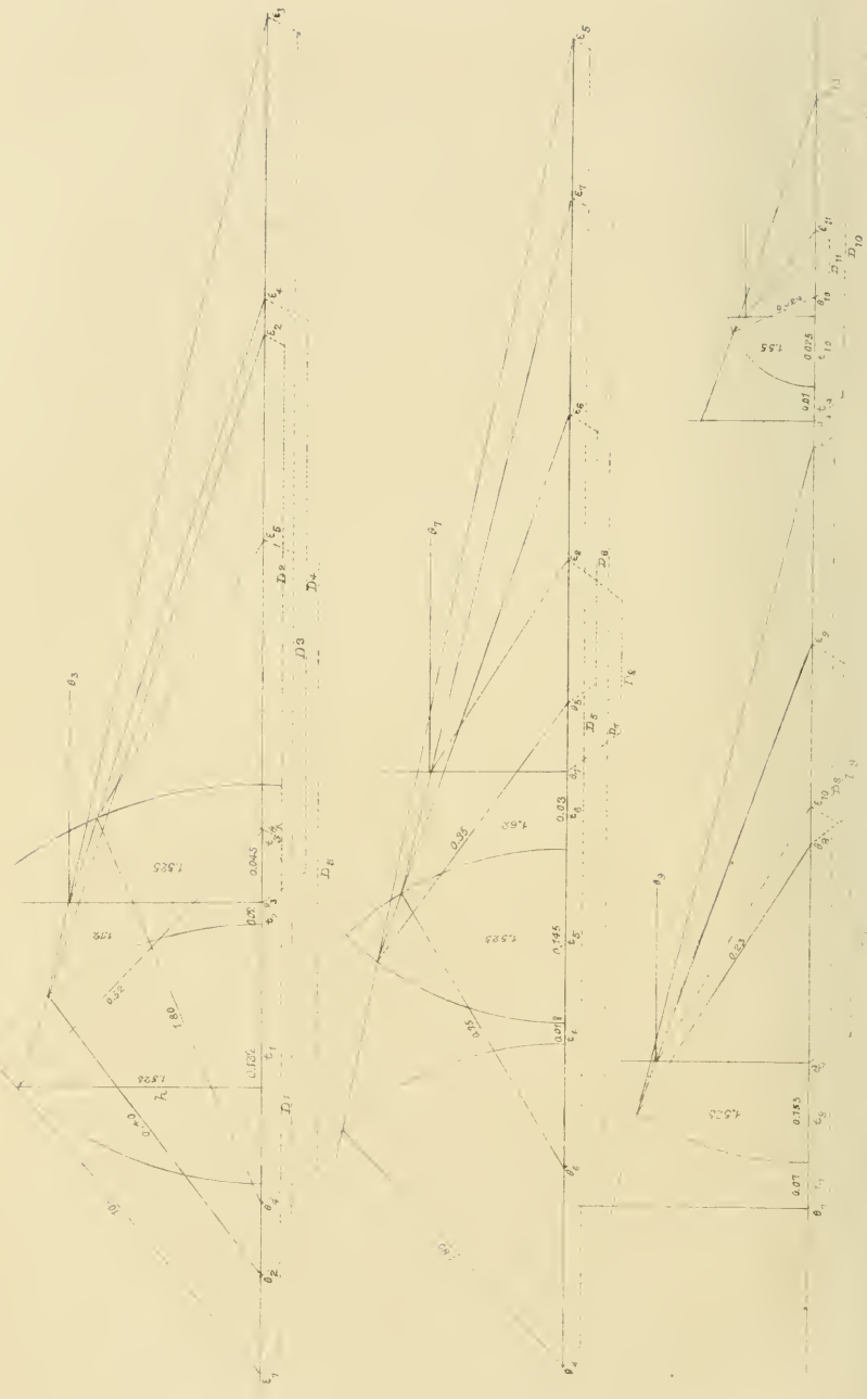
Diagrams exhibiting the path of a ray through Tolles' Immersion Objective.
