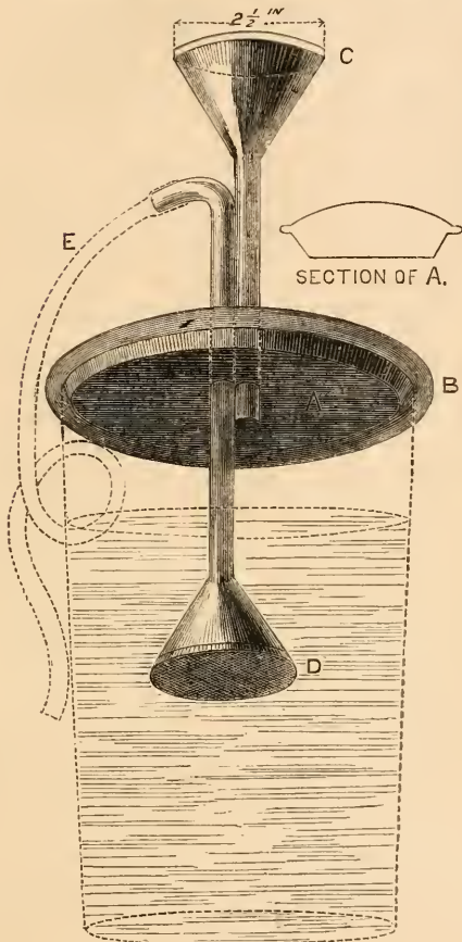
Fig. 81. Pond-side Filter.
