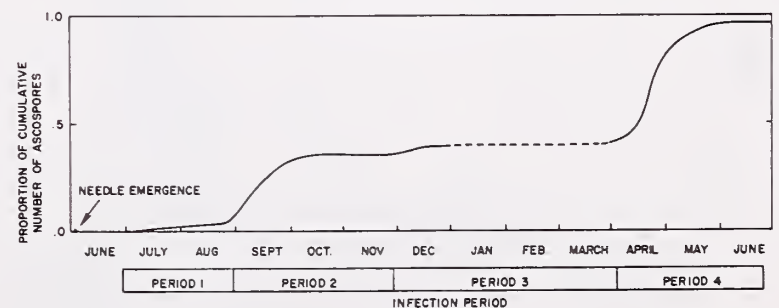
Figure 1.--Hypothetical Cyclaneusma minus inoculum availability curve for one year's complement of Pinus sylvestris needles in Pennsylvania. Dashed line indicates no spore trapping data exists from mid-December through March.
