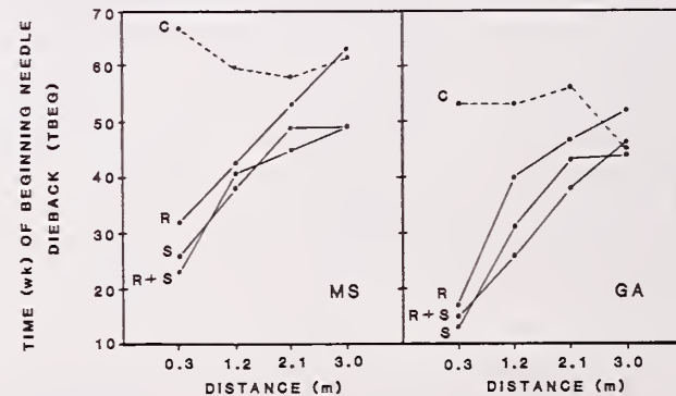
Figure 5.--Time (wk) of beginning brown spot needle dieback (TBEG) by distance (m) from initial infection focus for resistant (R), susceptible (S), mixed family (R+S), and control (C), plantings of longleaf pine in Mississippi (MS) and Georgia (GA).
