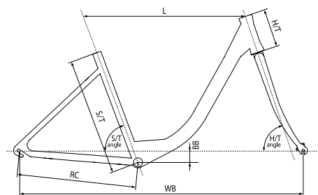
URBAN - CITY: AVENUE 30, AVENUE 10 Aluminum alloy monotube 26
