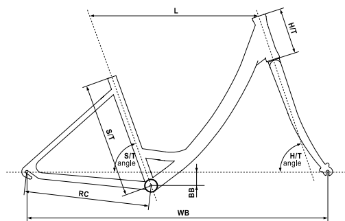
URBAN - CITY: AVENUE 50, AVENUE 20 Aluminum alloy monotube 28
