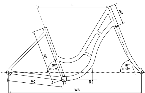
URBAN - CLASSIC: ROYAL DUTCH, ARWEN DUTCH, CLASSIC DUTCH van Kellys Dutch - Aluminum alloy 28
