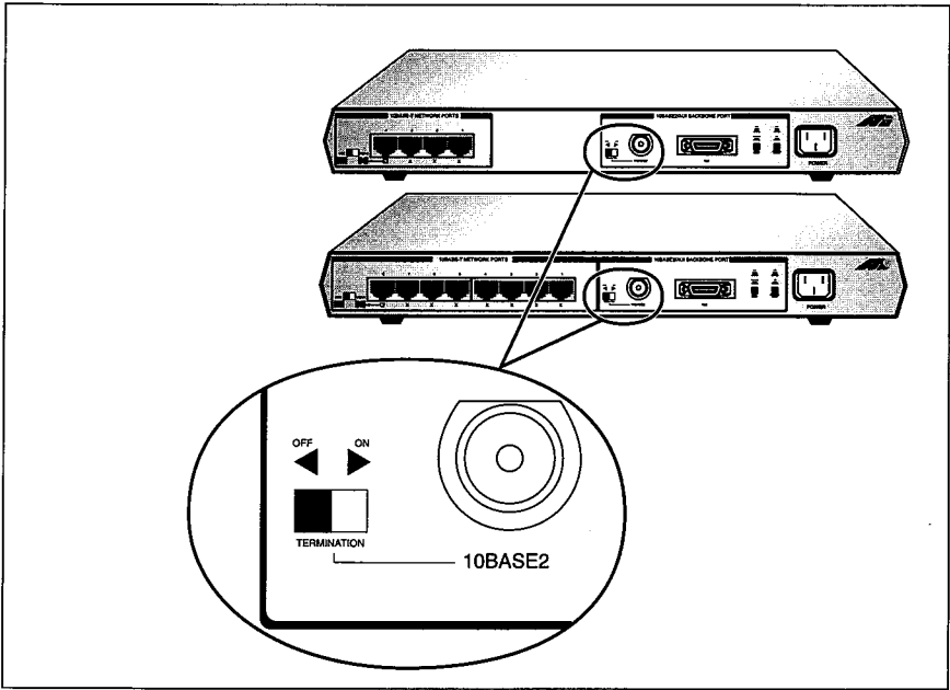
Figure 14: Terminator Switch
