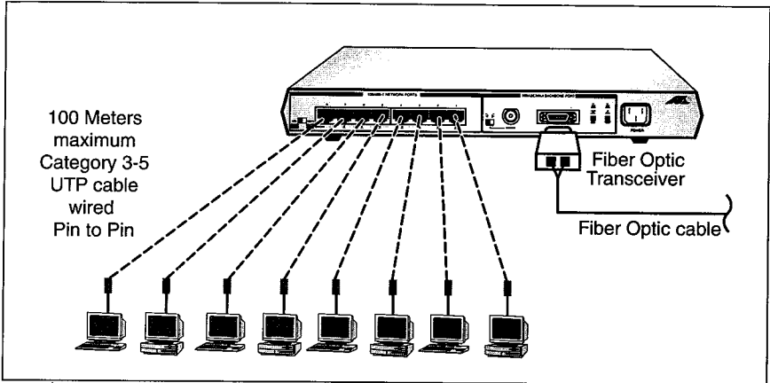
Figure 19: AT-MR820TR on a Fiber Optic Backbone
