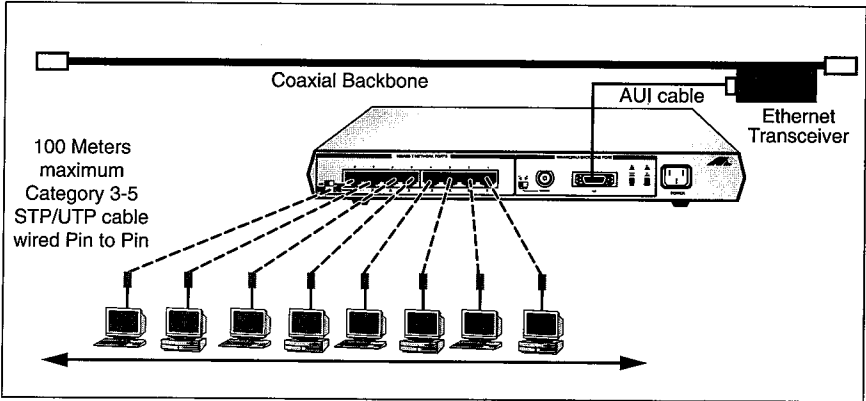
Figure 15: AT-MR820TR Backbone Topology
