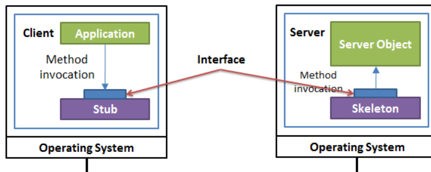
Obr. 6-8: Stub a Skeleton (Zdroj: http://lycog.com/distributed-systems/stub-skeleton/ )
