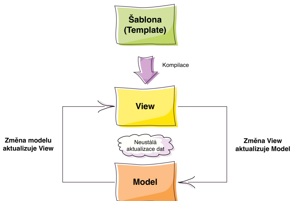
Obr. 9-11: Two-Way Data Binding
