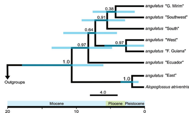
Figure 3. Species tree and divergence times inferred under a coalescent model with *BEAST for the lineages delimited by BPP. Node values correspond to posterior probabilities, and blue bars represent the 95% highest posterior density (HPD) intervals of divergence times (in millions of years).
