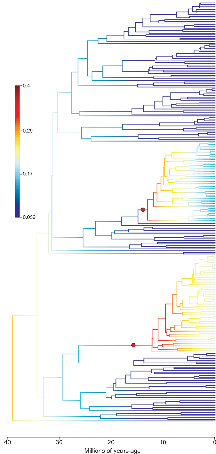
Figure 4. Best shift configuration sampled by Bayesian analysis of macroevolutionary mixtures (BAMM) for the naticrine phylogeny. Colours along the branches represent instantaneous rates of speciation, and the red circles represent shifts in the diversification regimes. These shifts are on branches leading to the North and Central American group (upper red circle) and one of the major Asian clades (lower red circle). For complete phylogeny, see Figure 2 . For complete geographical distribution information, see Figure 6 .
