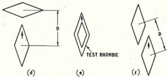
↑ denotes the test rhombic aerial D denotes distance between centres of aerials FIG. 13—RELATIVE POSITIONS OF RHOMBIC AERIALS
