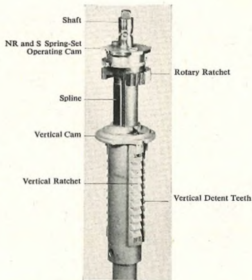
FIG. 3—RATCHET ASSEMBLY
