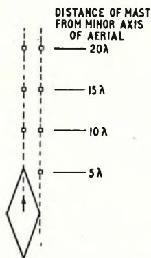
FIG. 12—POSITION OF MAST RELATIVE TO RHOMBIC AERIAL
