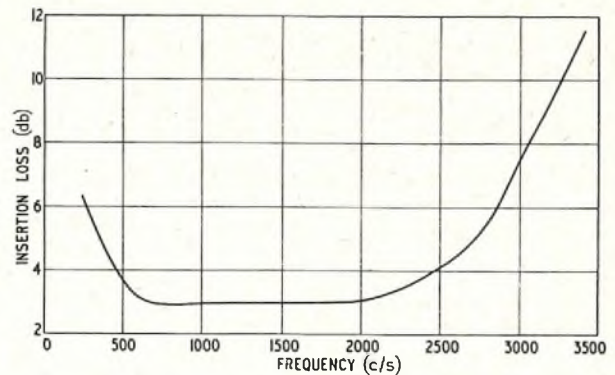
Circuit consisted of 28.5 miles of 20 lb/mile P.C.Q.T. cable loaded with 88 mH coils at 2,000 yd intervals
