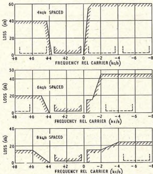
The requirements indicated are for single-sideband suppressed-carrier systems using lower-sideband 4 kc/s, 6 kc/s and 8 kc/s spaced carrier channels FIG. 1.—CHANNEL FILTER SPECIFICATIONS
