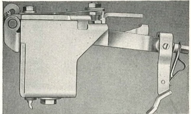
FIG. 5—ROTARY-MAGNET ASSEMBLY
