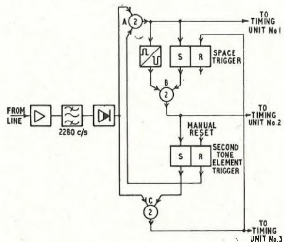
FIG. 6—THE 1 V.F. DETECTOR AND SEQUENCE CONTROL
