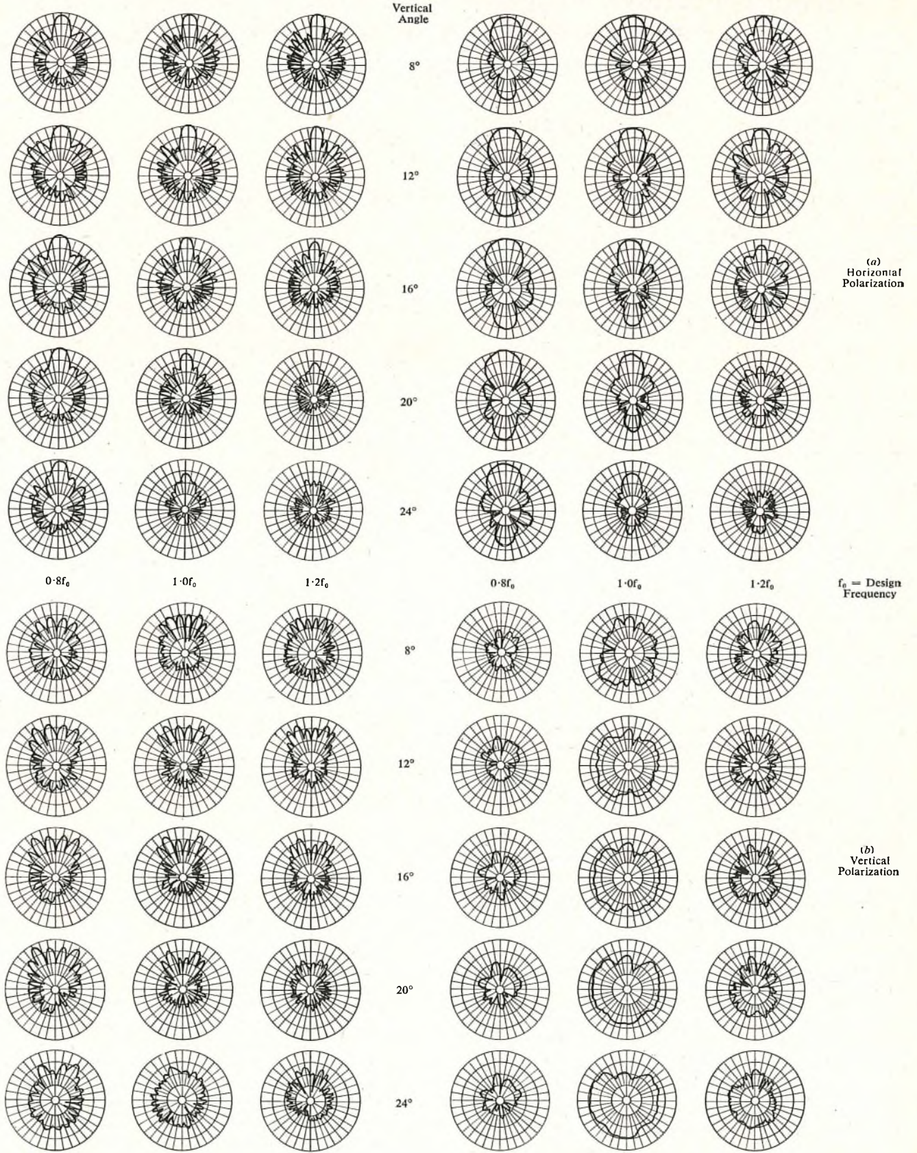
FIG. 9—AZIMUTHAL DIRECTIVITY CHARACTERISTICS OF RHOMBIC AERIAL AND HORIZONTAL ARRAY OF DIPOLES
