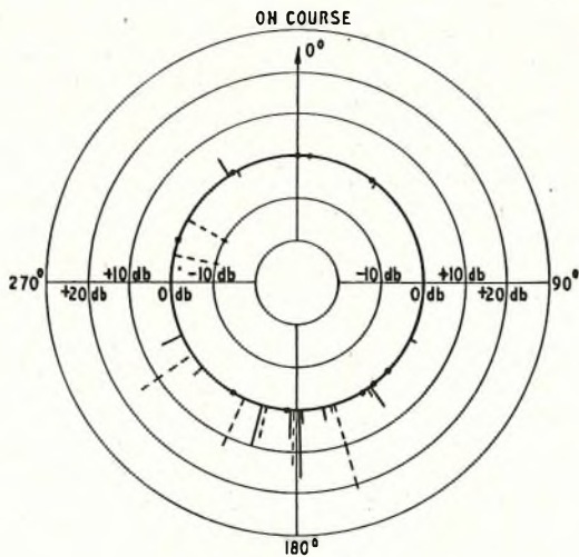
FIG. 10—RELATIVE PROTECTION RATIOS OF H.A.D. AND RHOMBIC AERIAL FROM RESULTS OF TRAFFIC OBSERVATIONS
