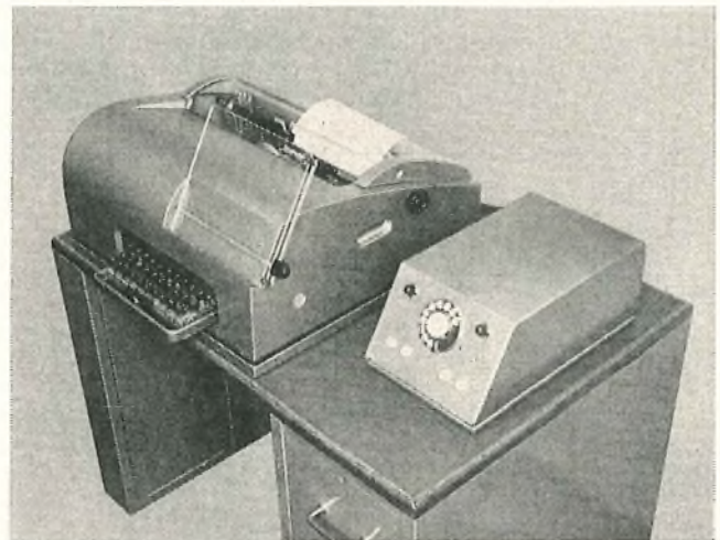
FIG. 3—SUBSCRIBER'S EQUIPMENT
