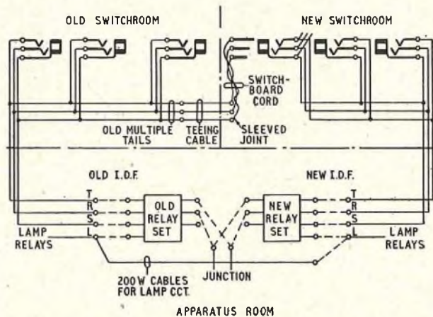
CHANGE-OVER ARRANGEMENTS AT HALIFAX AUTO-MANUAL SWITCHBOARD
