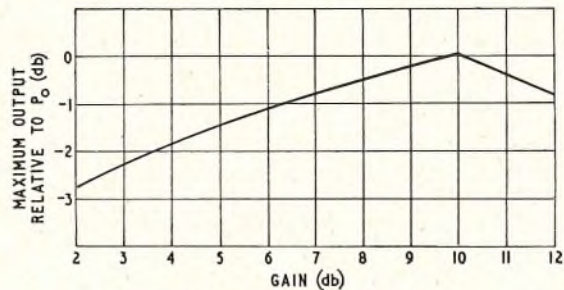
P_0 = Maximum power output at 10 db gain
