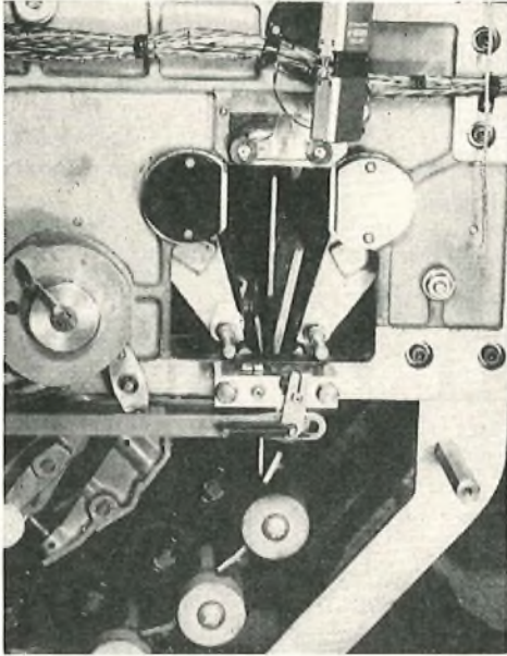
FIG. 8—DOUBLE WAITING-GATE
