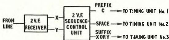
FIG. 2—MEASUREMENT OF 2 V.F. LINE SIGNALS
