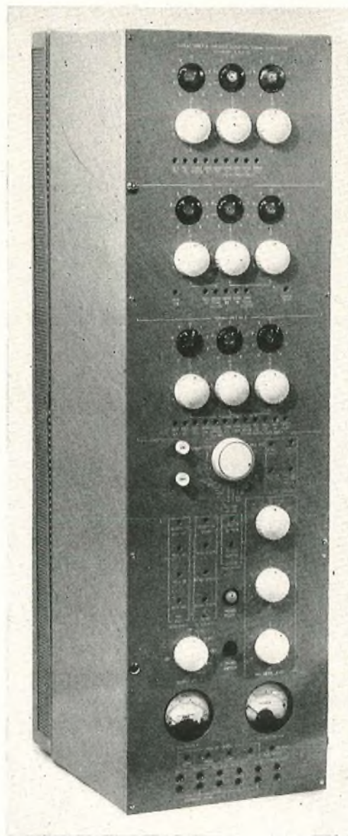
FIG. 1—SIGNAL GENERATOR AND MEASURING APPARATUS FOR INTERNATIONAL SIGNALLING SYSTEMS
