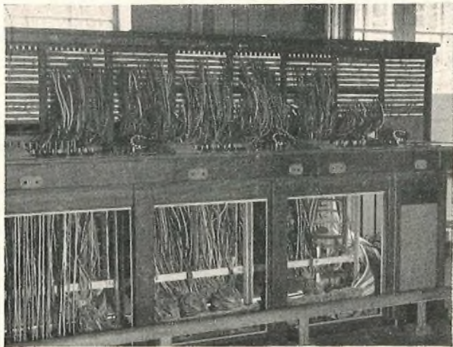
HALIFAX EXCHANGE, SHOWING TEEING OF WORKING CIRCUITS BETWEEN OLD AND NEW SWITCHBOARDS
