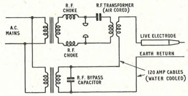
FIG. 25—ARGON-ARC WELDER
