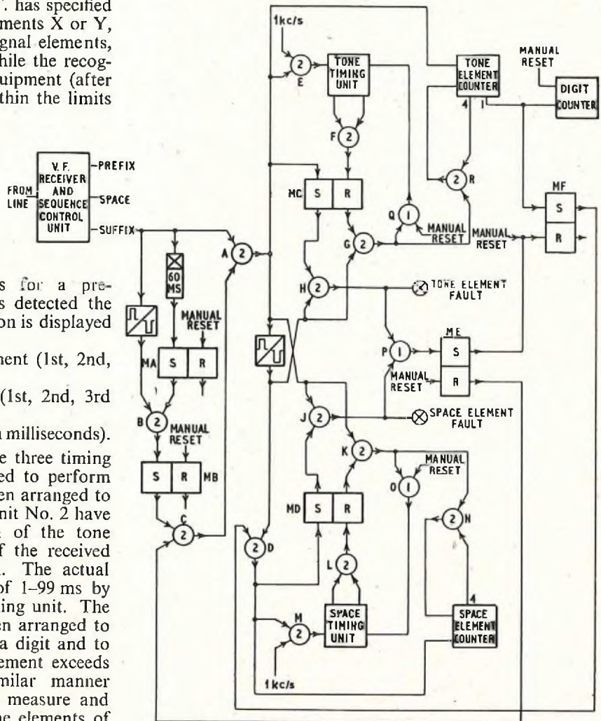
FIG. 5—LOGIC CIRCUIT FOR THE DIGIT CHECK
