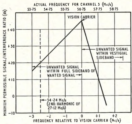
Based on C.C.I.R. (London) 1953 Report No. 34 FIG. 23—MINIMUM REQUIRED SIGNAL/INTERFERENCE RATIO FOR BRITISH TELEVISION SYSTEM
