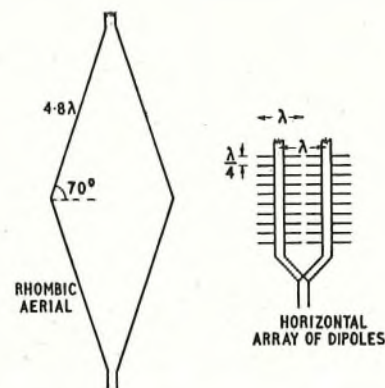
Height of each aerial above ground = 1.1\lambda FIG. 8—DETAILS OF TEST AERIALS
