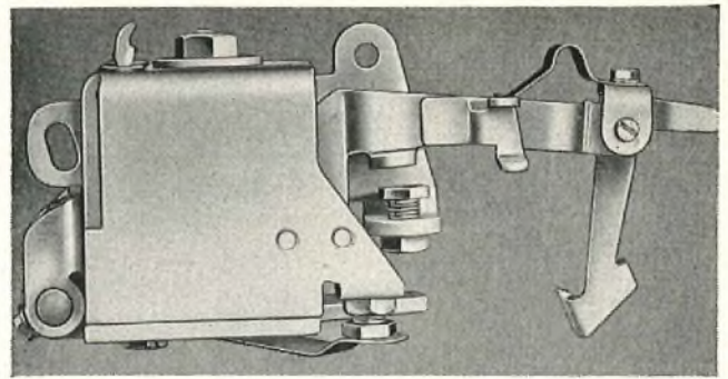
FIG. 4—VERTICAL-MAGNET ASSEMBLY
