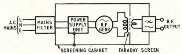
FIG. 24—MEDICAL DIATHERMY APPARATUS SHOWING INTERFERENCE-SUPPRESSION FEATURES
