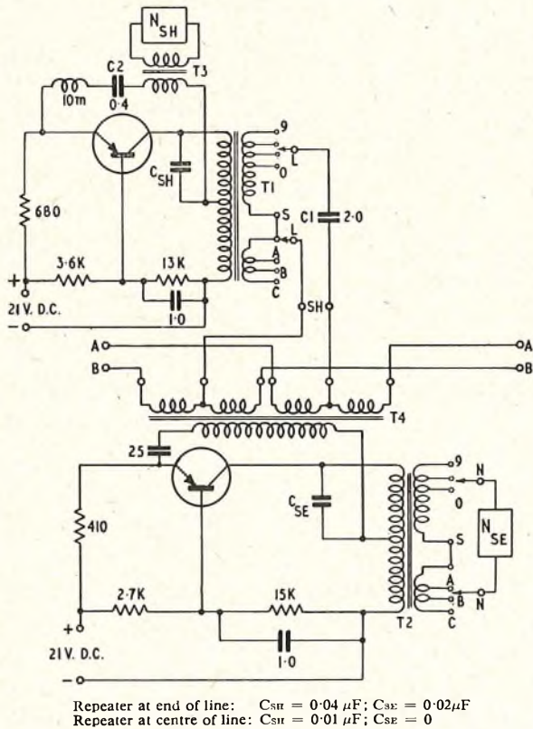
FIG. 8—CIRCUIT OF NEGATIVE-IMPEDANCE REPEATER
