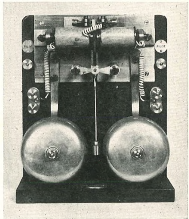
FIG. 2—ORIGINAL TYPE OF INTERNAL BELL
