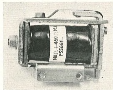
Armature is shown in the operated position FIG. 6—RELEASE MAGNET
