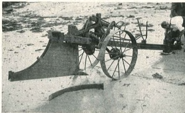
MODIFIED MOLEDRAINER USED FOR BURYING THE SHORE-END OF BOURNEMOUTH-JERSEY SUBMARINE CABLE
