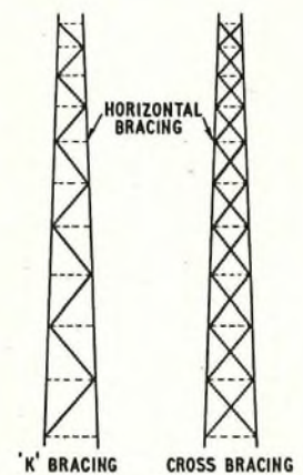
FIG. 11—BRACING ON MODEL LATTICE MAST
