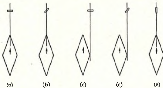
FIG. 14—POSITION OF KOOMANS ARRAY RELATIVE TO RHOMBIC AERIAL
