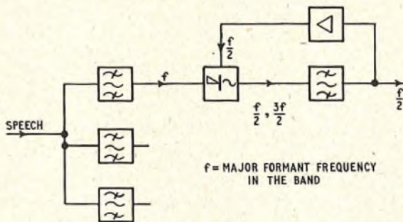
FIG. 5—VOBANC FREQUENCY-DIVIDING CIRCUIT
