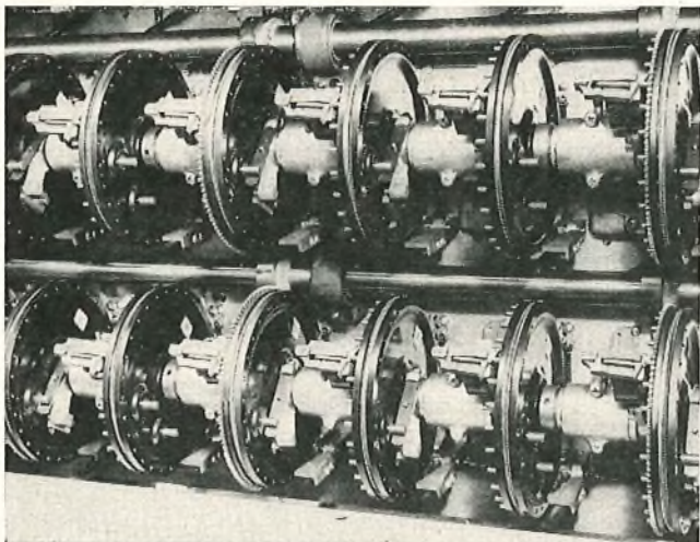
FIG. 10—PIN DISKS
