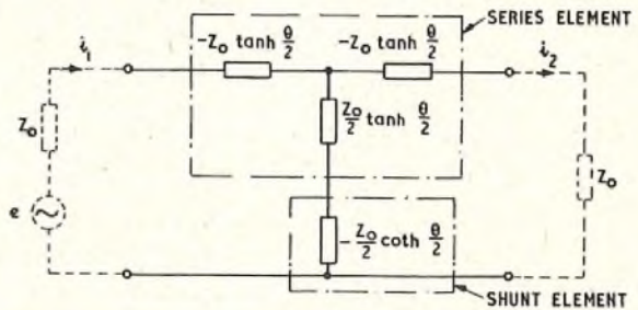
FIG. 7—EQUIVALENT CIRCUIT OF 4-TERMINAL NEGATIVE-IMPEDANCE REPEATER
