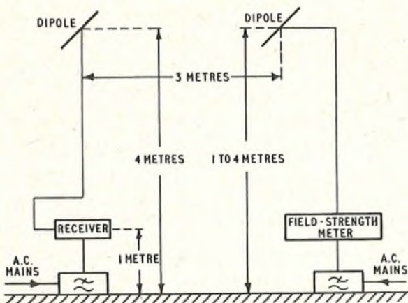
FIG. 27—MEASUREMENT OF OSCILLATOR RADIATION AT V.H.F.
