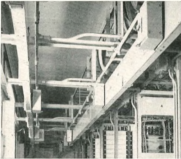
FIG. 4—POWER-DISTRIBUTION TRUNKING
