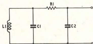
Network N_{SH} : L1 = 49.8 \text{ mH} ; R1 = 2,094 \text{ ohms} ; C1 = 0.0183 \mu F ; C2 = 0.0147 \mu F Network N_{SE} : L1 = 67.6 \text{ mH} ; R1 = 2,800 \text{ ohms} ; C1 = 0.0133 \mu F ; C2 = 0.0107 \mu F
