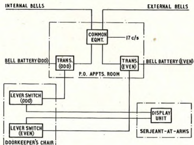
FIG. 3—BLOCK SCHEMATIC DIAGRAM OF THE NEW INSTALLATION
