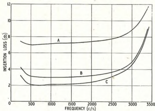
A—Insertion loss of line with no repeater in circuit B—Insertion loss of line plus repeater (1 db stability margin) C—Insertion loss of line plus repeater (no stability margin)
