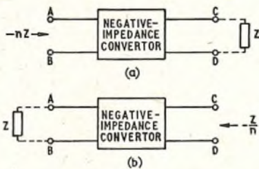
FIG. 1—COMBINATION OF A NEGATIVE-IMPEDANCE CONVERTOR AND A PASSIVE IMPEDANCE TO GIVE NEGATIVE IMPEDANCE
