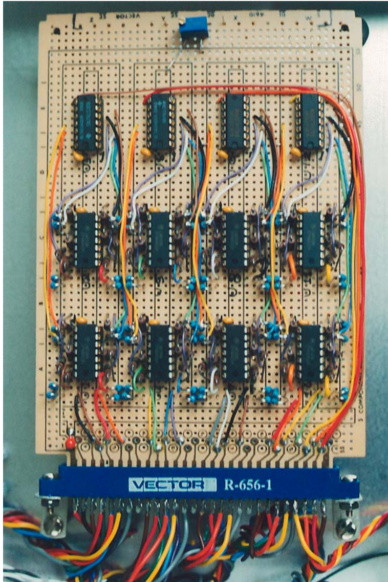
Figure A1-4. Detail of circuit board inside of Chassis 1047.
