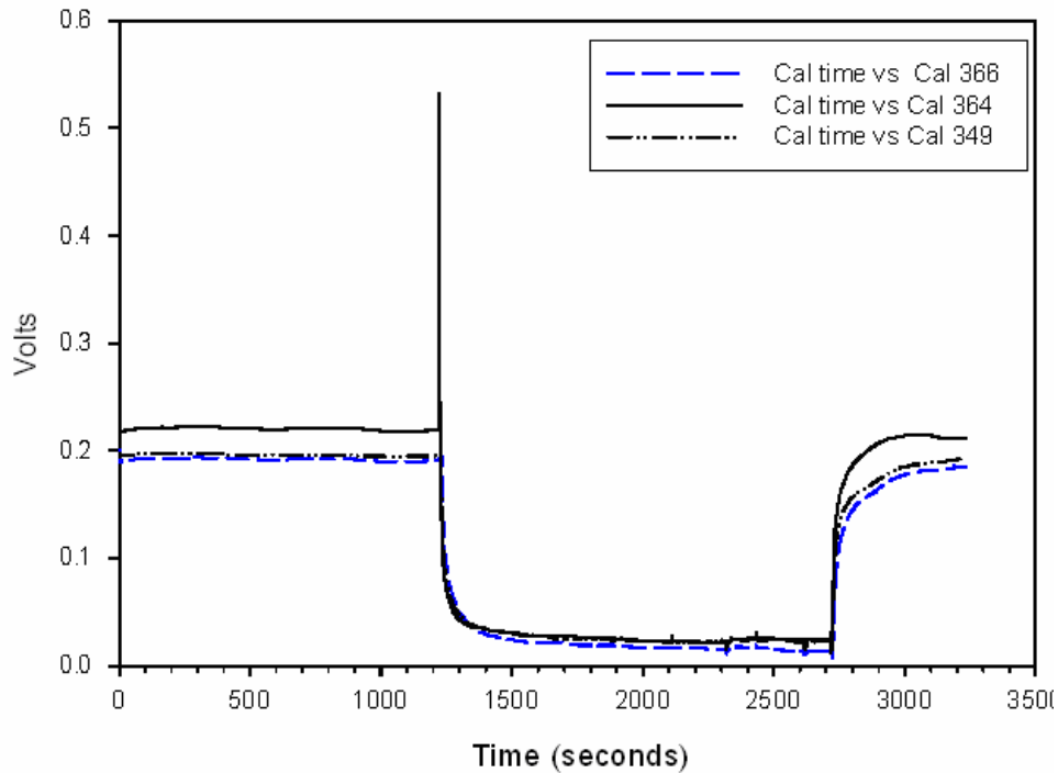
Figure 12. Pre-respiration run probe calibration trace showing probe stability at 100% and response time to 0% saturation. For 100% saturation filtered cave stream water was aerated with an airstone, while 0% saturated water was nitrogen bubbled for a minimum of 30 minutes to displace all oxygen. The voltage spike is associated with physically moving the probes into the 0% water.
