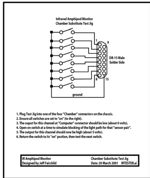
Figure A1-2. Infrared Amphipod Activity Monitor: A. Chassis 1047 connector pin assignments; B. Substitute test jig (Instructions: 1. Plug Test Jig into one of the four "Chamber" connectors on the chassis; 2. Ensure all switches are set to "on" [to the right]; 3. The output for this channel at "Computer" connector should be low [about 0 volts]; 4. Open "on" switch at a time to simulate blocking of the light path for that "sensor pair"; 5. The output for this channel should now be high [about 5 volts]; and 6. Return the switch to its "on" position, then test the next switch.).
