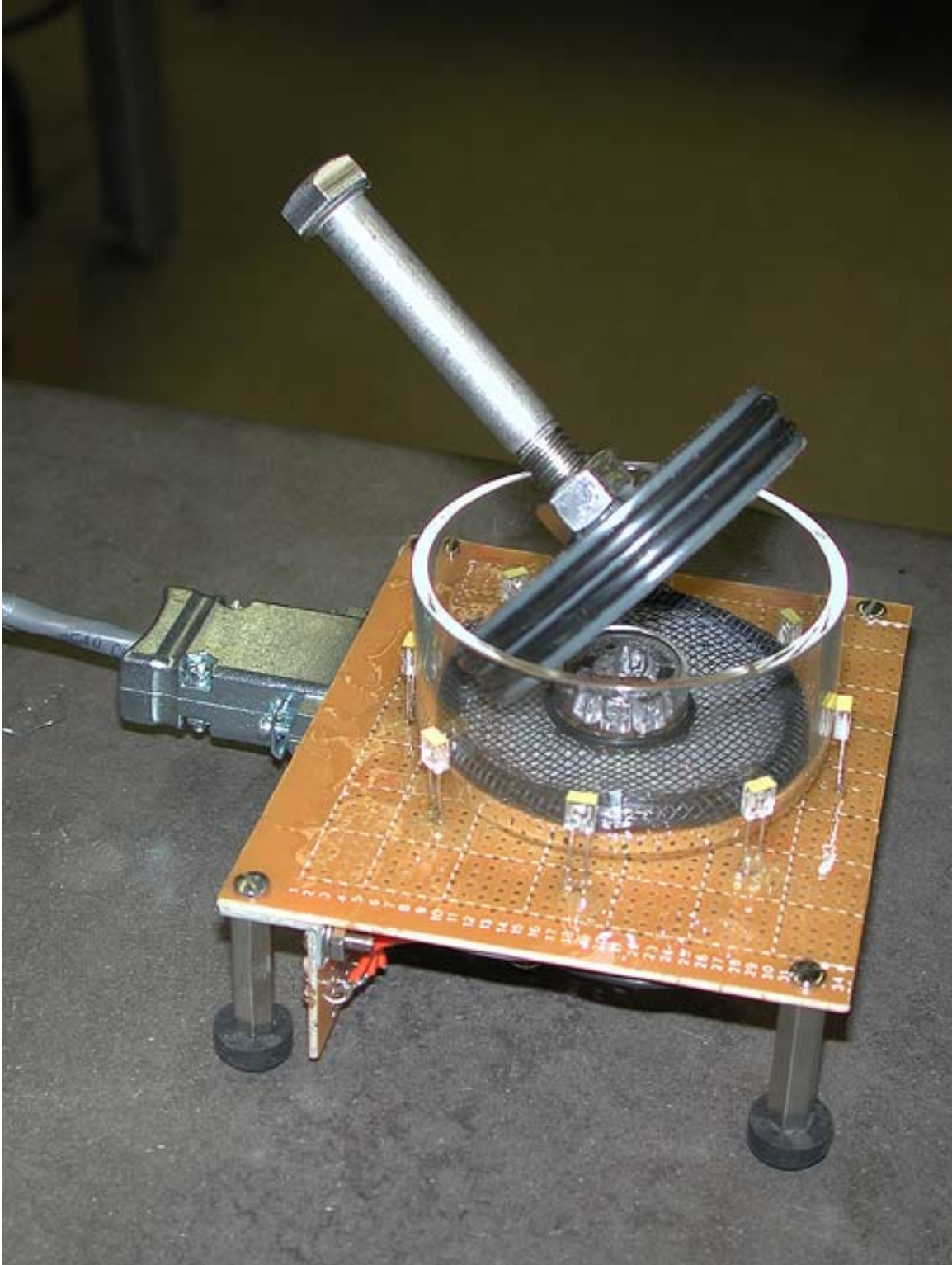
Figure A1-7. The activity chamber. Doughnut shaped screen elevates amphipods to a level where they will be detected by the infrared sensors. The stopper, with two o-rings, is sitting on top at an angle, and the cable to the left goes to the analog to digital board.
