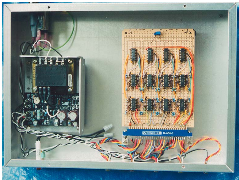
Figure A1-3. Chassis 1047. A. front view; B. back view; C. top view (cover removed to show power supply and circuit board).
