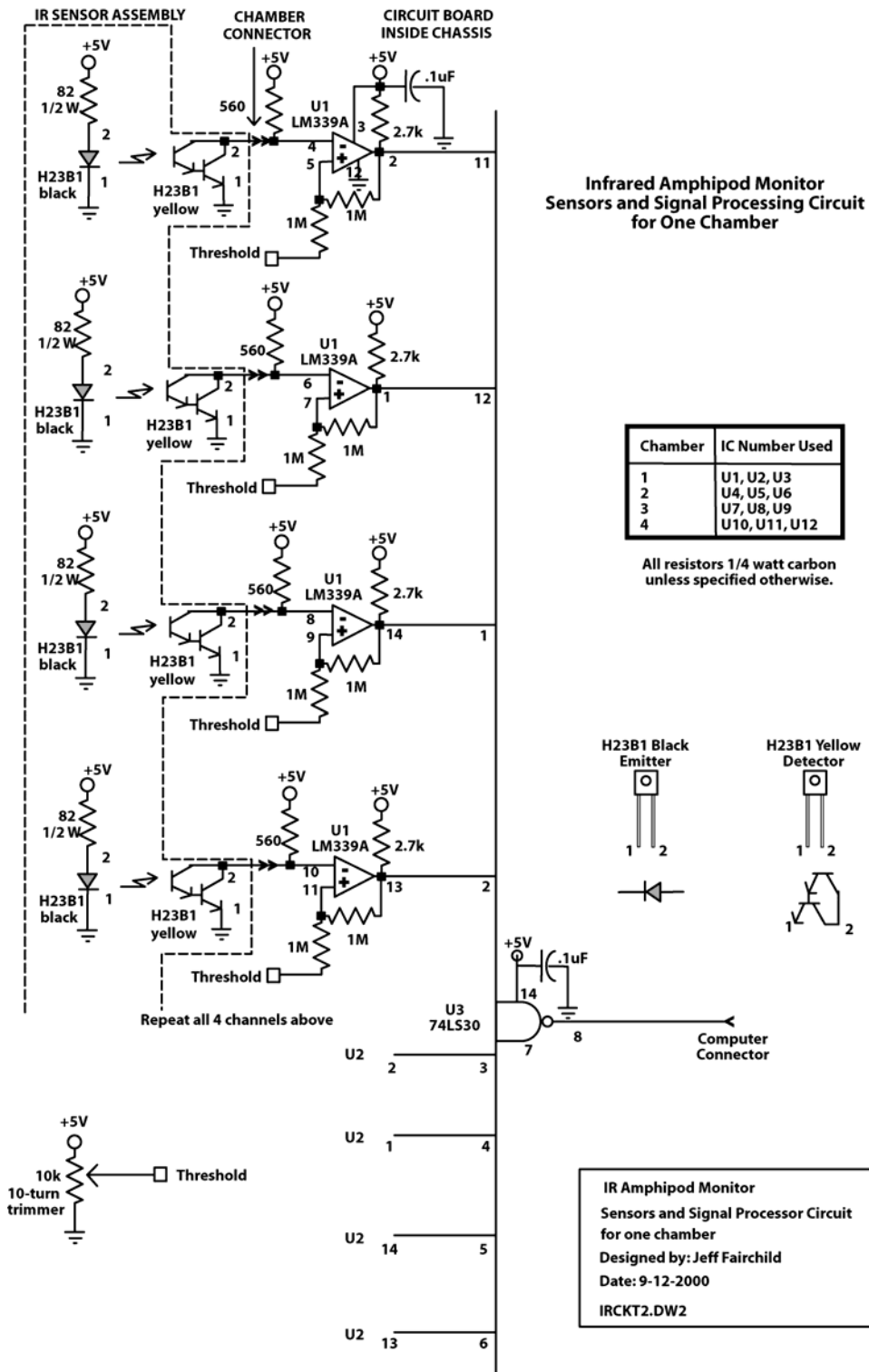
Figure A1-1. Infrared amphipod activity monitor: Sensors and signal processing circuit for one chamber.
