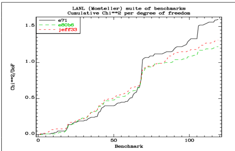
FIG. 3.3. Cumulative Chi-square per degree of freedom for the Mosteller suite of 119 benchmark cases assigning a minimum uncertainty of any benchmark to be 200 pcm.
