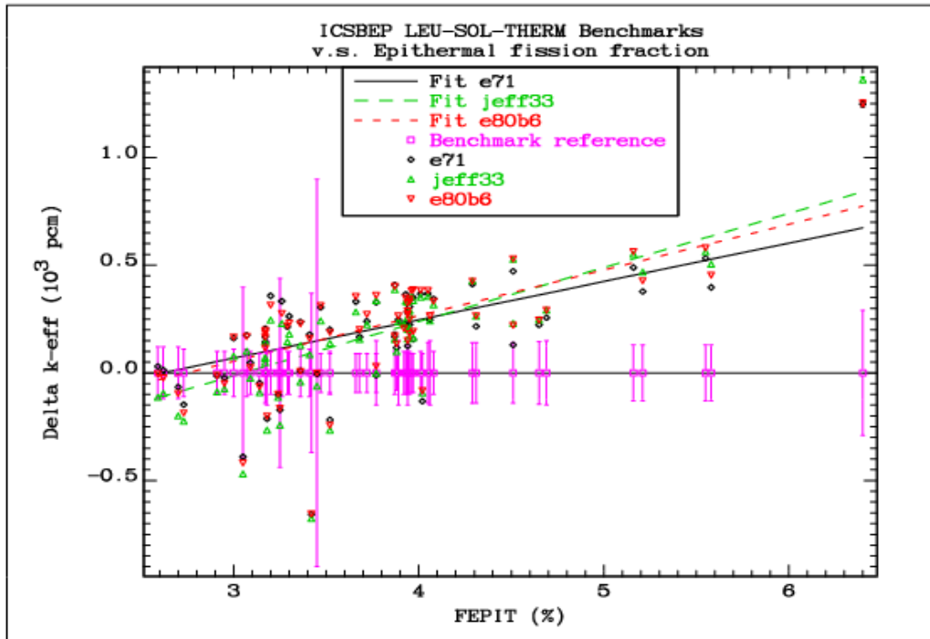
FIG. 6.3.1. Comparison of the differences between the calculated k_{eff} values and the reference benchmark values as a function of the epithermal fission fraction for the LEU-SOL-THERM benchmarks.
