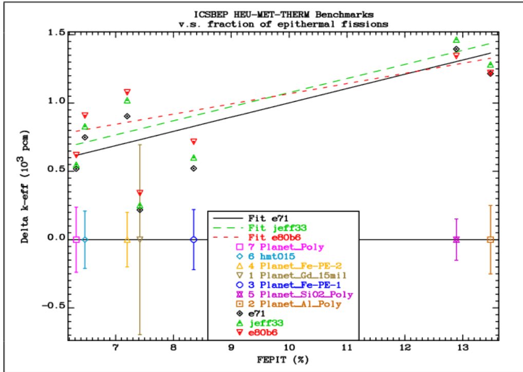
FIG. 4.8.2. Comparison of the differences between the calculated k_{eff} values and the reference benchmark values for HEU-MET-THERM benchmarks (excluding Valduc) as a function of the epithermal fission fraction. These are mainly cases containing polyethylene.
