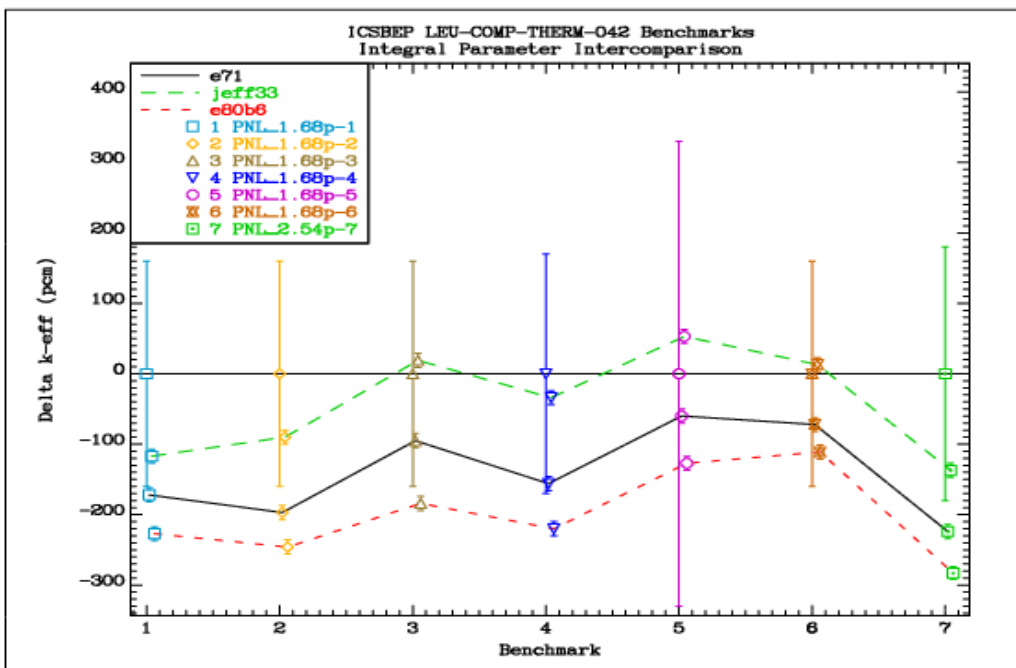
FIG. 6.1.7. Comparison of the differences between the calculated k_{\text{eff}} values and the reference benchmark values for the LEU-COMP-THERM-042 group of benchmarks.
