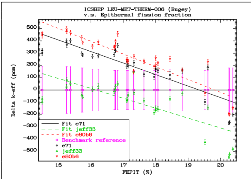
FIG. 6.2.6. Comparison of the differences between the calculated k_{eff} values and the reference benchmark values as a function of the epithermal fission fraction for the LEU-MET-THERM-006 benchmarks with a light water moderator.
