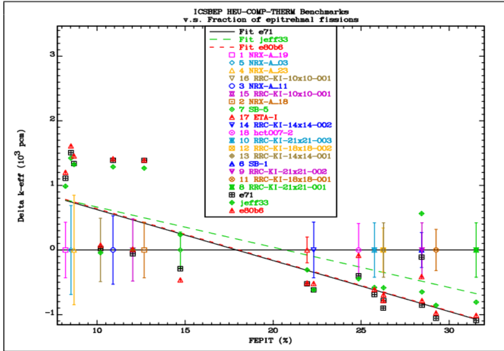
FIG. 4.4.2. Comparison of the differences between the calculated k_{eff} values and the reference benchmark values for the “HEU-COMP-THERM” benchmarks (excluding the group HEU-COMP-THERM-021) as a function of the epithermal fission fraction.
