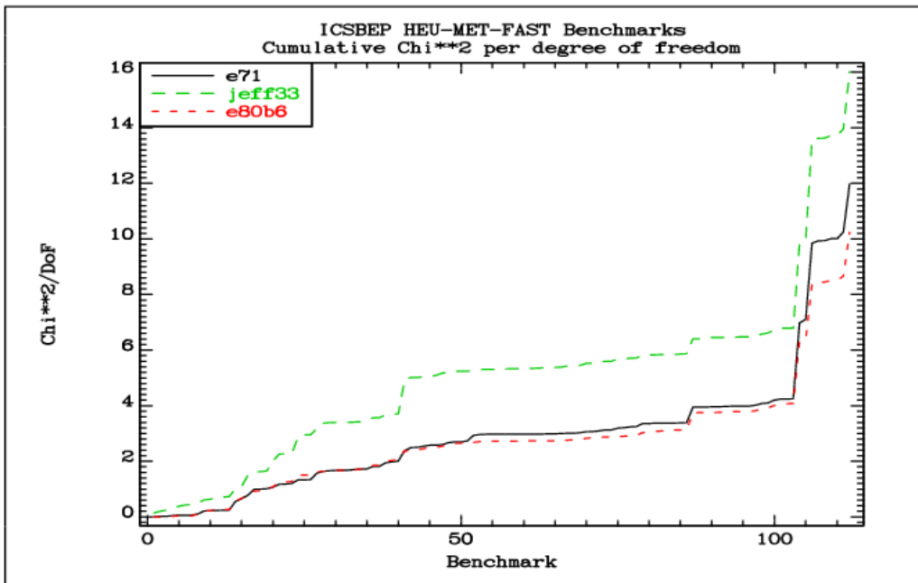
FIG. 4.5.2. Cumulative Chi-square per degree of freedom for the HEU-MET FAST group of benchmarks from the full IAEA suite of 1000 benchmark cases.
