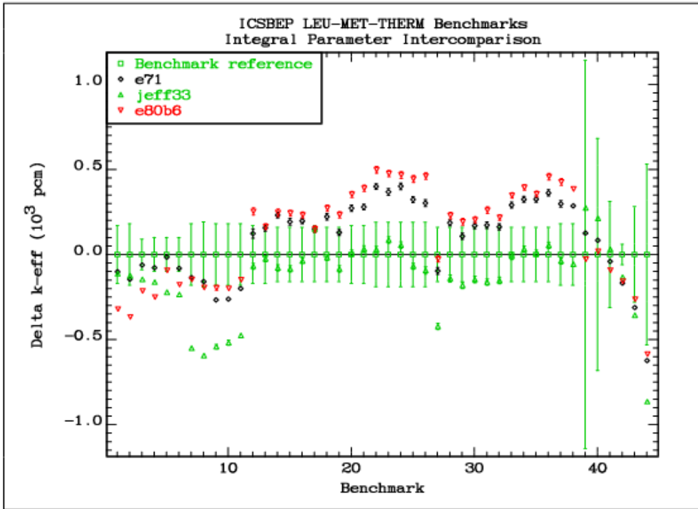
FIG. 6.2.3. Comparison of the differences between the calculated k_{eff} values and the reference benchmark values for the LEU-MET-THERM benchmarks with a light water moderator.
