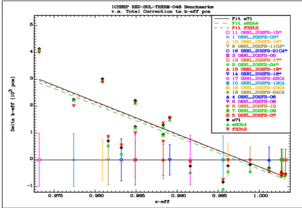
FIG. 4.9.6. Comparison of the differences between the calculated k_{\text{eff}} values and the reference benchmark values for the HEU-SOL-THERM-048 benchmark cases.
