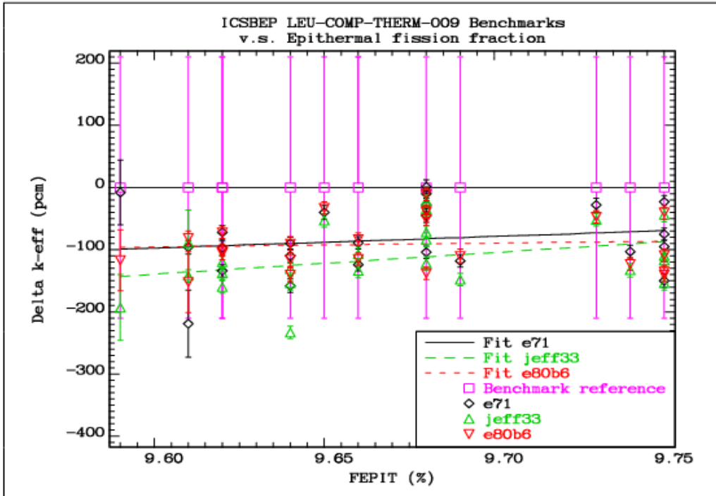
FIG. 6.1.4. Comparison of the differences between the calculated k_{\text{eff}} values and the reference benchmark values for the LEU-COMP-THERM-009 group of benchmarks as a function of the epithermal fission fraction.
