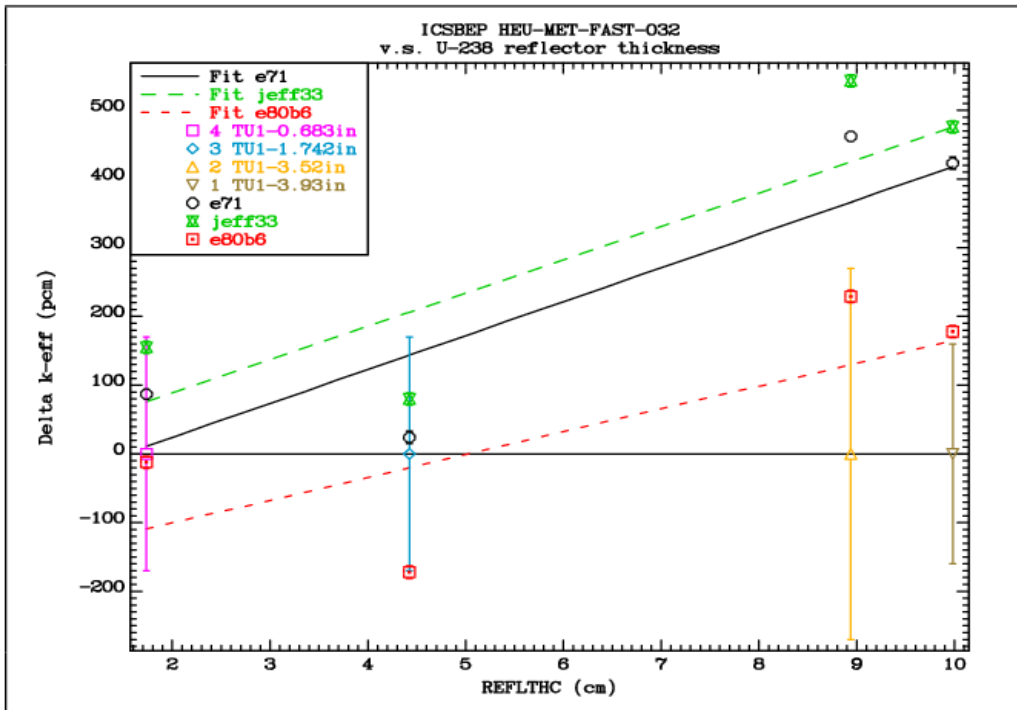
FIG. 4.5.6. Comparison of the differences between the calculated k_{eff} values and the reference benchmark values for the uranium-reflected assemblies of the HEU-MET-FAST-032 group of benchmarks as a function of reflector thickness.
