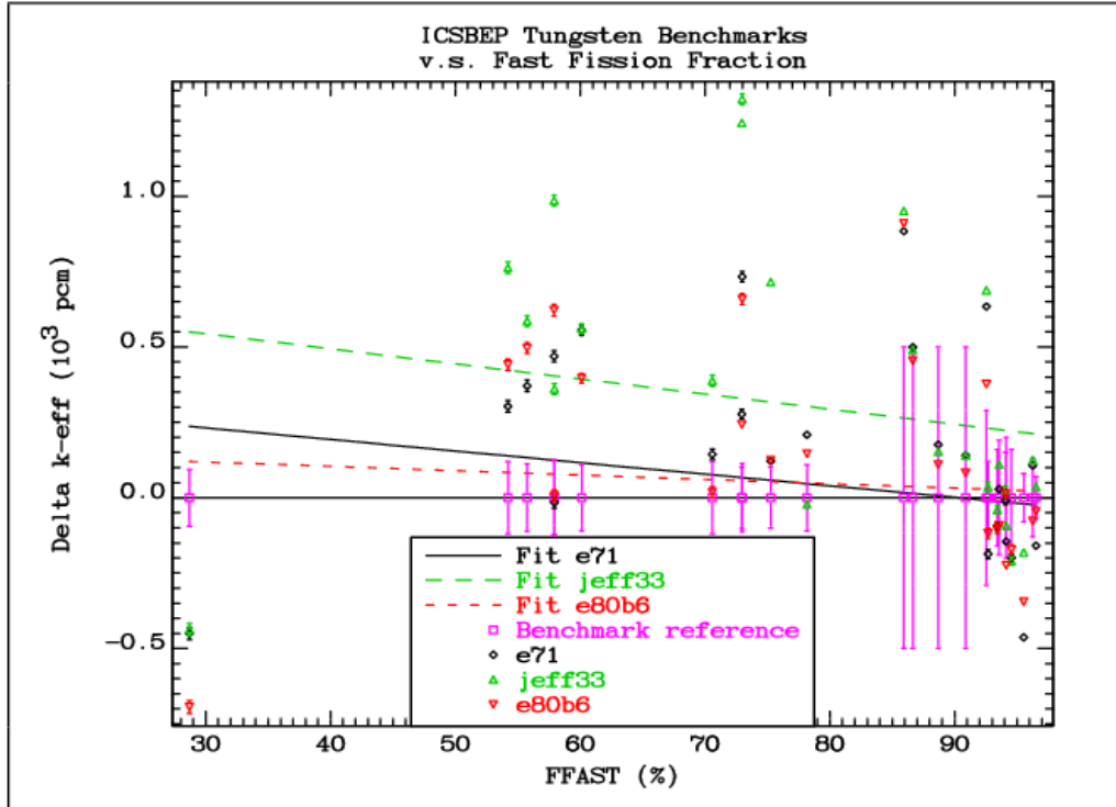
FIG. 7.3.1. Comparison of the differences between the calculated k_{eff} values and the reference benchmark values for all benchmarks containing tungsten. Benchmarks in which tungsten is the fuel dilutant have the softer spectrum.
