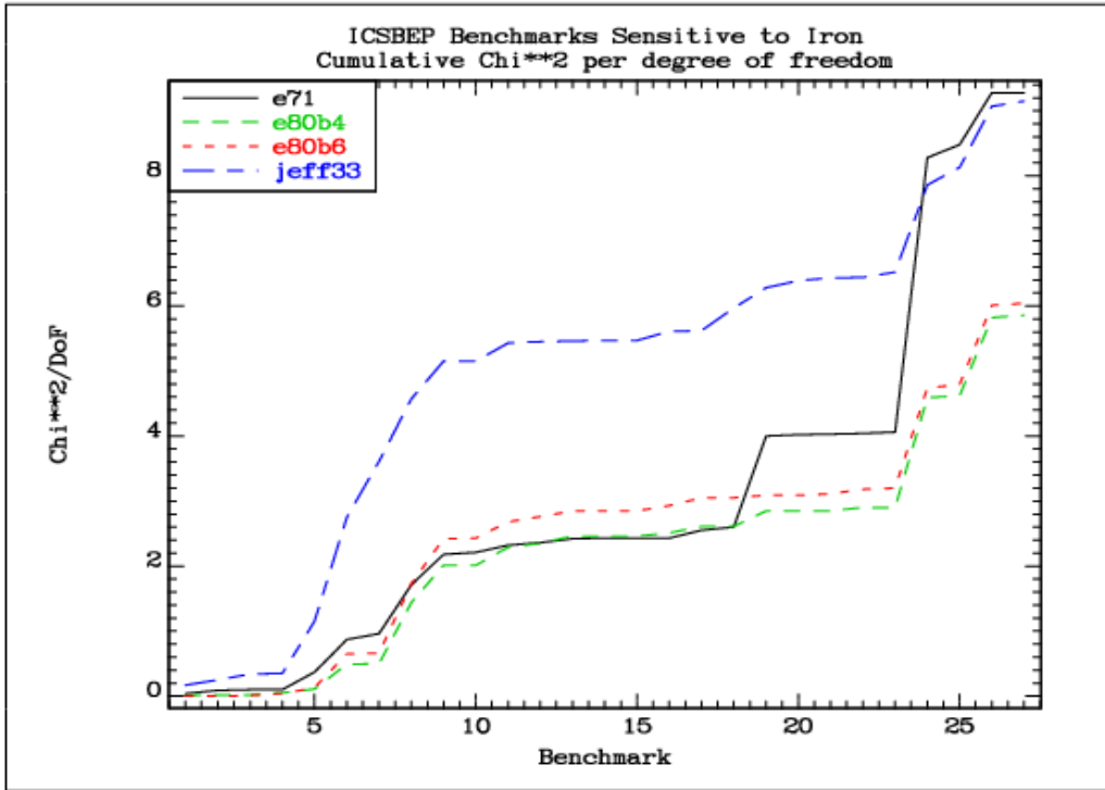
FIG. 7.1.1. Cumulative Chi-square per degree of freedom for the iron benchmarks from the full IAEA suite of benchmark cases.
