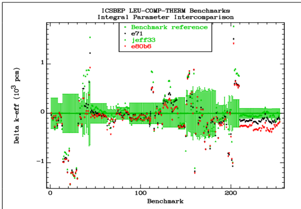
FIG. 6.1.1. Comparison of the differences between the calculated k_{eff} values and the reference benchmark values for the LEU-COMP-THERM group of benchmarks.
