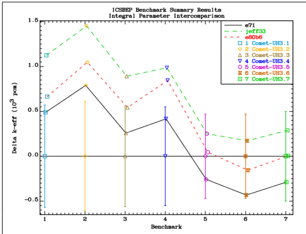
FIG. 4.2.1. Comparison of the differences between the calculated k_{eff} values and the reference benchmark values for the HEU-COMP-INTER-003 (Comet) assemblies with different reflectors.
