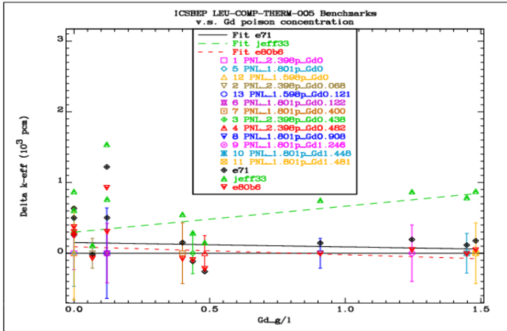
FIG. 6.1.2. Comparison of the differences between the calculated k_{\text{eff}} values and the reference benchmark values for the LEU-COMP-THERM-005 group of benchmarks as a function of Gd concentration.
