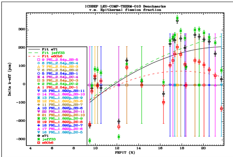
FIG. 6.1.5a. Comparison of the differences between the calculated k_{eff} values and the reference benchmark values for the LEU-COMP-THERM-010 group of benchmarks (excluding the lead-reflected cases) as a function of the epithermal fission fraction. The trendlines are parabolic fits.
