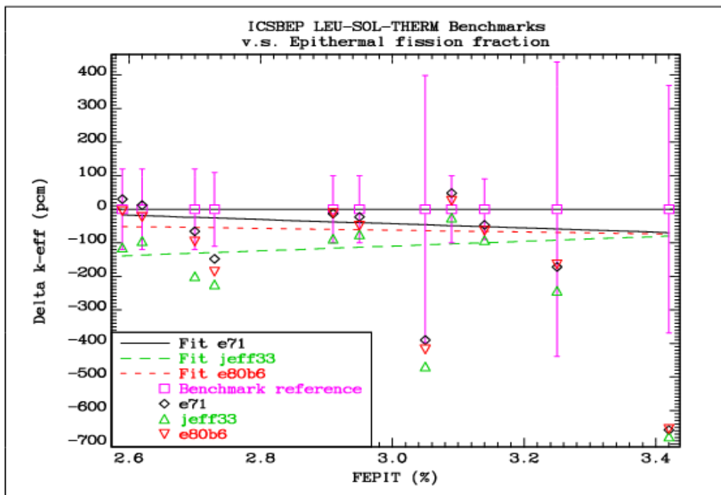
FIG. 6.3.3. Comparison of the differences between the calculated k_{eff} values and the reference benchmark values as a function of the epithermal fission fraction for the LEU-SOL-THERM benchmarks, which do not exhibit a gradient in reactivity.
