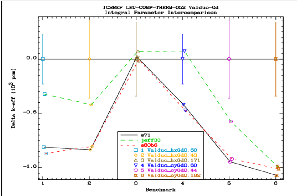
FIG. 6.1.3a. Comparison of the differences between the calculated k_{\text{eff}} values and the reference benchmark values for the Valduc LEU-COMP-THERM-052 group of benchmarks that contain gadolinium in the solution.
