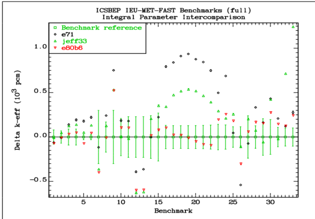
FIG. 5.3.1. Comparison of the differences between the calculated k_{eff} values and the reference benchmark values for the IEU-MET-FAST group of benchmarks.
