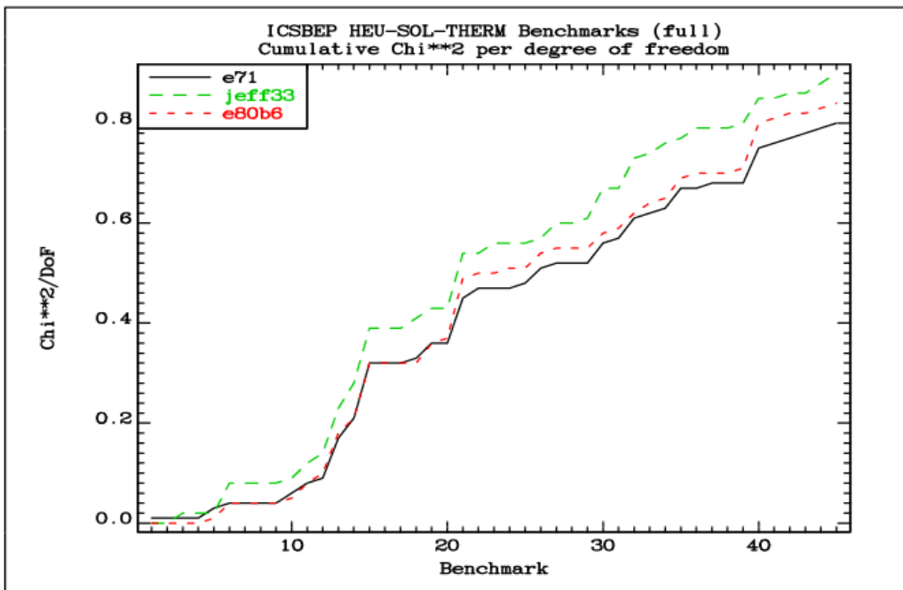
FIG. 4.9.2. Cumulative Chi-square per degree of freedom for the HEU-SOL-THERM benchmark cases.
