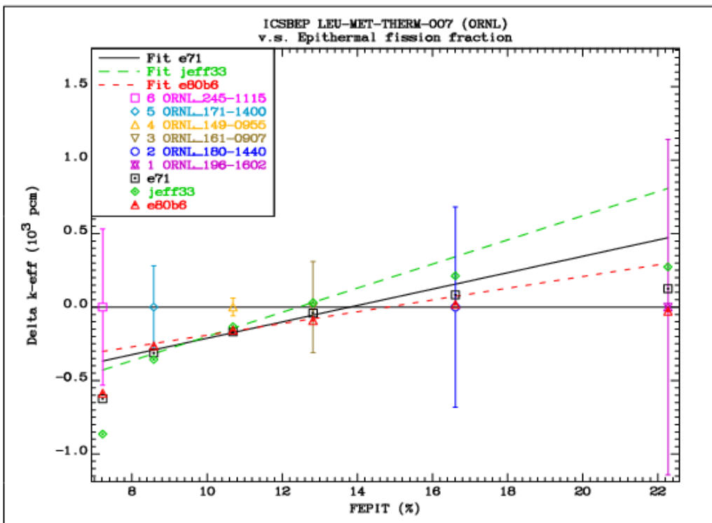
FIG. 6.2.4. Comparison of the differences between the calculated k_{eff} values and the reference benchmark values as a function of the epithermal fission fraction for the LEU-MET-THERM-007 benchmarks with a light water moderator.
