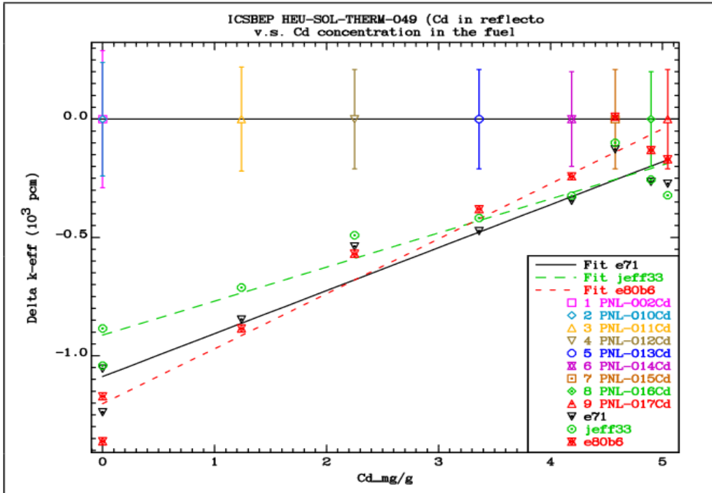
FIG. 4.9.8. Comparison of the differences between the calculated k_{eff} values and the reference benchmark values for the HEU-SOL-THERM-049 benchmark cases with cadmium in the reflector solution.
