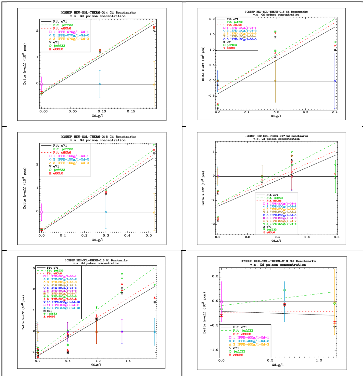
FIG. 4.9.9. Comparison of the differences between the calculated k_{eff} values and the reference benchmark values for the IPPE highly-enriched solution benchmarks as a function of the gadolinium concentration.
