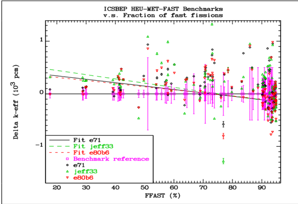
FIG. 4.5.1. Comparison of the differences between the calculated k_{eff} values and the reference benchmark values for the HEU-MET-FAST group of benchmarks from the full IAEA suite of 1000 benchmark cases as a function of the fast fission fraction.
