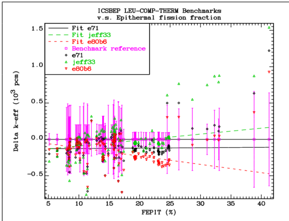
FIG. 6.1.9. Comparison of the differences between the calculated k_{eff} values and the reference benchmark values for the selected groups of benchmarks as a function of the epithermal fission fraction.
