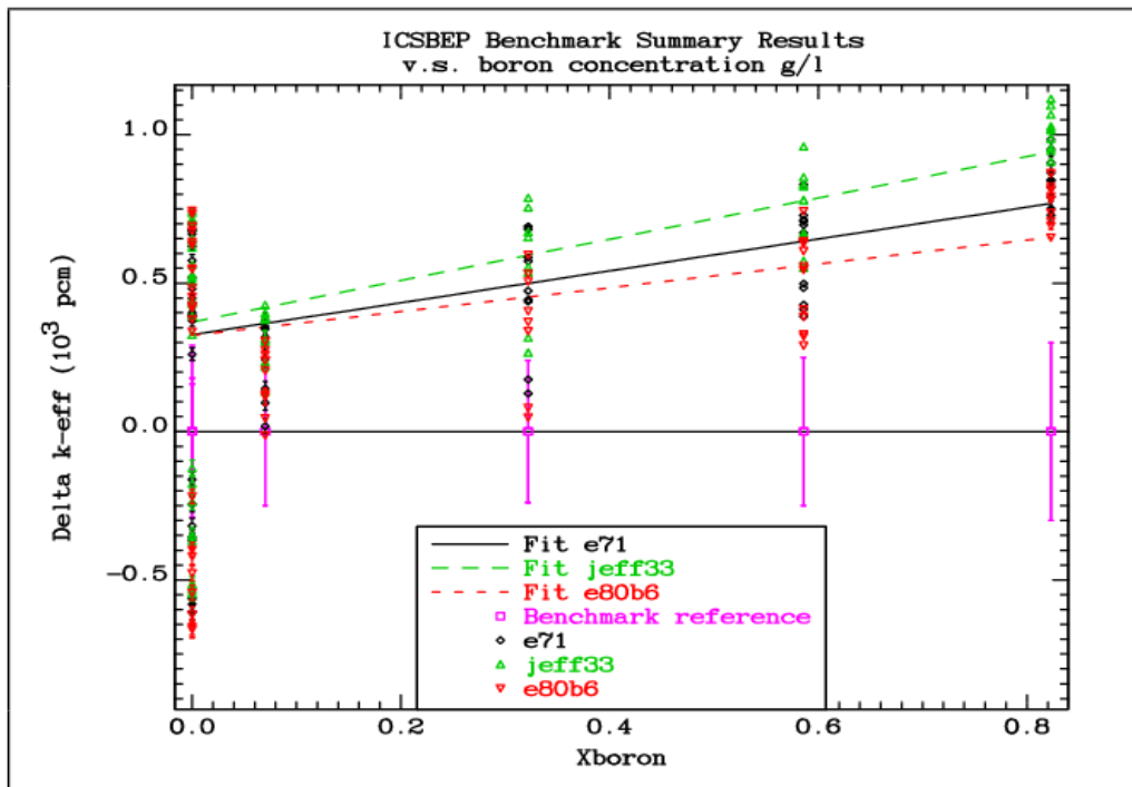
FIG. 4.4.1. Comparison of the differences between the calculated k_{eff} values and the reference benchmark values for the "HEU-COMP-THERM-021" benchmarks as a function of boron concentration [g/l].
