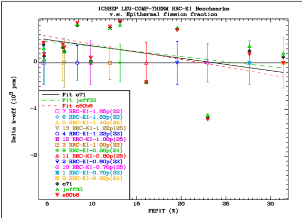
FIG. 6.1.6. Comparison of the differences between the calculated k_{\text{eff}} values and the reference benchmark values for the LEU-COMP-THERM-022, 24, 25 group of benchmarks as a function of the epithermal fission fraction.
