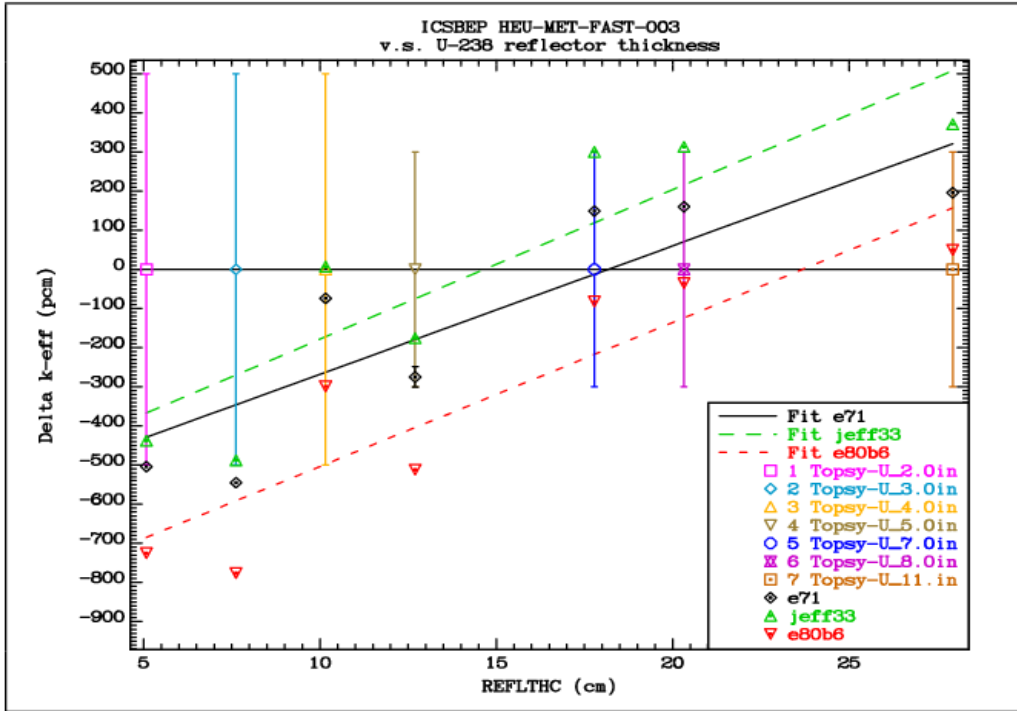
FIG. 4.5.5. Comparison of the differences between the calculated k_{eff} values and the reference benchmark values for the uranium-reflected assemblies of the HEU-MET-FAST-003 group of benchmarks as a function of reflector thickness.
