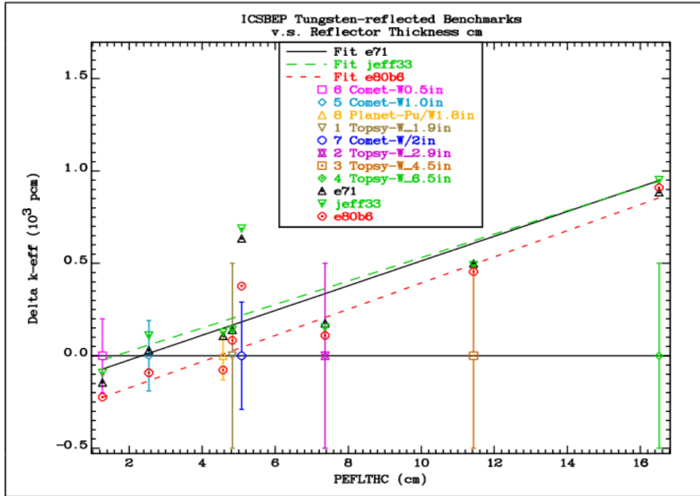
FIG. 7.3.2. Comparison of the differences between the calculated k_{eff} values and the reference benchmark values for the benchmarks with a tungsten reflector as a function of reflector thickness.
