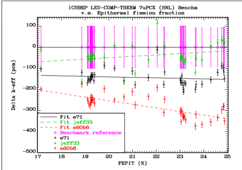
FIG. 6.1.8. Comparison of the differences between the calculated k_{eff} values and the reference benchmark values for the LEU-COMP-THERM-078, 80 and 96 group of benchmarks as a function of the epithermal fission fraction.
