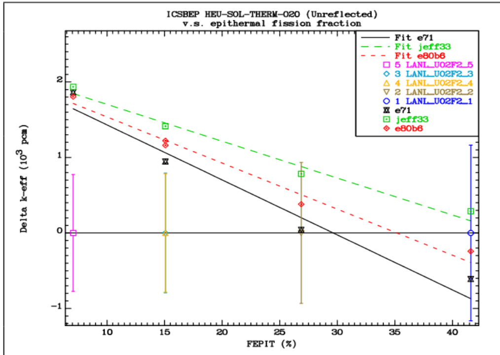
FIG.4.9.5. Comparison of the differences between the calculated k_{eff} values and the reference benchmark values for the HEU-SOL-THERM-020 benchmark cases as a function of the epithermal fission fraction.
