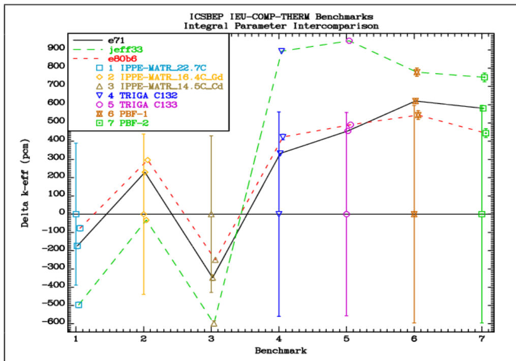
FIG. 5.2.1. Comparison of the differences between the calculated k_{eff} values and the reference benchmark values for the IEU-COMP-THERM group of benchmarks.
