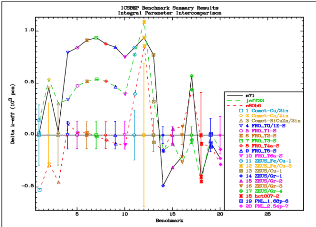
FIG. 7.2.1. Comparison of the differences between the calculated k_{eff} values and the reference benchmark values for the copper-reflected assemblies.
