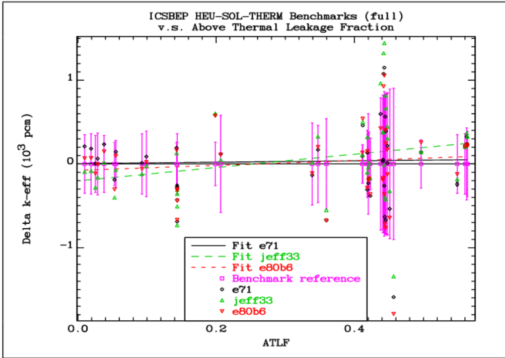
FIG. 4.9.1. Comparison of the differences between the calculated k_{\text{eff}} values and the reference benchmark values for the HEU-SOL-THERM benchmark cases.
