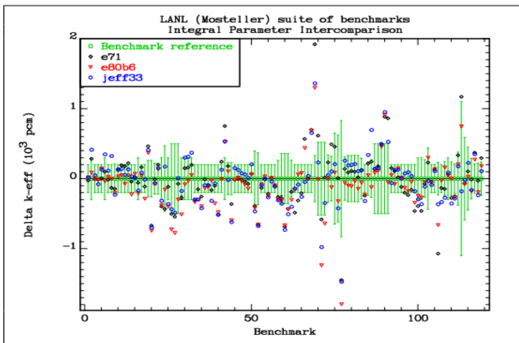
FIG. 3.1. Comparison of the differences between the calculated k_{\text{eff}} values and the reference benchmark values for the Mosteller suite of 119 benchmark cases.
