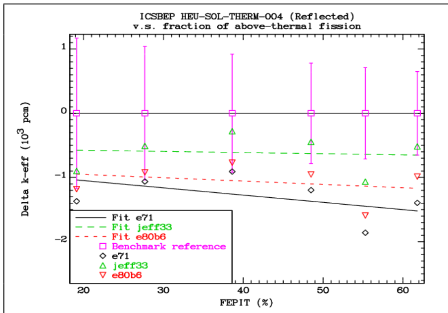
FIG. 4.9.4. Comparison of the differences between the calculated k_{eff} values and the reference benchmark values for the HEU-SOL-THERM-004 benchmark cases as a function of the epithermal fission fraction.
