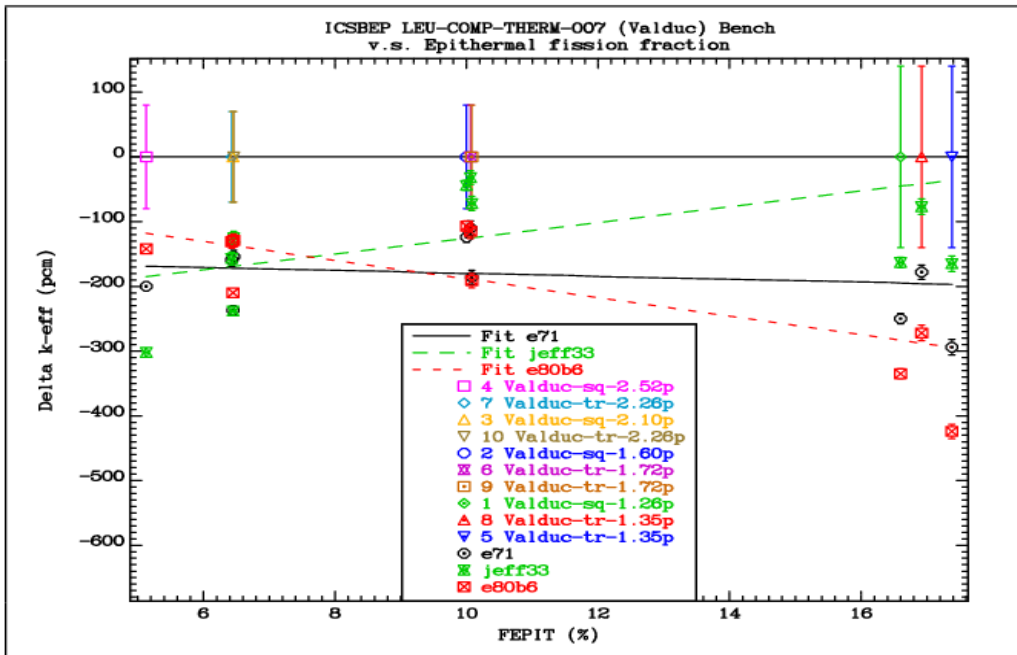
FIG. 6.1.3. Comparison of the differences between the calculated k_{eff} values and the reference benchmark values for the Valduc LEU-COMP-THERM-007 group of benchmarks as a function of the epithermal fission fraction.
