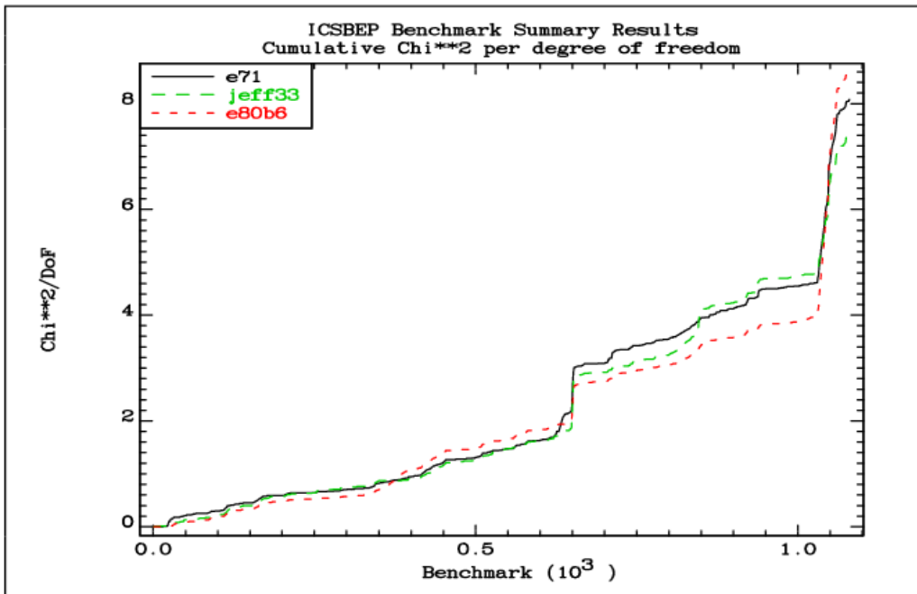
FIG. 3.5. Cumulative Chi-square per degree of freedom for the full IAEA suite of 1000 benchmark cases.
