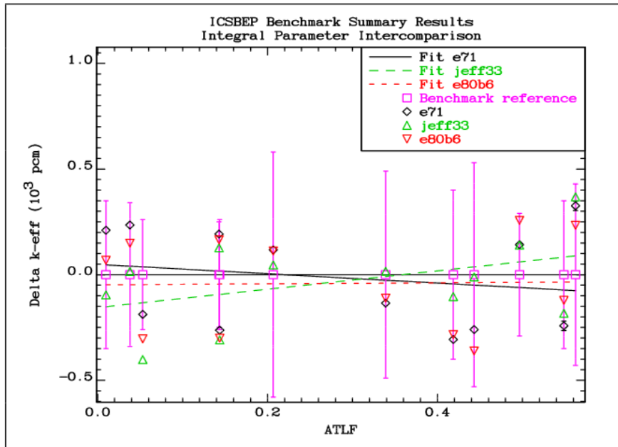
FIG. 4.9.3. Comparison of the differences between the calculated k_{eff} values and the reference benchmark values for the short list of representative HEU-SOL-THERM benchmark cases.
