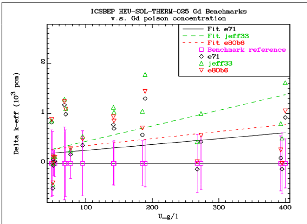
FIG. 4.9.11. Comparison of the differences between the calculated k_{\text{eff}} values and the reference benchmark values for the HEU-SOL-THERM-025 benchmarks as a function of uranium concentration.
