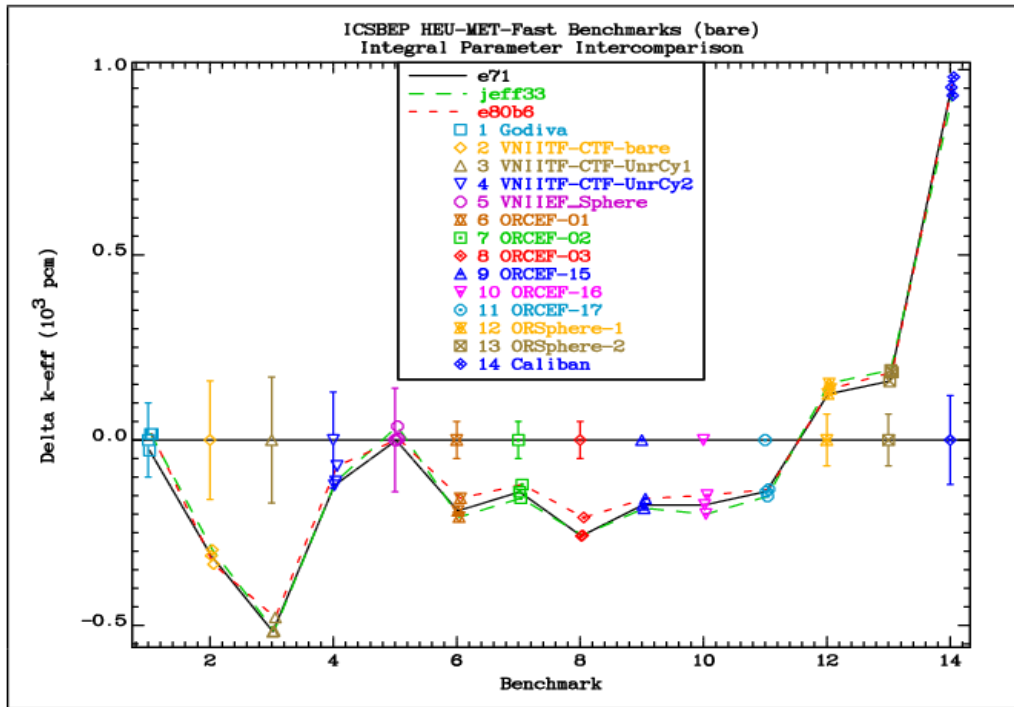
FIG. 4.5.3. Comparison of the differences between the calculated k_{eff} values and the reference benchmark values for the bare assemblies of the HEU-MET-FAST group of benchmarks.
