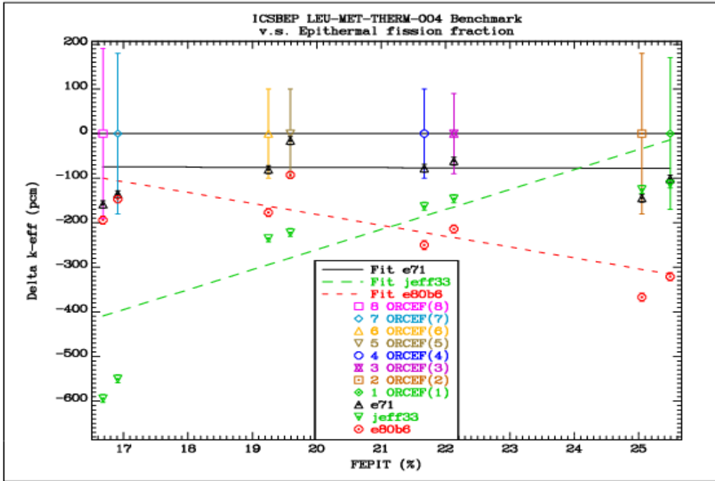
FIG. 6.2.5. Comparison of the differences between the calculated k_{eff} values and the reference benchmark values as a function of the epithermal fission fraction for the LEU-MET-THERM-004 benchmarks with a light water moderator.
