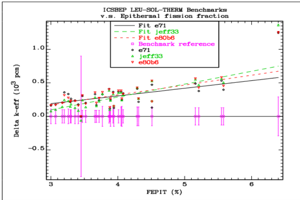
FIG. 6.3.2. Comparison of the differences between the calculated k_{eff} values and the reference benchmark values as a function of the epithermal fission fraction for the LEU-SOL-THERM benchmarks, which exhibit a gradient in reactivity.
