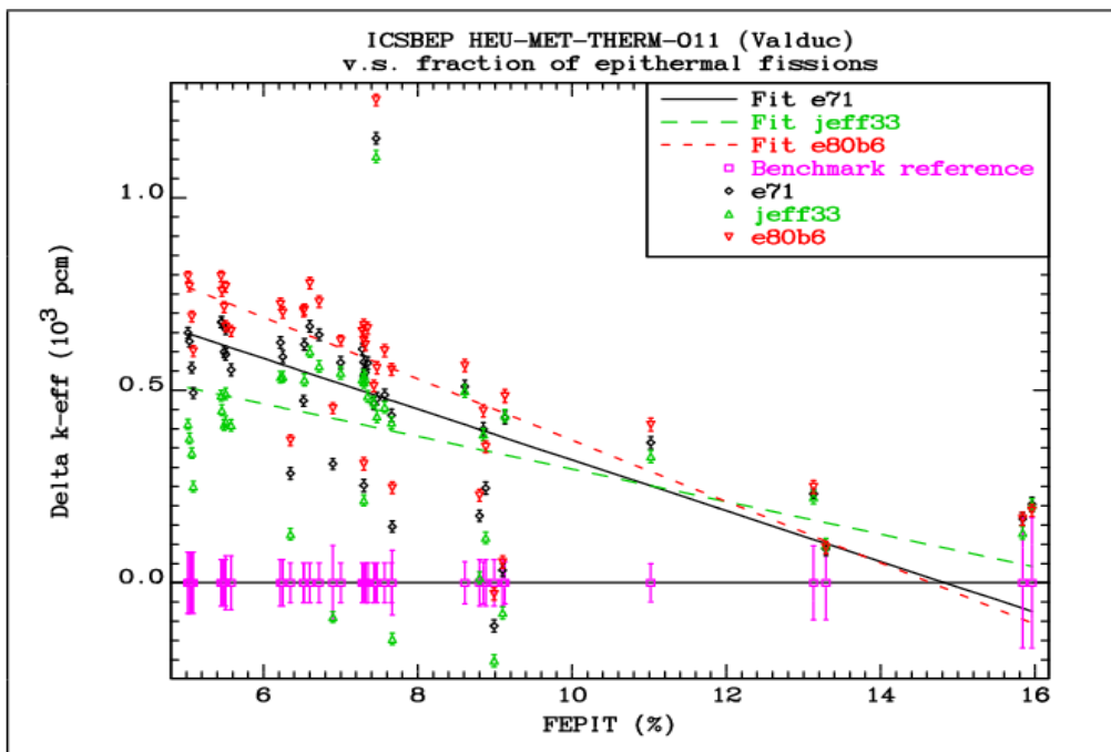
FIG. 4.8.1. Comparison of the differences between the calculated k_{\text{eff}} values and the reference benchmark values for HEU-MET-THERM-011 (Valduc) benchmarks as a function of the epithermal fission fraction.
