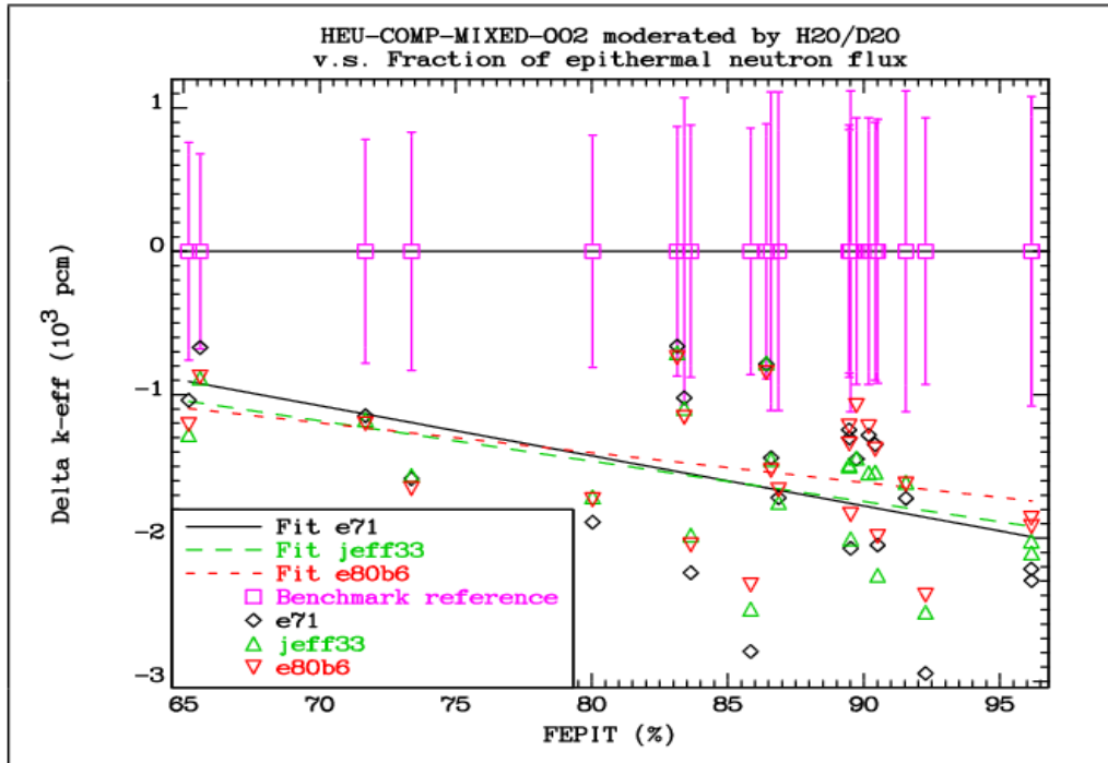
FIG. 4.3.1. Comparison of the differences between the calculated k_{eff} values and the reference benchmark values as a function of the epithermal fission fraction (FEPIT) for the HEU-COMP-MIXED-002 benchmarks.
