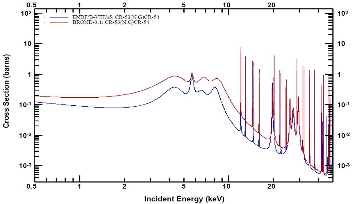
FIG. 4.2.3. Comparison of the ^{53}\text{Cr}(n,g) cross sections from the ENDF/B-VIII. and BROND-3.1 libraries. The Cross sections in ENDF/B-VII.1 are identical to ENDF/B-VIII.
