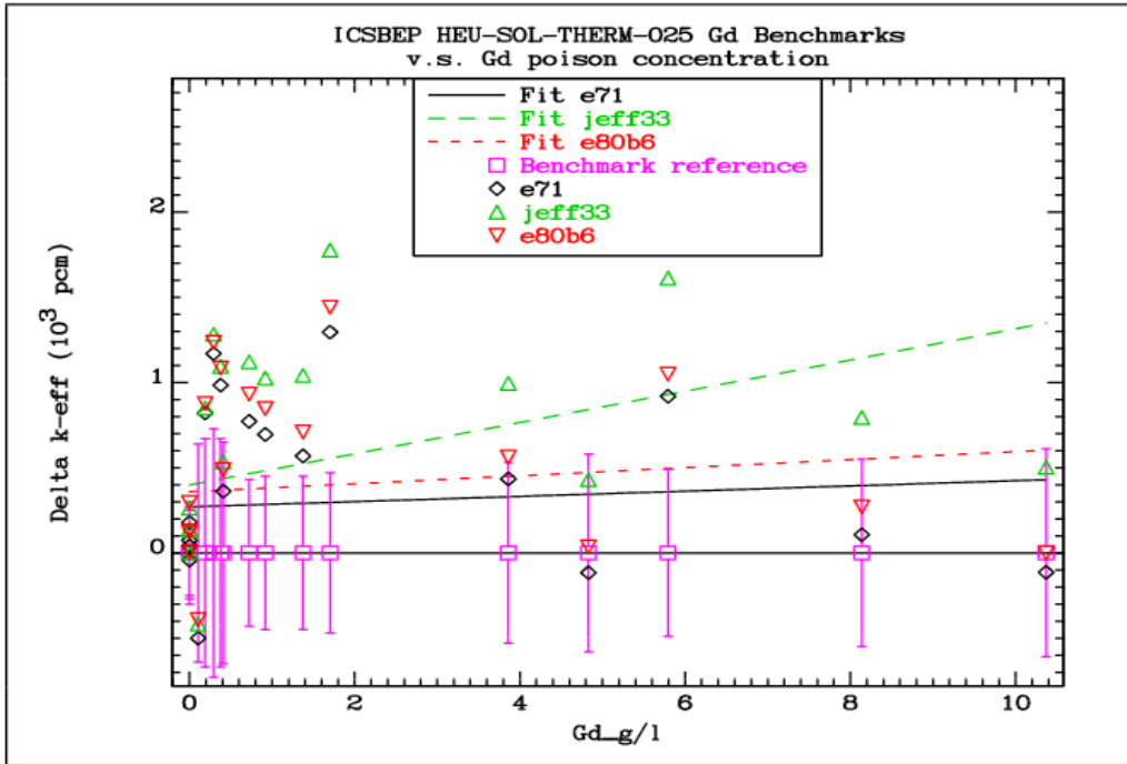
FIG. 4.9.10. Comparison of the differences between the calculated k_{\text{eff}} values and the reference benchmark values for the HEU-SOL-THERM-025 benchmarks as a function of gadolinium concentration.
