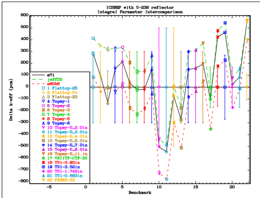
FIG. 4.5.4. Comparison of the differences between the calculated k_{eff} values and the reference benchmark values for the uranium-reflected assemblies of the HEU-MET-FAST group of benchmarks with a uranium reflector.
