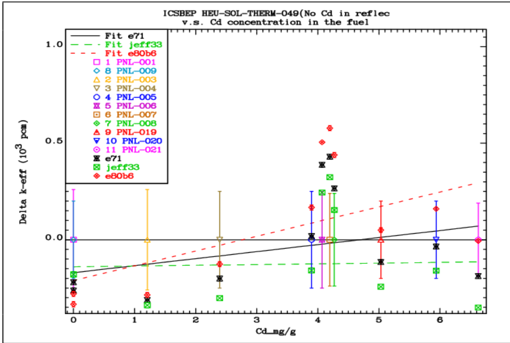
FIG. 4.9.7. Comparison of the differences between the calculated k_{eff} values and the reference benchmark values for the HEU-SOL-THERM-049 benchmark cases without cadmium in the reflector solution.
