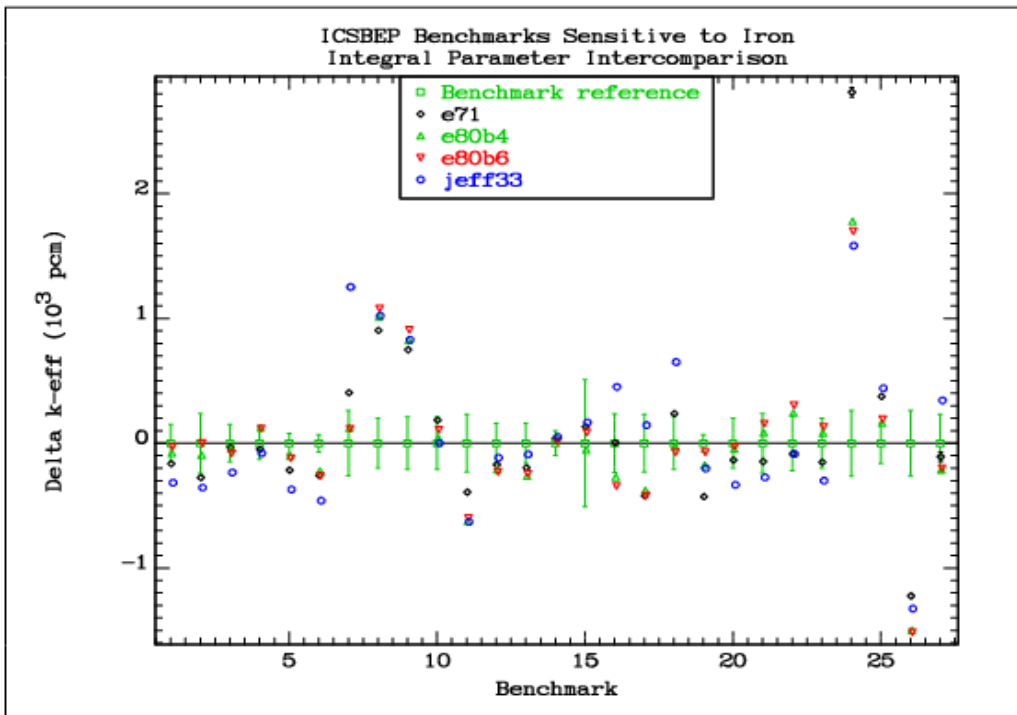
FIG. 7.1.2. Comparison of the differences between the calculated k_{eff} values and the reference benchmark values for the iron- or stainless steel-reflected assemblies of the HEU-MET-FAST group of benchmarks.
