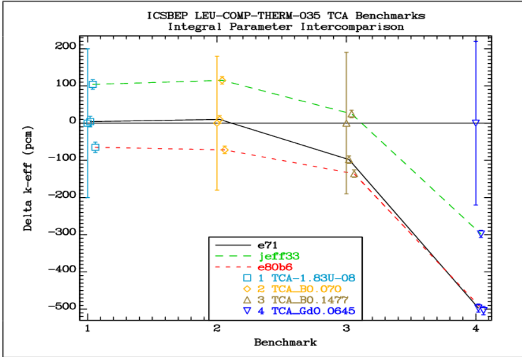
FIG. 6.1.2b. Comparison of the differences between the calculated k_{eff} values and the reference benchmark values for the LEU-COMP-THERM-035 group of benchmarks; the first case is the reference LEU-COMP-THERM-006 Case 8 without any absorber in the solution.
