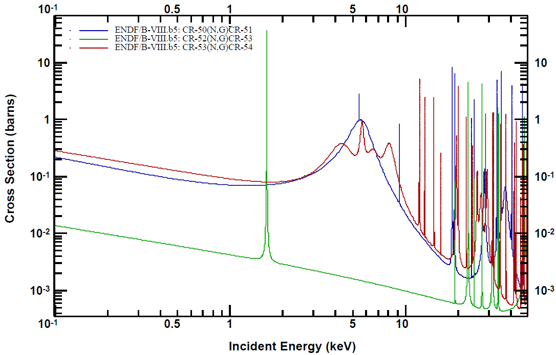
FIG. 4.2.4. Comparison of the capture cross sections of the minor Cr isotopes from the ENDF/B-VIII library.
