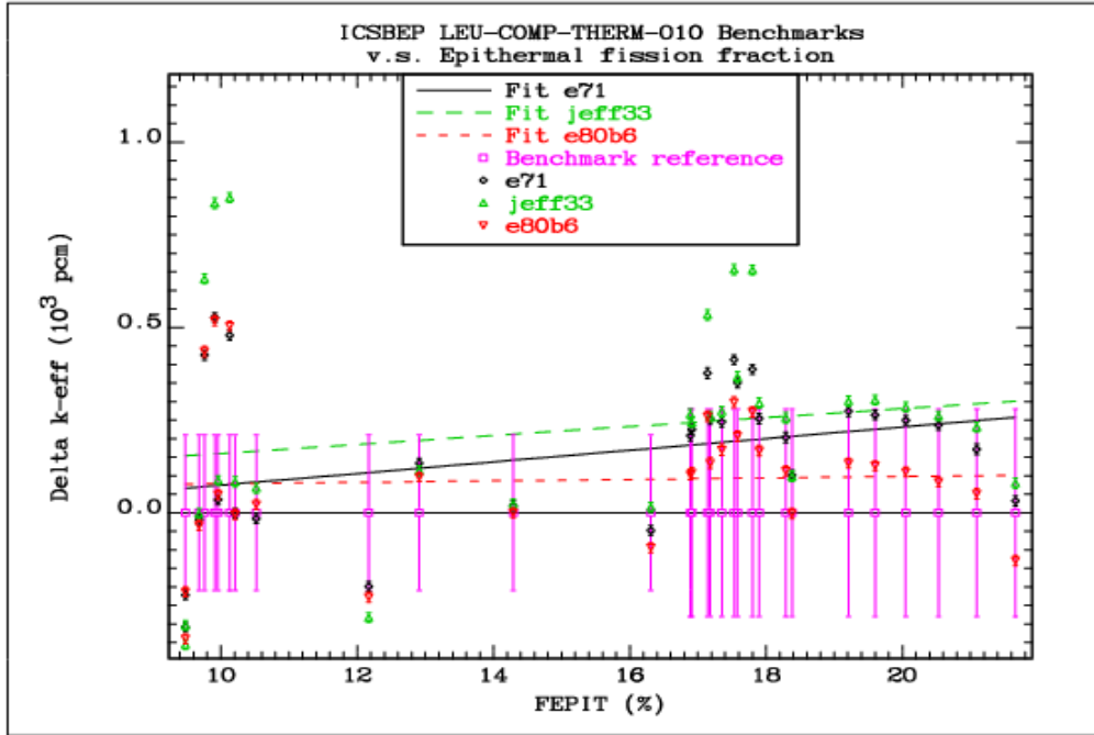
FIG. 6.1.5. Comparison of the differences between the calculated k_{eff} values and the reference benchmark values for the LEU-COMP-THERM-010 group of benchmarks as a function of the epithermal fission fraction.
