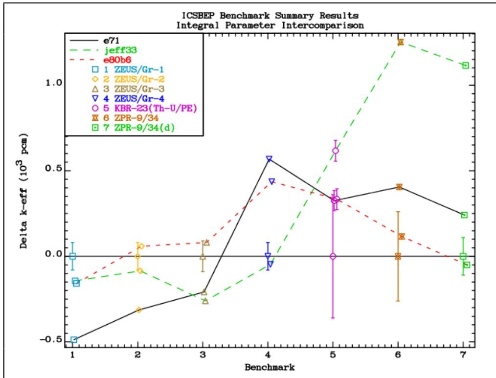
FIG. 4.6.1. Comparison of the differences between the calculated k_{eff} values and the reference benchmark values for the HEU-MET-INTER group of benchmarks.
