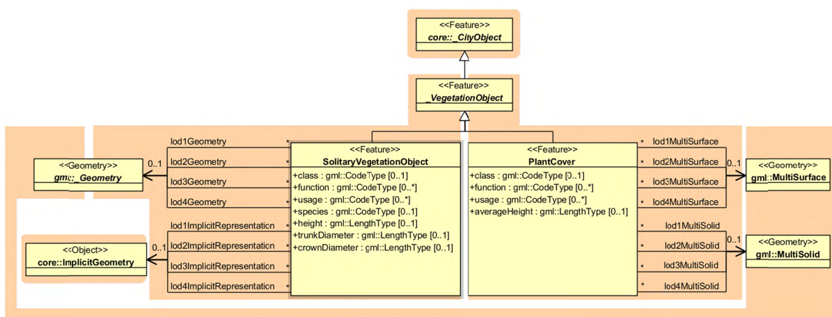
Figure 24: Vegetation Model
