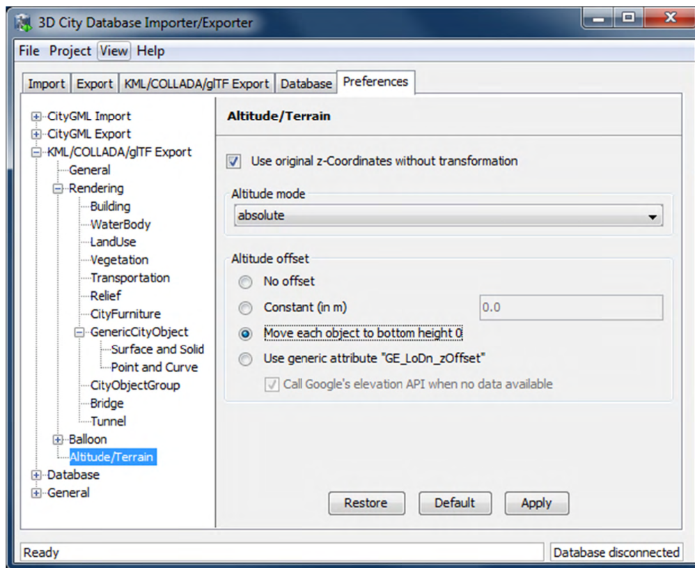
Figure 108: Altitude/Terrain settings.
