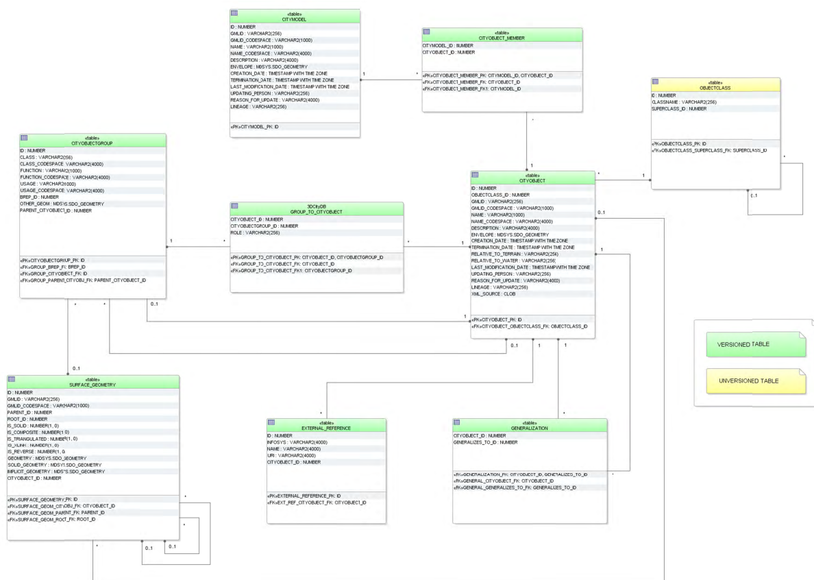
Figure 28: Database schema of the CityGML core elements
