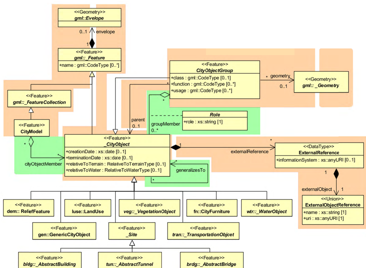
Figure 5: Core Model and thematic top level classes
