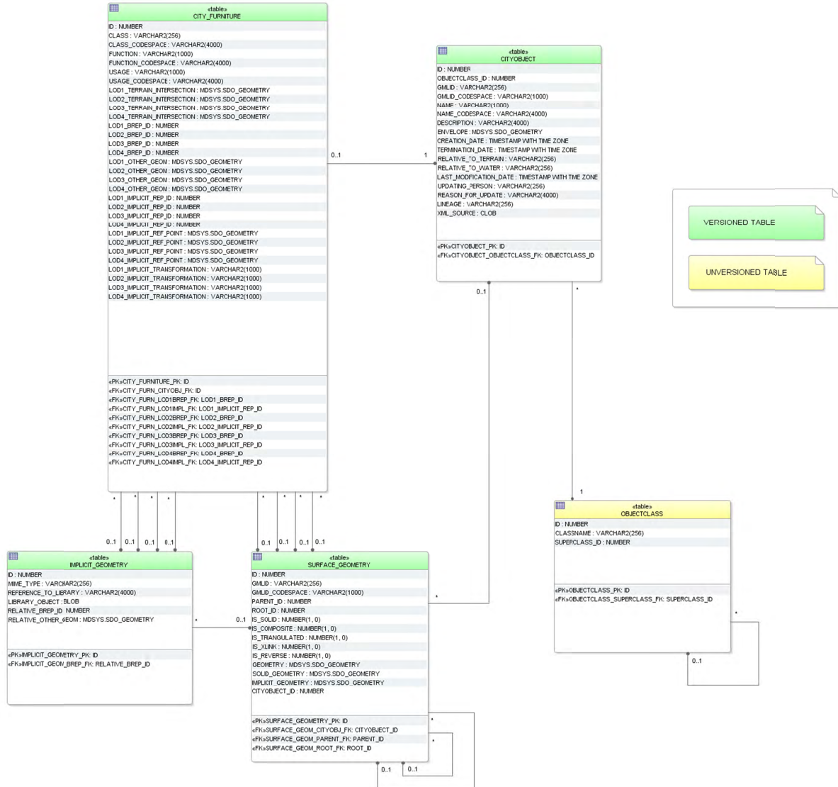
Figure 40: CityFurniture database schema
