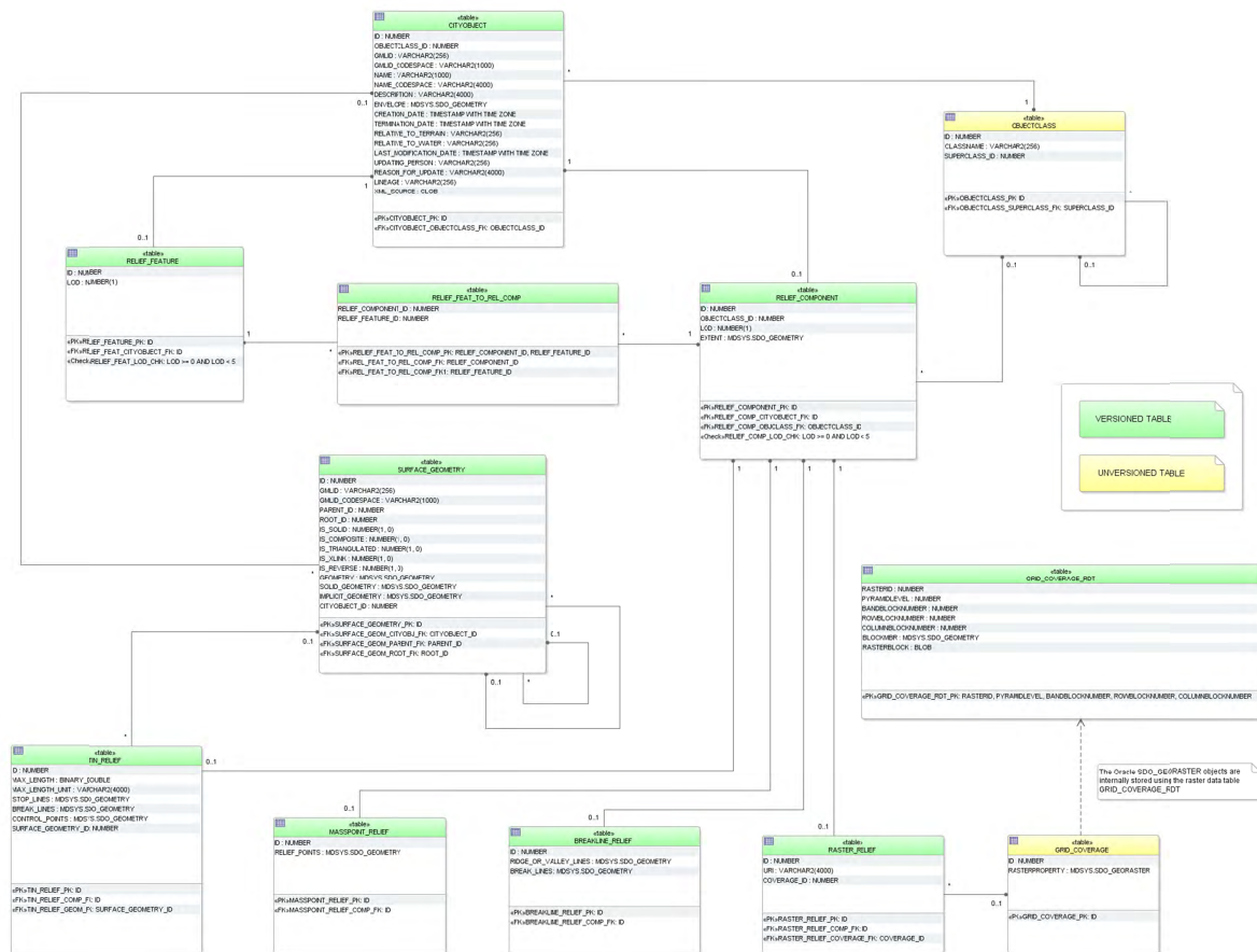
Figure 41: Digital Terrain Model database schema
