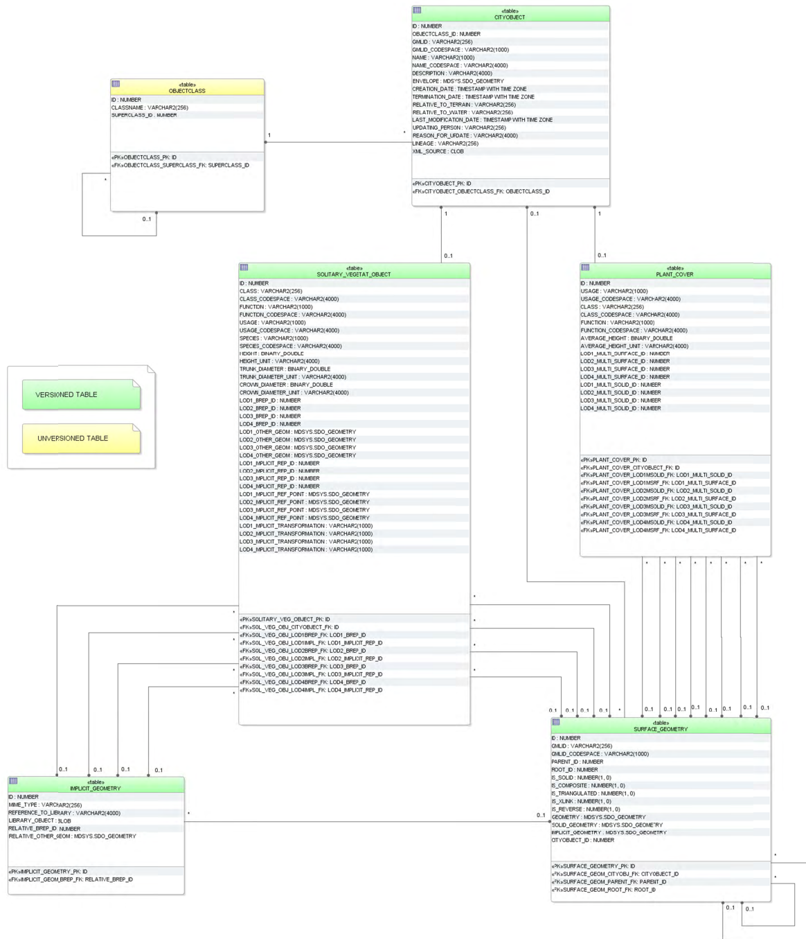
Figure 46: Vegetation database schema
