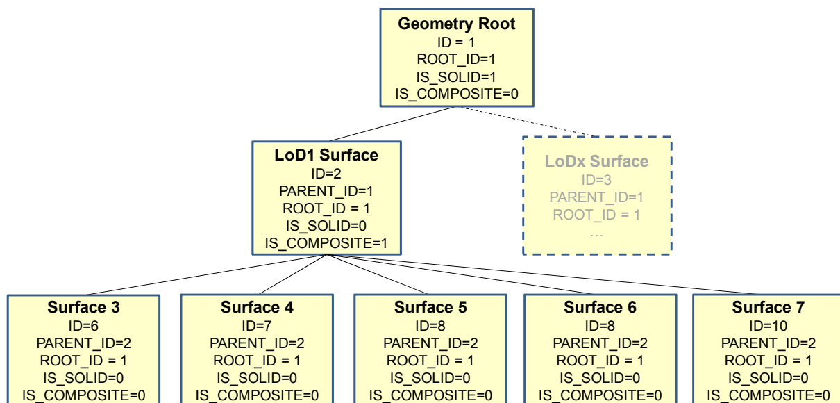
Figure 29: Geometry hierarchy for the solid geometry shown in Figure 30
