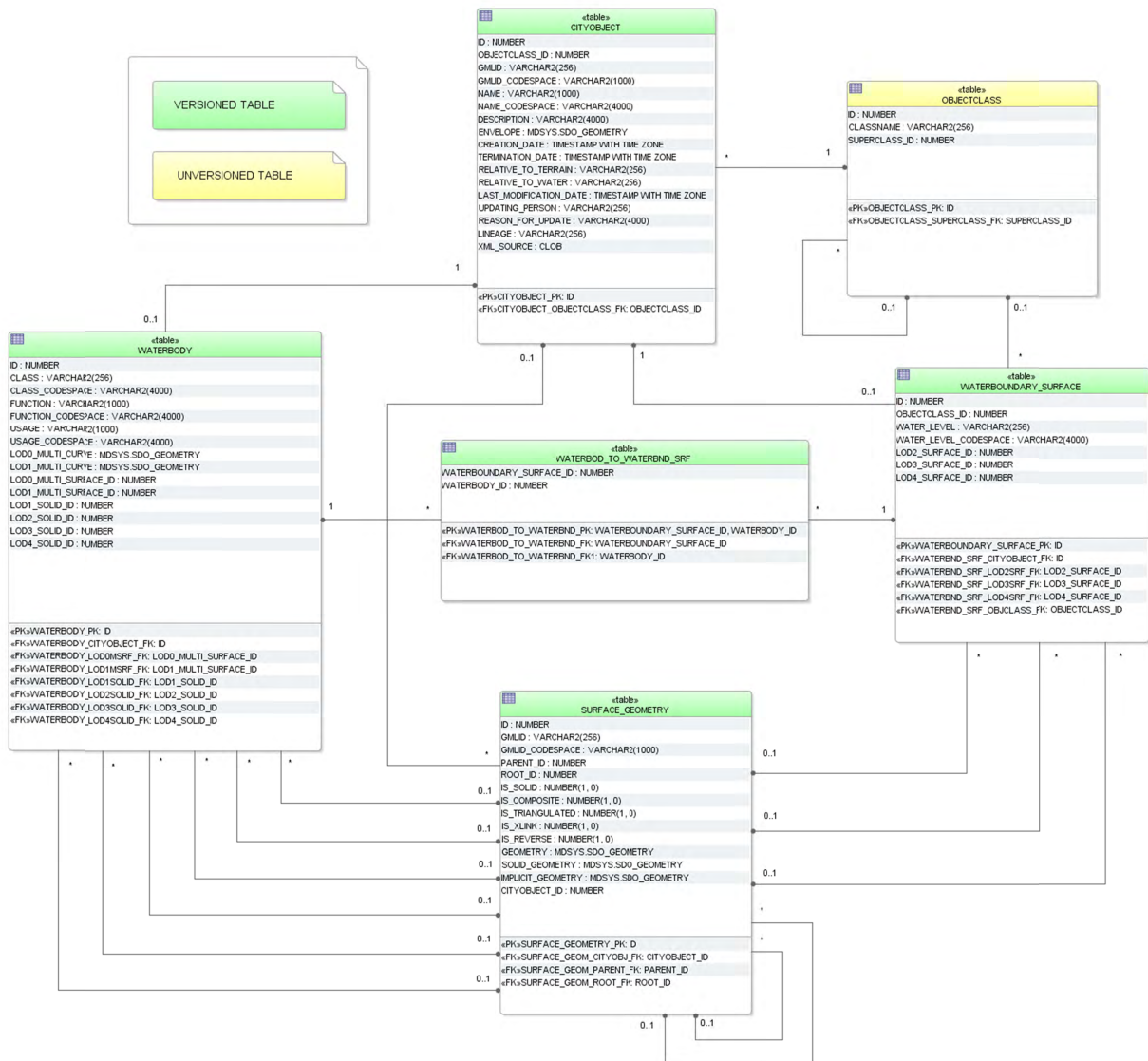
Figure 47: WaterBody database schema
