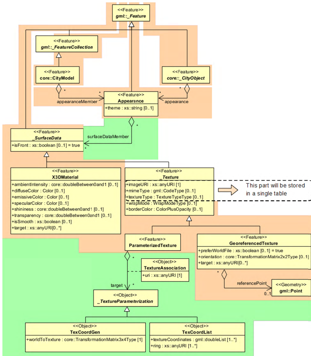
Figure 4: Appearance model
