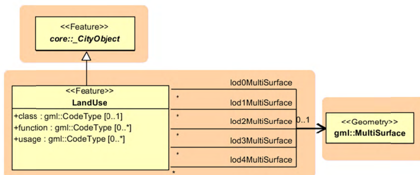
Figure 17: Landuse model
