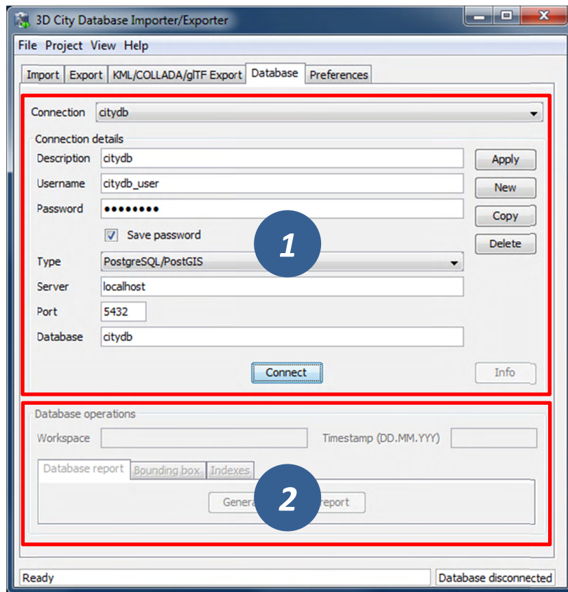
Figure 59: Database tab.
