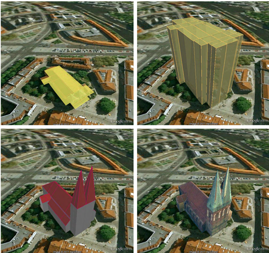
Figure 71: The same building displayed as (top down and left to right) footprint, extruded, geometry, COLLADA
