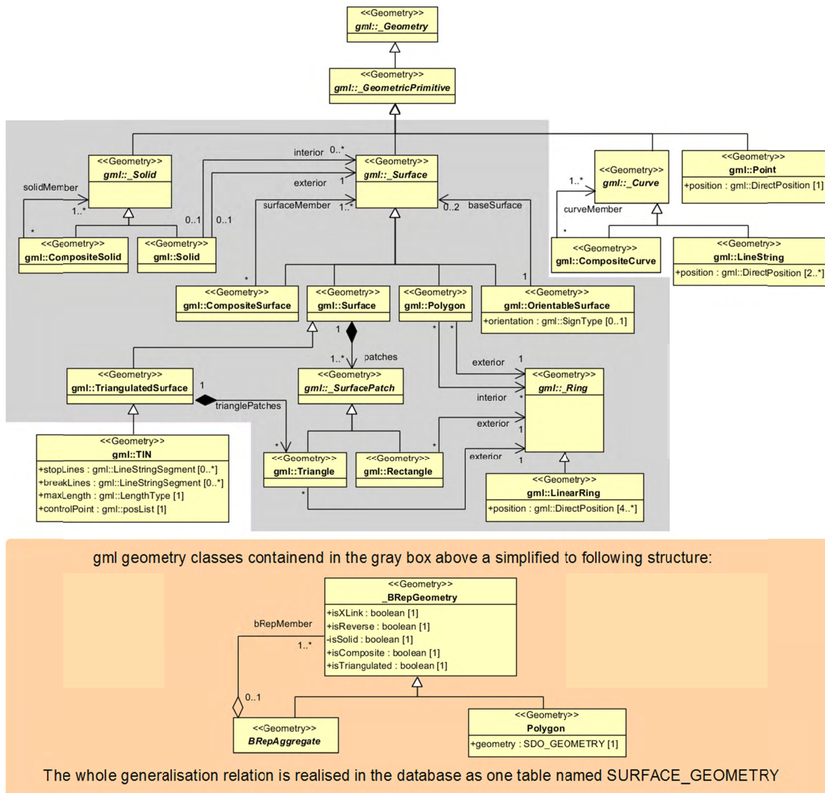
Figure 2: Geometrical-topographical model.
