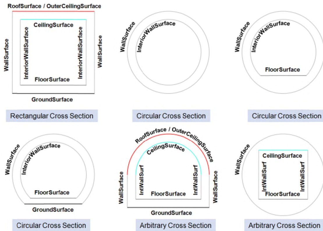
Figure 22: Different BoundarySurfaces of a tunnel
