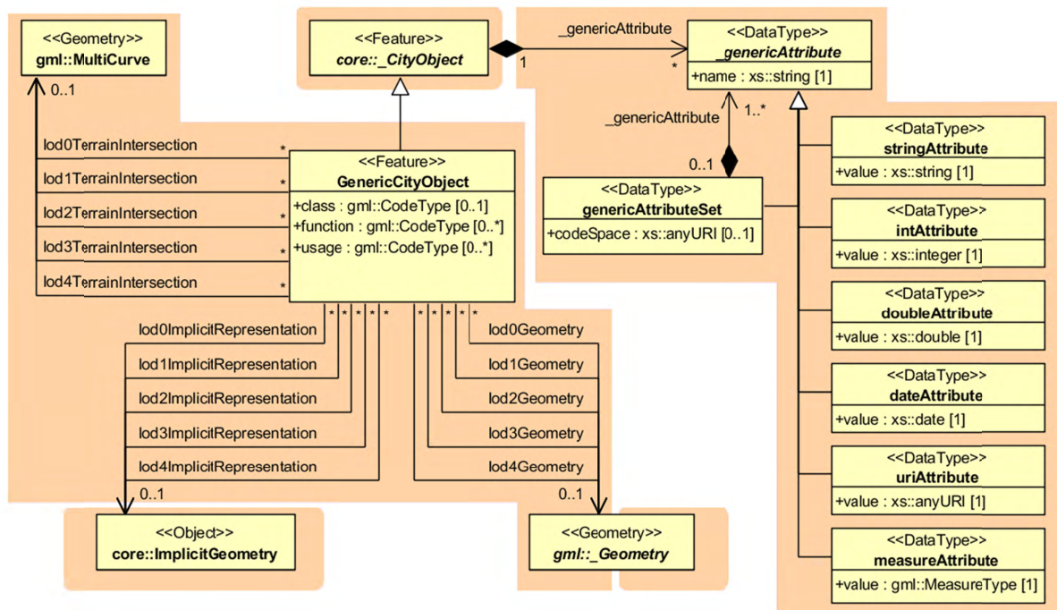
Figure 16: Generic CityObject model
