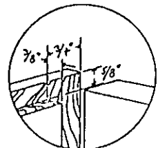
(B) DETAIL OF FRAME REST
