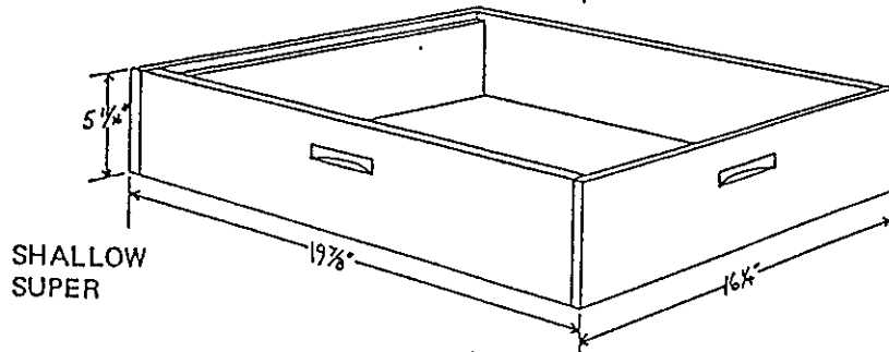
SHALLOW FRAME
