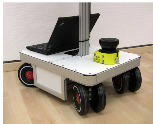
Fig. 2. Omnidirectional base with four individually steerable diff-drives.
