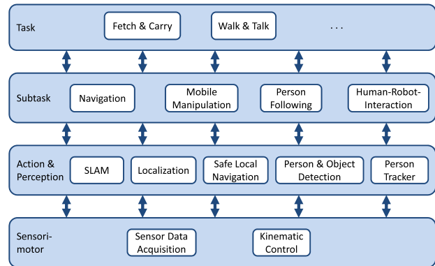
Fig. 4. Overview over the control modules within Dynamaid's behavior architecture.
