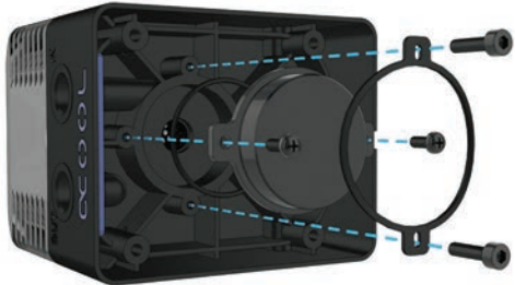
Installation DC-LT pump
