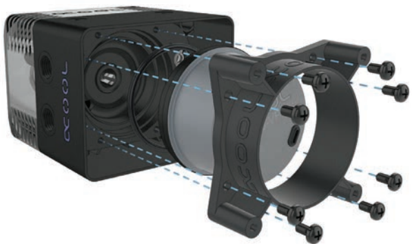
Installation VPP pump
