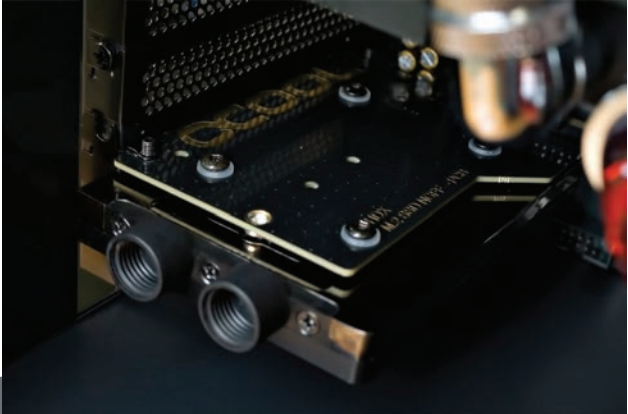
The HDX - M.2 SSD for one M2 SSD - passive cooled
