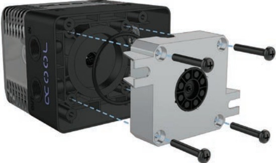
Installation DDC pump
