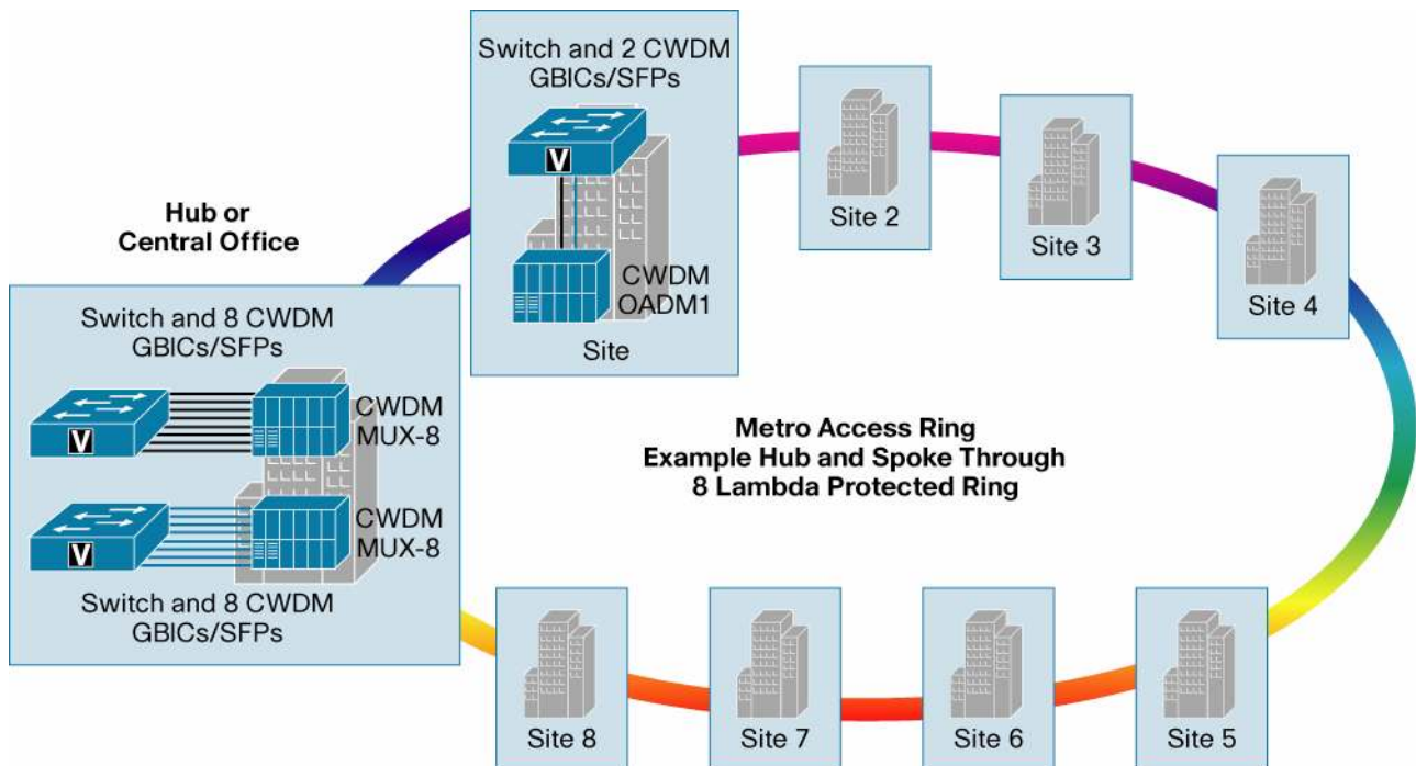
Figure 4. Hub-and-Spoke (Ring) Architecture
