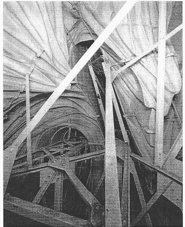
3.35. Statue of Liberty (1886), New York, architects Gustave Eiffel and Auguste Bartholdi: folds, armature and bracing.
