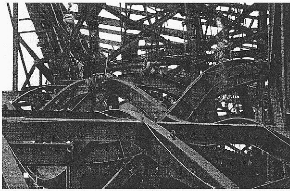
3.34. Assembly of the structural frame for the Disney Concert Hall (2003), Los Angeles, architect Frank Gehry.
