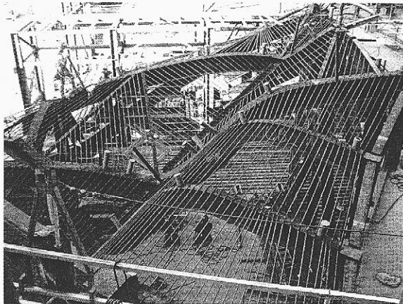
3.55a–c. Use of ruled surfaces in the Water Pavilion (1998), the Netherlands, architect Lars Spuybroek/NOX Architects.
