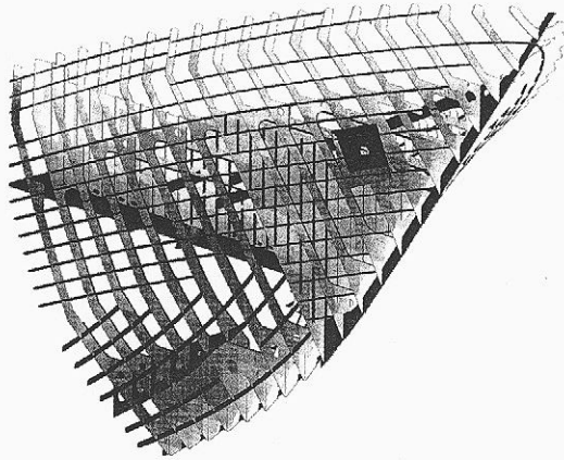
3.38. Structural framework for a ship's hull.
