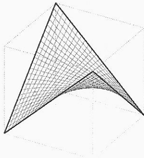
3.52. Ruled surface: hyperbolic paraboloid.
