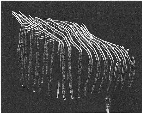
3.36a–b. Structural frames in Frank Gehry's Experience Music Project (2000) in Seattle were produced by contouring.
