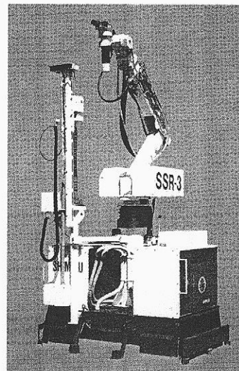
3.27. Shimizu's Insulation Spray Robot .
