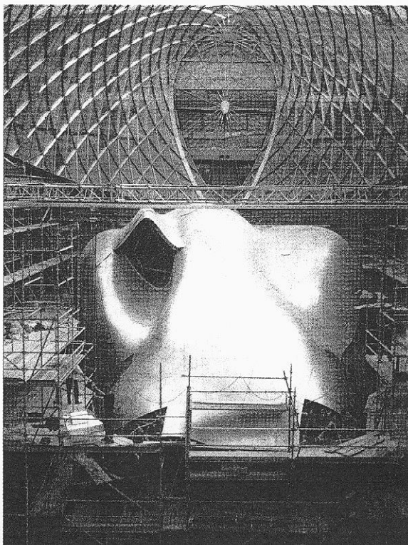
3.57. The doubly curved steel plates for the conference chamber of the DG Bank (2000), Berlin, Germany, architect Gehry Partners.
