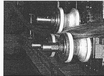
3.24a–b. The CNC bending of the aluminum profiles for the "Brandscape" BMW Pavilion at the 2000 Auto Show in Geneva, Switzerland, architects Bernhard Franken and ABB Architekten.
