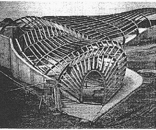
3.55a–c. Use of ruled surfaces in the Water Pavilion (1998), the Netherlands, architect Lars Spuybroek/NOX Architects.
