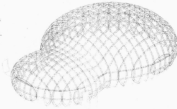
3.37. Structural framework for Bernhard Franken's "Bubble" BMW Pavilion produced by bi- directional contouring.
