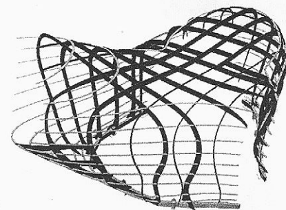
3.33a-b. Restaurant Georges : model of the monocoque shell for the "bar" volume.
