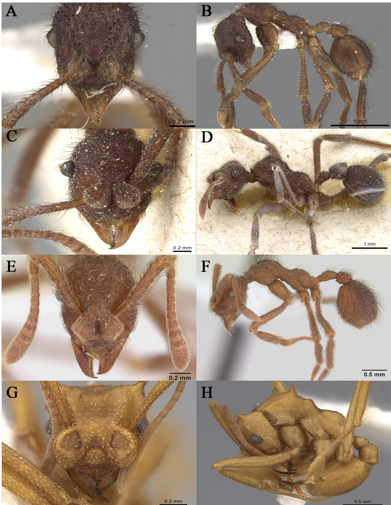
Figure 5. Apterostigma and Cyphomyrmex species encountered in Colombia. A, B. Apterostigma reburrum , CASENT0901686/ R. Perry. C, D. Apterostigma robustum , CASENT0904977/ Z. Lieberman. E, F. Apterostigma pilosum complex, CASENT0603533/ A. Nobile. G, H. Cyphomyrmex cornutus , CASENT0923103/ W. Lee. Photographs obtained from the Antweb database ( http://www.antweb.org ).
