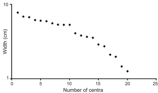
Fig. 8. Graphic representation of vertebral size decrease in Carcharomodus escheri (Agassiz, 1843) from anterior to posterior. Steps at positions 10-11, 14-15 and 18-19 indicate missing portions due to collecting and/or taphonomic artefacts.
