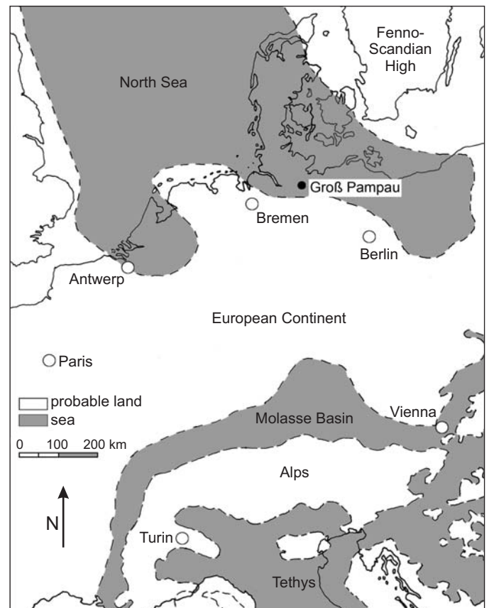
Fig. 1. Palaeogeographic map of mid-west Europe during the middle–late Miocene (compiled from Steininger et al. 1985; Huuse 2002; Rasmussen 2005) showing the locality Groß Pampau in a bay of the North Sea where the partial skeleton was recovered.
