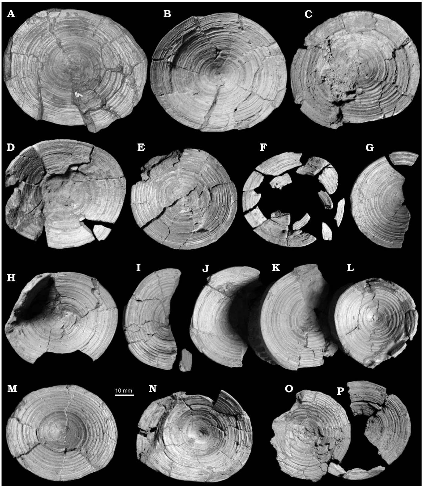
Fig. 5. Trunk vertebrae of the mackerel shark Carcharomodus escheri (Agassiz, 1843), MNU 071-20, from Groß Pampau, the middle-late Miocene, displaying the characteristic lamniform morphology and concentric growth bands from anterior (A) to posterior (P).
