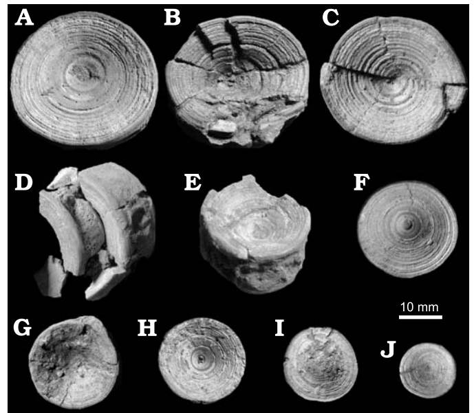
Fig. 7. Posteriormost precaudal and caudal vertebrae of the mackerel shark Carcharomodus escheri (Agassiz, 1843), MNU 071-20, from Groß Pampau, the middle-late Miocene, from anterior (A) to posterior (J).
