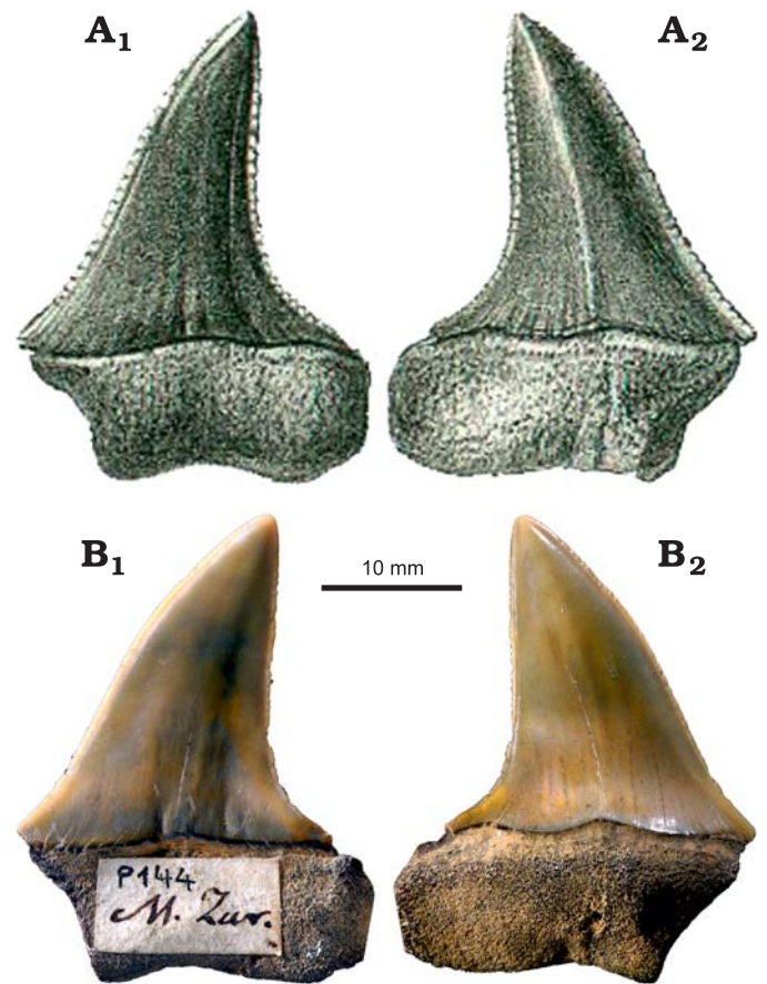
Fig. 4. Holotype of the mackerel shark Carcharomodus escheri (Agassiz, 1843) from the Upper Marine Molasse (Burdigalian-Ottngian, early Miocene) of Switzerland. A. Original drawings of Agassiz (1843: pl. 36: 16–18), in labial (A 1 ) and lingual (A 2 ) views. B. Photographs of holotype (ETZ 000000001750), in labial (B 1 ) and lingual (B 2 ) views.
