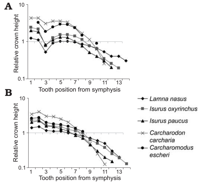
Fig. 13. Relative crown heights of the reconstructed dentition of Carcharomodus escheri (Agassiz, 1843) in comparison to living lamnids. Upper (A) and lower (B) jaw. Scaled logarithmically.
