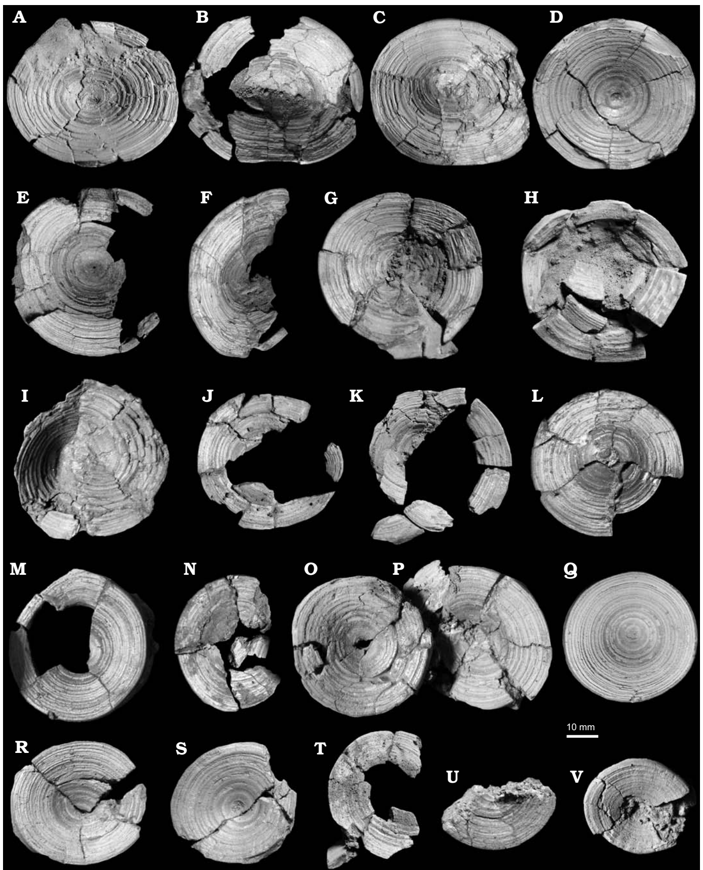
Fig. 6. Trunk and precaudal vertebrae of the mackerel shark Carcharomodus escheri (Agassiz, 1843), MNU 071-20, from Groß Pampau, the middle-late Miocene, from anterior (A) to posterior (V).
