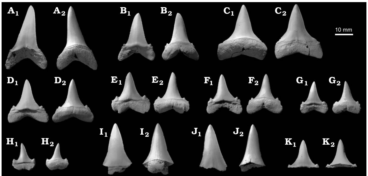
Fig. 11. Lower jaw teeth of the mackerel shark Carcharomodus escheri (Agassiz, 1843), MNU 071-20, from Groß Pampau, the middle-late Miocene. A. Lower left anterior tooth. B. Lower left intermediate tooth. C–H. Lower lateral teeth. Labial ( A_1 – H_1 ) and lingual ( A_2 – H_2 ) views. I. Incomplete anterior lower lateral tooth. J, K. Incompletely mineralized lower replacement teeth.
