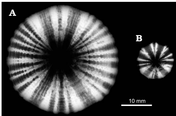
Fig. 9. Radiographs of vertebrae of the mackerel shark Carcharomodus escheri (Agassiz, 1843), MNU 071-20, from Groß Pampau, the middle-late Miocene. A. Precaudal vertebra, same as in Fig. 6Q. B. Caudal abdominal/caudal vertebra, same as in Fig. 7J.
