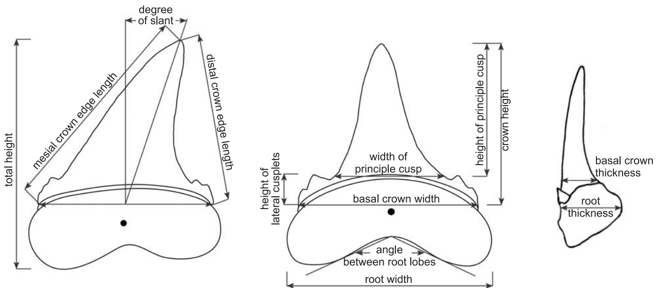
Fig. 3. Tooth measurements used in this study.
