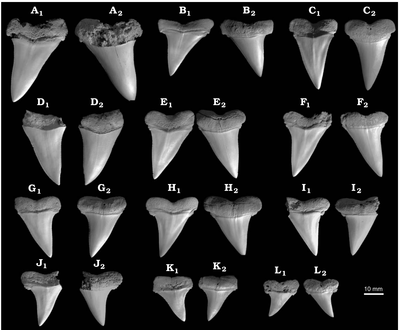
Fig. 10. Upper teeth of the mackerel shark Carcharomodus escheri (Agassiz, 1843), MNU 071-20, from Groß Pampau, the middle-late Miocene. A. Second upper right anterior tooth. B. Right upper first lateral tooth. C–L. Left (C, D, G, I, K) and right (E, F, H, J, L) upper teeth. Labial (A 1 –L 1 ) and lingual (A 2 –L 2 ) views. For positions of lateral teeth within jaw see Fig. 12.
