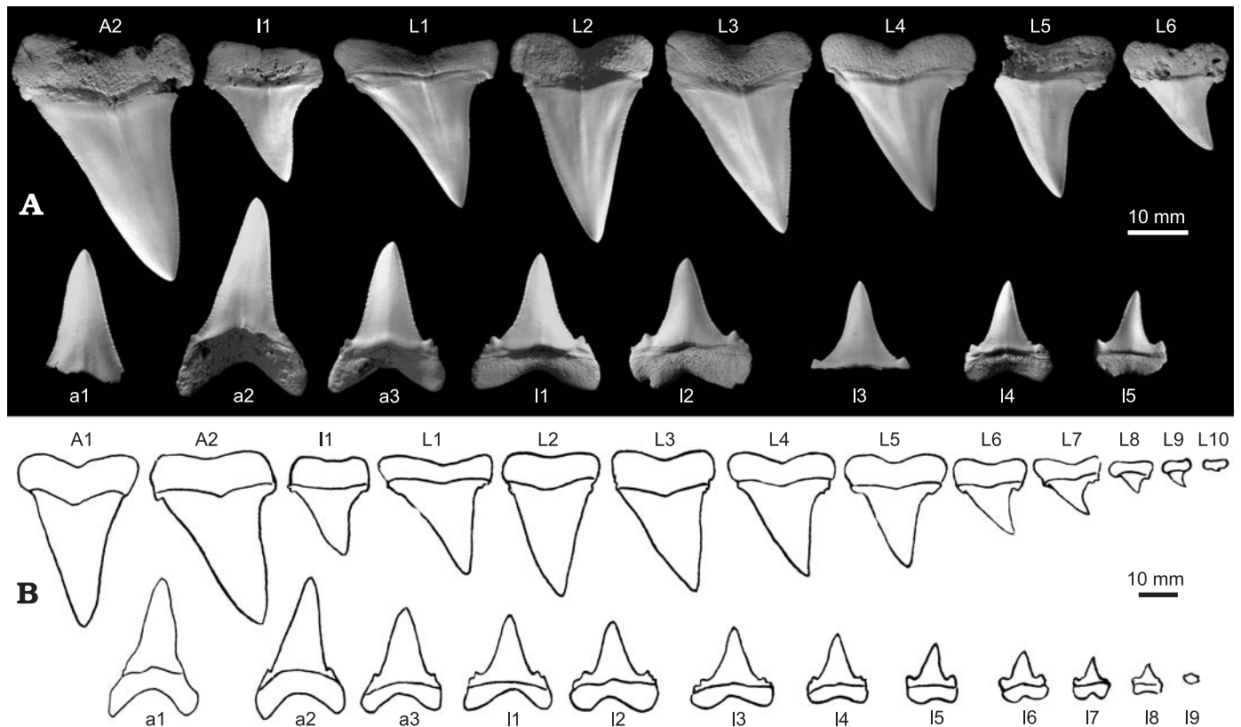
Fig. 12. Reconstructed left upper and lower tooth rows of the mackerel shark Carcharomodus escheri (Agassiz, 1843), in lingual view. A. Reconstruction based on preserved teeth. B. Drawing of the completely reconstructed dentition based on preserved teeth and comparisons with living lamnid sharks.
