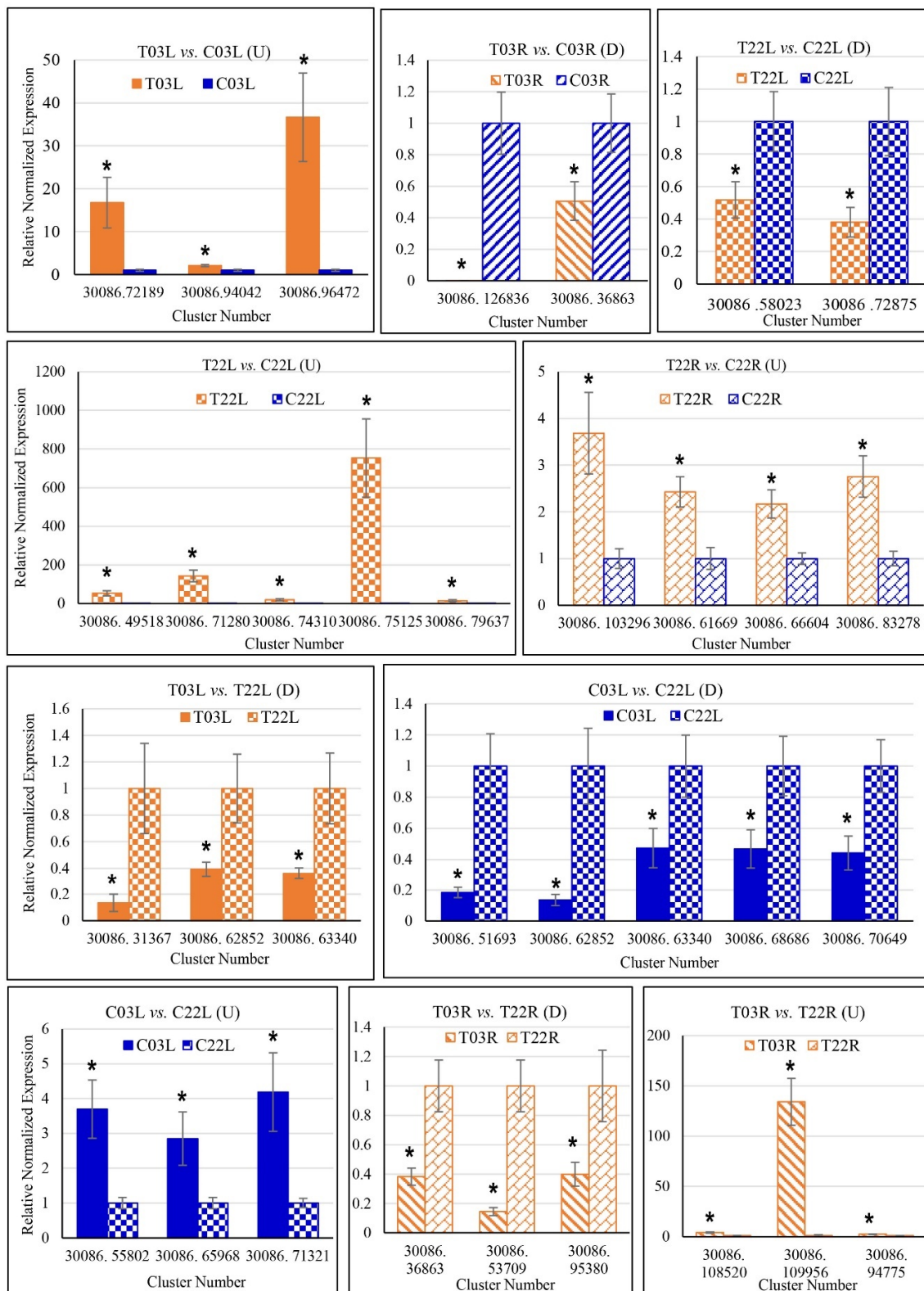
Figure 2. qRT-PCR validation of gene expression observed through RNA-Seq analysis. The y-axis indicates relative normalized expression, and the x-axis indicates cluster number (gene IDs). Graphs for upregulated (U) and downregulated (D) genes are shown separately. An asterisk (*) indicates a significant difference (t-test at p \leq 0.05 ). T03L, Treatment '03' Leaf; C03L, Control '03' Leaf; T22L, Treatment '22' Leaf; C22L, Control '22' Leaf; T22R, Treatment '22' Root; C22R, Control '22' Root, T03R, treatment '03' Root, and C03R, Control '03' Root.
