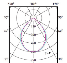
(cd/1000lm) 0-180° 90-270° Optional: SM340C, MLO, BAP-tauglich
