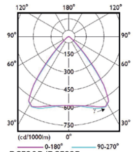
RC530B/RC532B, BAP-tauglich
