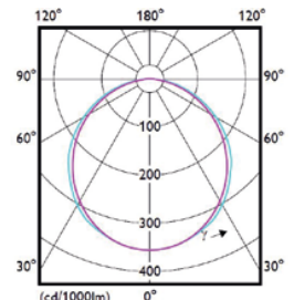
SM531C, opal
