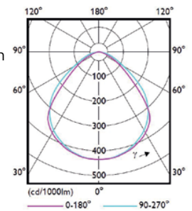
SM134V NOC
