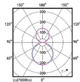
SP543P, opal
