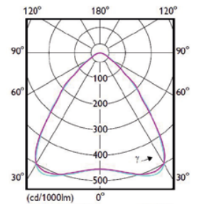
(cd/1000lm) 0-180° 90-270° SM340C, PCS, BAP-tauglich
