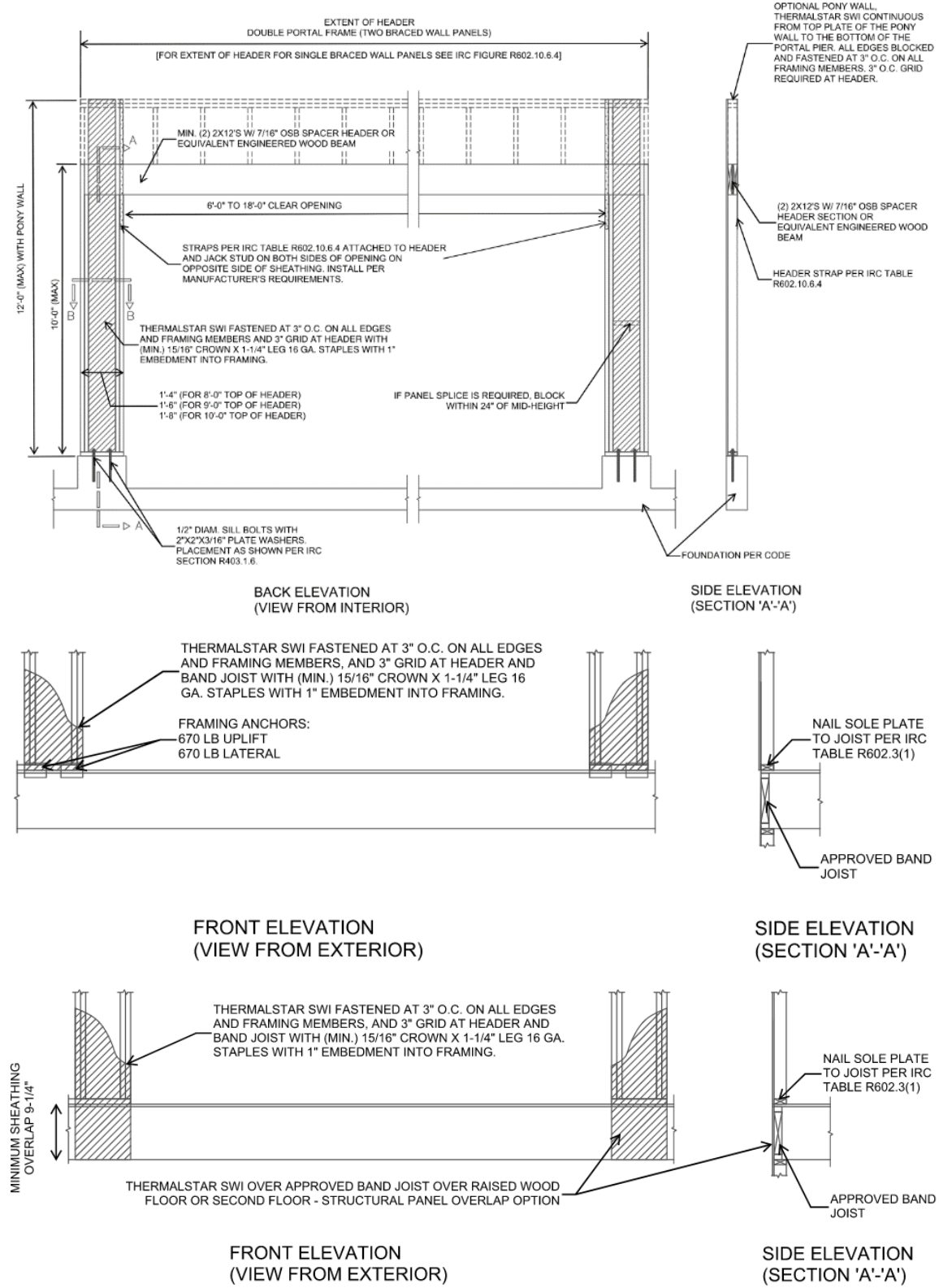
Figure 2. ThermalStar® SWi Structural Sheathing CS-PF
