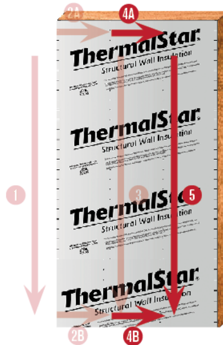
Figure 8. Installation: Step 4 and Step 5
