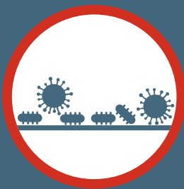
Contamination of surfaces with bacteria, viruses, fungus and spores
