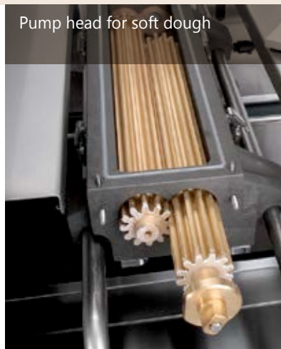
Volumetric pump head for soft dough
