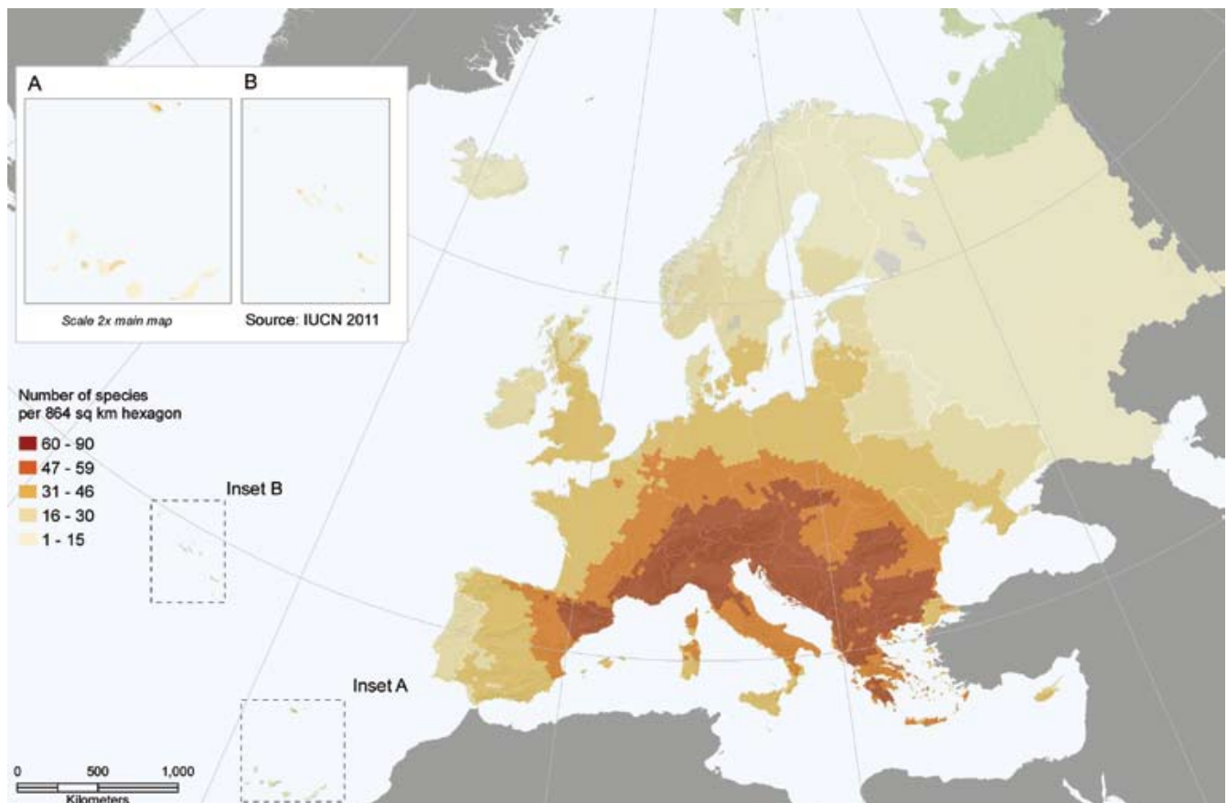
Figure 15. Species richness of selected families of European terrestrial molluscs
