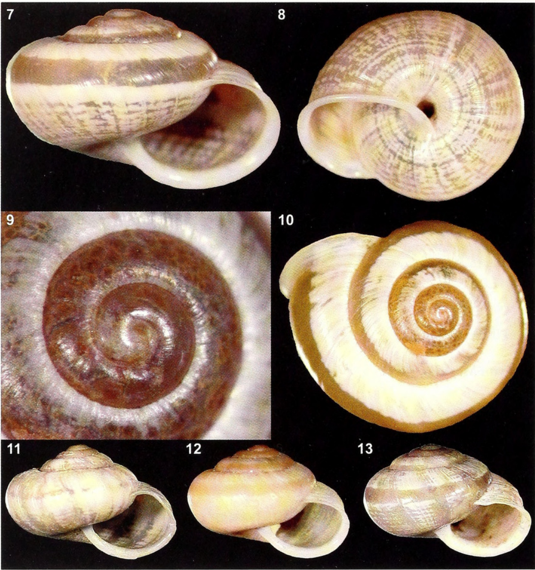
Figures 7–13. Shells of Praticolella mexicana new species. 7–10. Holotype, SW of Linares, Nuevo León, Mexico, 27 May 1992, Ned E. Strenth, ANSP 426031; side, top, and basal views of the shell and embryonic whorls, w=9.58 mm, h=6.59 mm, 5.25 whorls. 11. ANSP 426020, Hidalgo, Hidalgo Co. Texas, w=10.59, h=7.46, 5.25 whorls, 21 Sept. 1991, Ned E. Strenth coll. 12. ANSP A22090, College of the Bahamas Research Station, Staniard Creek, Andros Island, Bahamas, w=10.57, h=7.63, 5.25 whorls, 20 May 2005, K.E. Perez coll. 13. ANSP 426026, Canoas, San Luis Potosí, Mexico, w=9.79 mm, h=7.18 mm, 5.25 whorls, 23 July 2002, K.E. Perez, J.B. Pollock colls.
