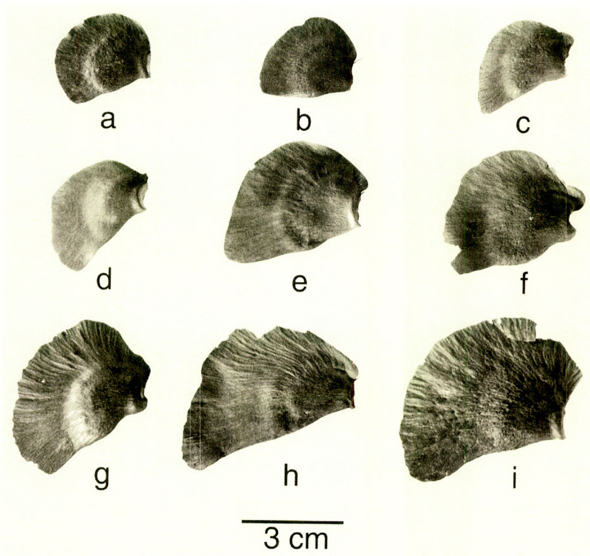
FIG. 3. Samaras of Heteropterys leona from the New World. a. Brazil (Maguire et al. 47120, NY). b. French Guiana (Cremers & Hoff 11239, US). c. Nicaragua (Moreno & Sandino 12141, MO). d. Honduras (Vargas et al. 355, NY). e. Guyana (Gillespie 1203, MICH). f. Colombia (Albert de Escobar 3245, NY). g. Jamaica (Britton 1484, NY). h. Colombia (Cuatrecasas 15936, US). i. Guyana (Fanthaw 531, NY).
