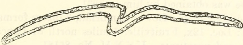
FIGURE 1.—Diagrammatic cross section of the holotype of Camptostroma rodnyi , showing fold on both the upper and under sides produced by lateral compression
