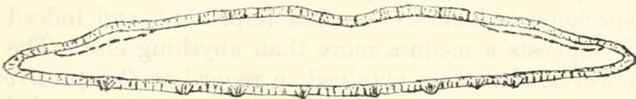
FIGURE 2.—Vertical section of Camptostroma rodnyi , showing the layer of coenenchym with the thecal pores on upper and under sides and monticules on underside. The dotted lines indicate extent of ribs
