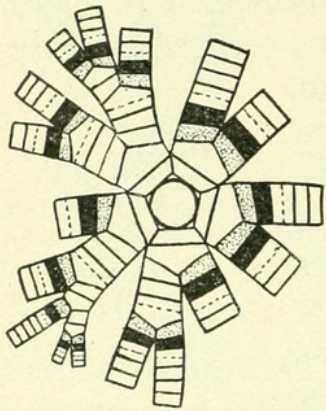
FIG. 19.—THALASSOMETRIDÆ; CHARITOMETRA.
