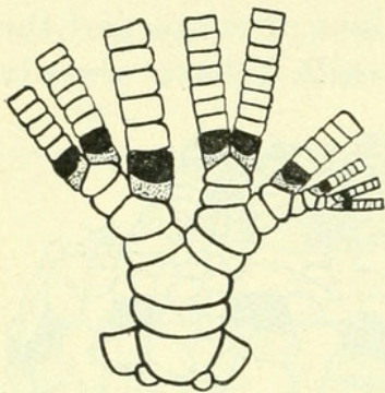
FIG. 26.—PENTACRINITIDÆ; ENDOXOCRINUS.
