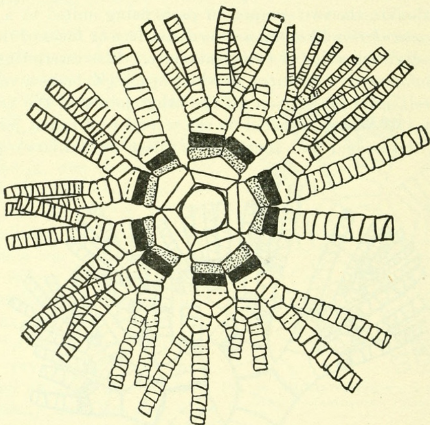
FIG. 24.—COMASTERIDÆ; COMASTER.
