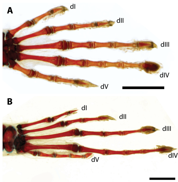
Figure 2. Forelimb (A) and hindlimb (B) of Cercosaura schreibersi , showing the generalized phalangeal arrangement. Digit identity is indicated as dI-dV. Anterior to the top. Scale bar = 1mm.
