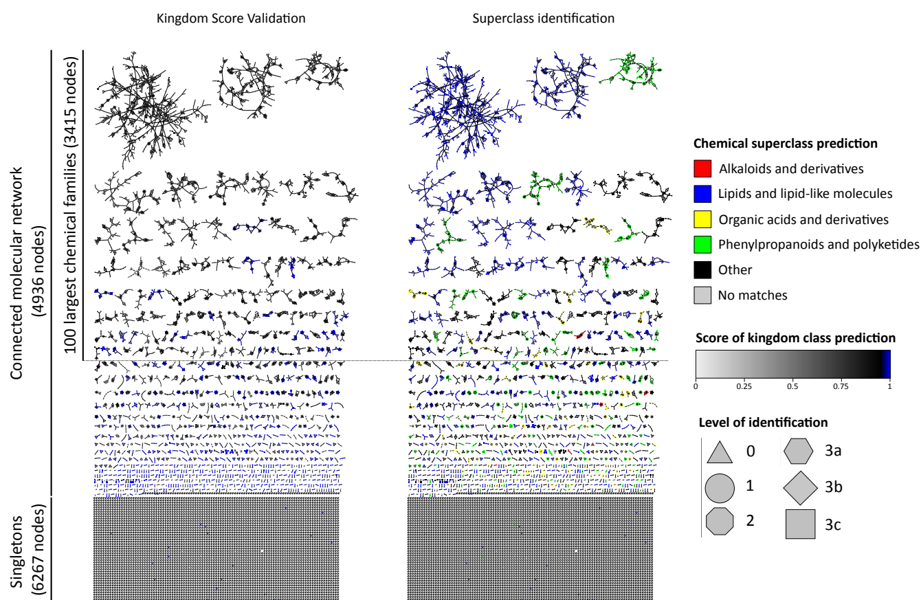
Figure 2. Validation of dereplication in the global molecular network of Mycoporeae. The global molecular network of Mycoporeae comprises a connected part, with clusters of spectral features that represent structurally-related putative metabolites, as well as singletons, which represent features that did not show spectral similarity to another one. The connected dataset was dereplicated using public, in house and in silico spectral libraries and subsequent Network Annotation Propagation (NAP). Identification of nodes took place on six different levels, with level 1: m/z , retention time and MS^2 match using in house spectral library; level 2: MS^2 match using in house and public spectral libraries; level 3a-c: Fusion, Consensus or MetFrag algorithm based in silico fragmentation database match; level 0: no spectral match. The presented network on the left, displays a kingdom score based assessment with overall high scoring values that support a robust dereplication of the corresponding chemical families. The network on the right side displays NAP-generated chemical superclass prediction for each chemical family, with selected classes highlighted in colour.
