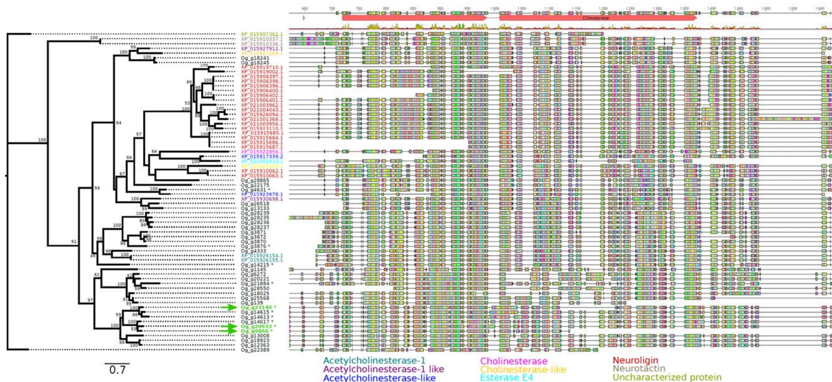
Fig. S18. Alignment (COBALT) and maximum likelihood tree of the encoded protein sequences of all Acetylcholinesterase (AChE) related genes of O. gibbosus (“Og_x”) and those of the spider Parasteatoda tepidariorum (“XP_x”). The tree was constructed on the COBALT alignment with RAxML v. 8.2.11 using the WAG substitution model and gamma distributed rate variation among sites. Bootstrap values are presented next to the branches. The AChE genes located on the hunch-specific sequence are indicated with a green arrow, while those located outside the hunch-specific sequence are indicated in black. Sequence names of P.tepidariorum are color-coded according to their predicted function.
