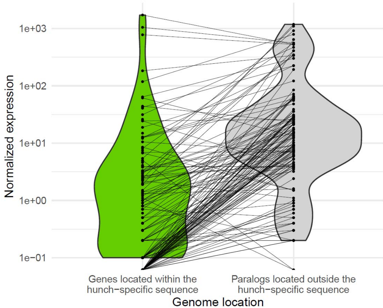
Fig. S16. Comparison of the distribution of normalized gene expression of coding sequences (CDS) located on the hunch-specific sequence and their closest paralogs located outside this sequence fragment. Dots represent individual CDS connected with their closest paralog.
