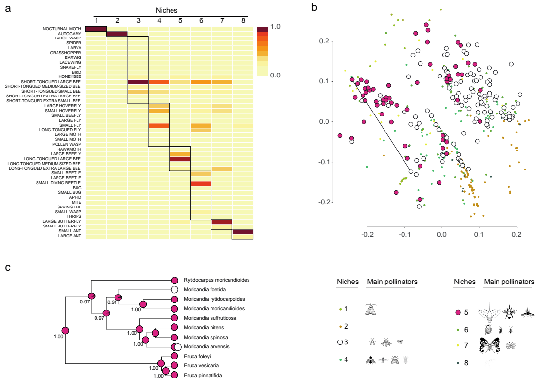
820 Figure 3. Plasticity-mediated changes in pollination niches. (A) Outcome of the modularity 821 analysis showing the number of pollination niches inferred, the among-niche differences in 822 relative frequency of each pollinator functional group, and the pollinator functional groups defining 823 the niches (n = 511 Brassicaceae species). (B) Morphospatial distribution of the eight pollination 824 niches detected in Brassicaceae. Insect silhouettes were drawn by Divulgare ( www.divulgare.net ) 825 under a Creative Commons license ( http://creativecommons.org/licenses/by-nc-sa/3.0 ). (C) 826 Estimate of the ancestral pollination niche of the Moricandia lineage using a stochastic character 827 mapping inference analysis. The numbers underneath each ancestral node indicate the posterior 828 Bayesian probability of belonging to pollination niche 5.
