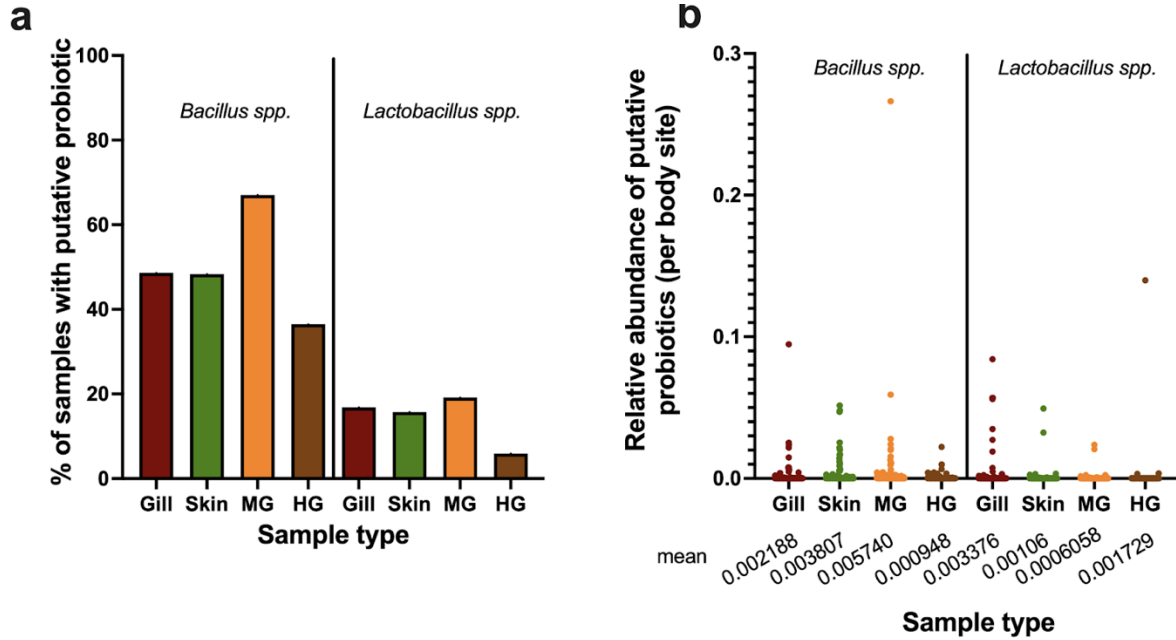
Supplemental Figure 4 Probiotic. Distribution of putative probiotic ASVs grouped by genera: Bacillus or Lactobacillus . a) The total percentage of samples within a given body site having either a Bacillus ASV or Lactobacillus ASV. b) The relative abundances of Bacillus and Lactobacillus ASVs within each body site (including samples with 0 counts).
