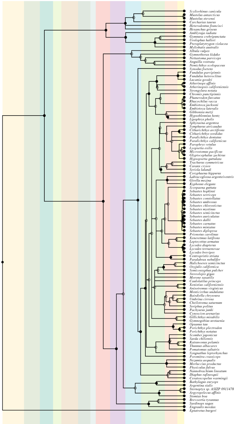
Supplemental Figure 3. Phylogenetic tree of fish species used in "FMP" beta diversity analysis
