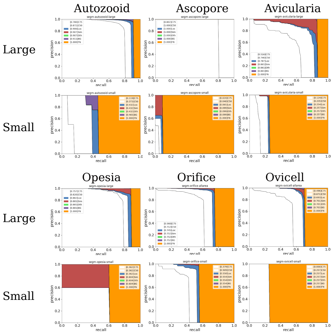
Figure S2 - Precision-recall (PR) curves for all six classes of objects, broken down according to structure size (small vs large). The area in white defines the PR curve for an IoU value of 0.5. By adding the blue area (Loc), it becomes the PR curve while ignoring localization error (IoU of 0.1). By adding the area in red (Sim), it becomes the PR curve while ignoring classification errors (e.g. mistaking an ovicell as an autozoid). By adding the area in purple (BG), it becomes the PR curve including false positive errors. Finally, the area in orange (FN) represents the false negatives.
