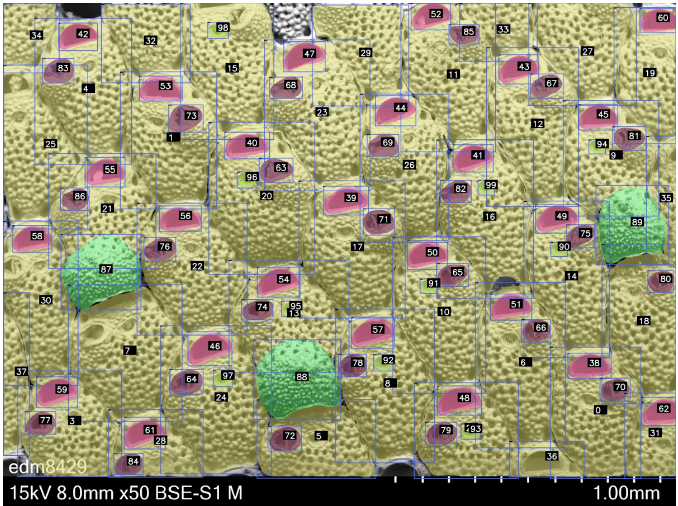
Figure S1 - Prediction layout shown by the DeepBryo app when activating the option to show bounding boxes (blue) and the structure-level identification numbers (squares with dark background). ID numbers can be used to filter the output table.
