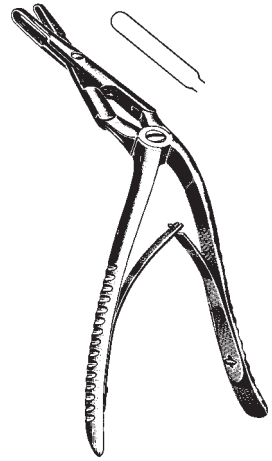
MIDDLETON-JANSEN 47325-19 19 cm, 7 1/2"
