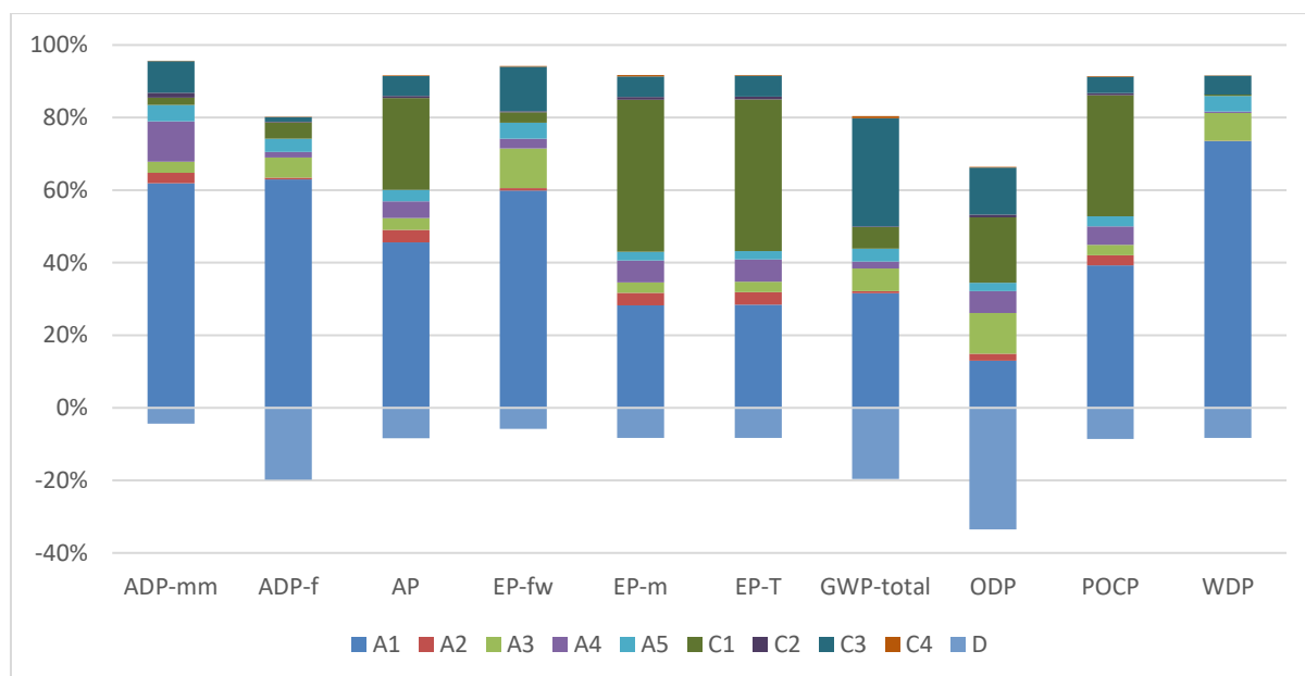
Figure 2: Tensar® TriAx® TX150 - Impact of the individual modules on the environmental core indicators (NMD set 2)
