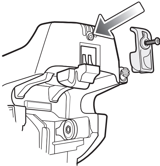
Figure 7-15 Locking Mechanism
