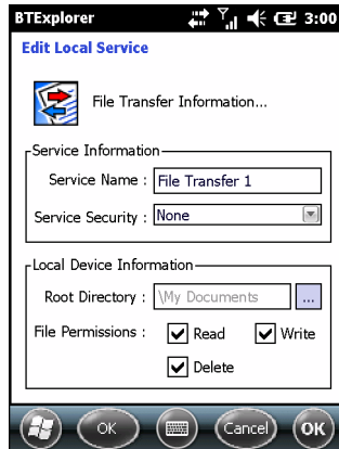
Figure 5-31 BTE Explorer Settings - File Transfer Information
