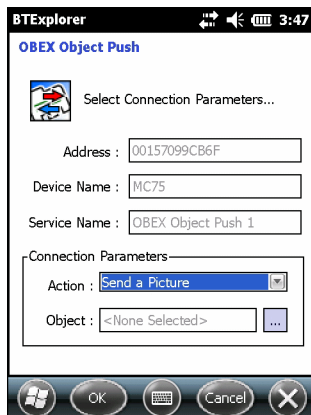
Figure 5-22 OBEX Object Push Window
