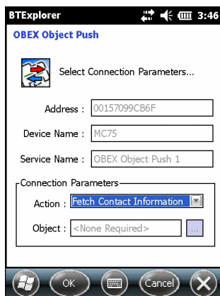
Figure 5-21 OBEX Object Push Window
