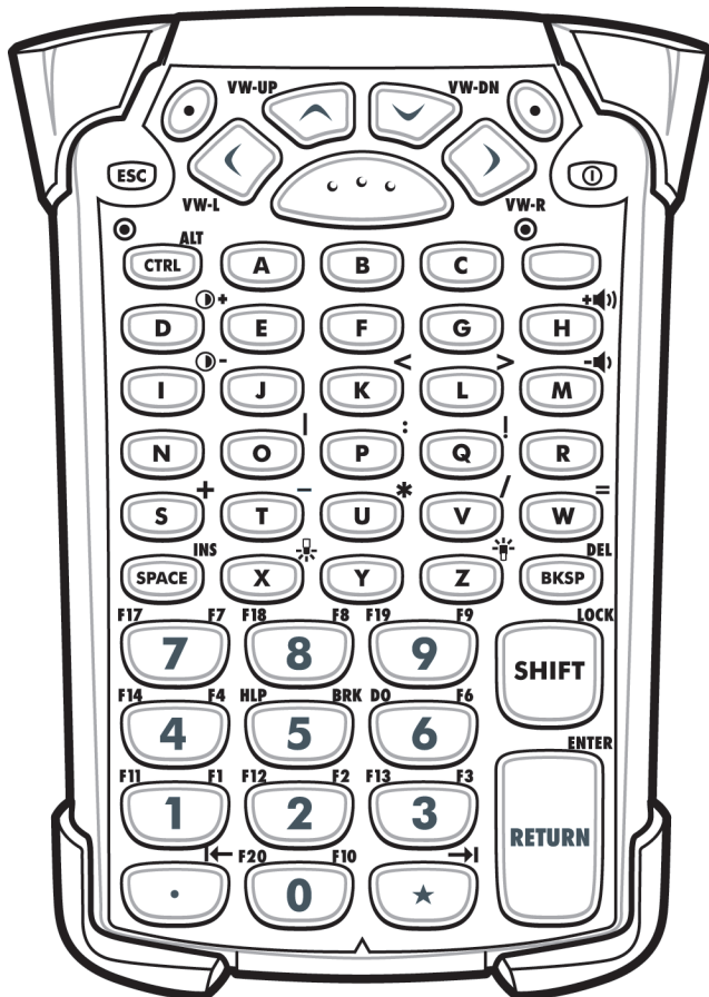
Figure B-6 VT Emulator Keypad
