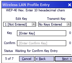
Figure 2-21 WEP-40 WEP Keys Dialog Box
