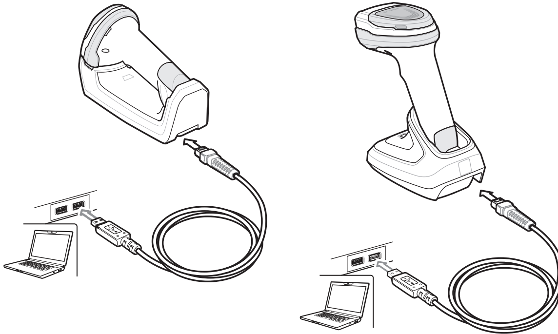
Figure 8-1 USB Connection
