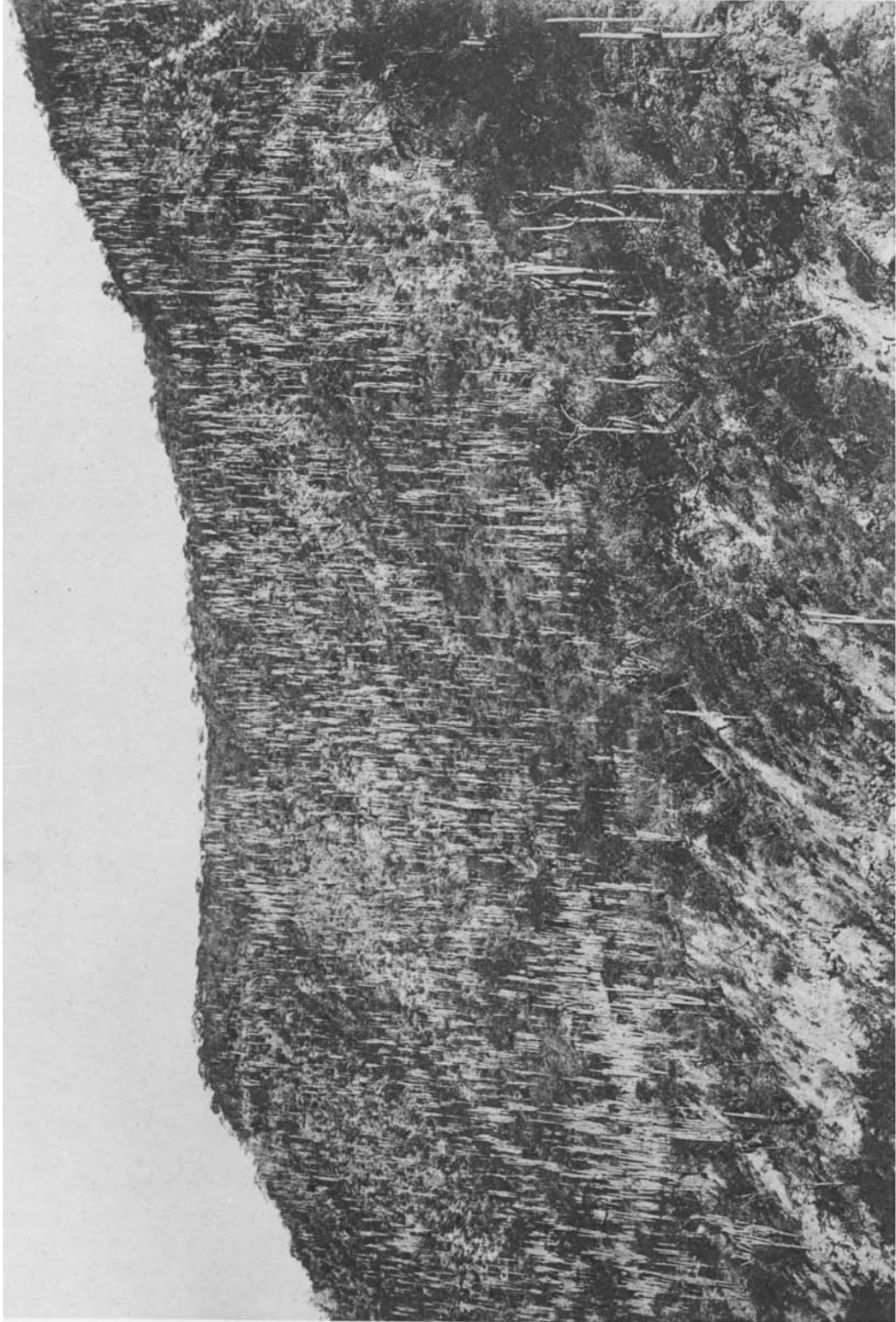
A mountain-side along Tomellín Canyon, Mexico, covered with Pachycereus columnna-trajani .
