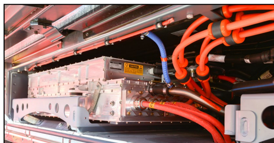
EXRAD ® HV Cables in a Hybrid System on a Commercial Bus.
