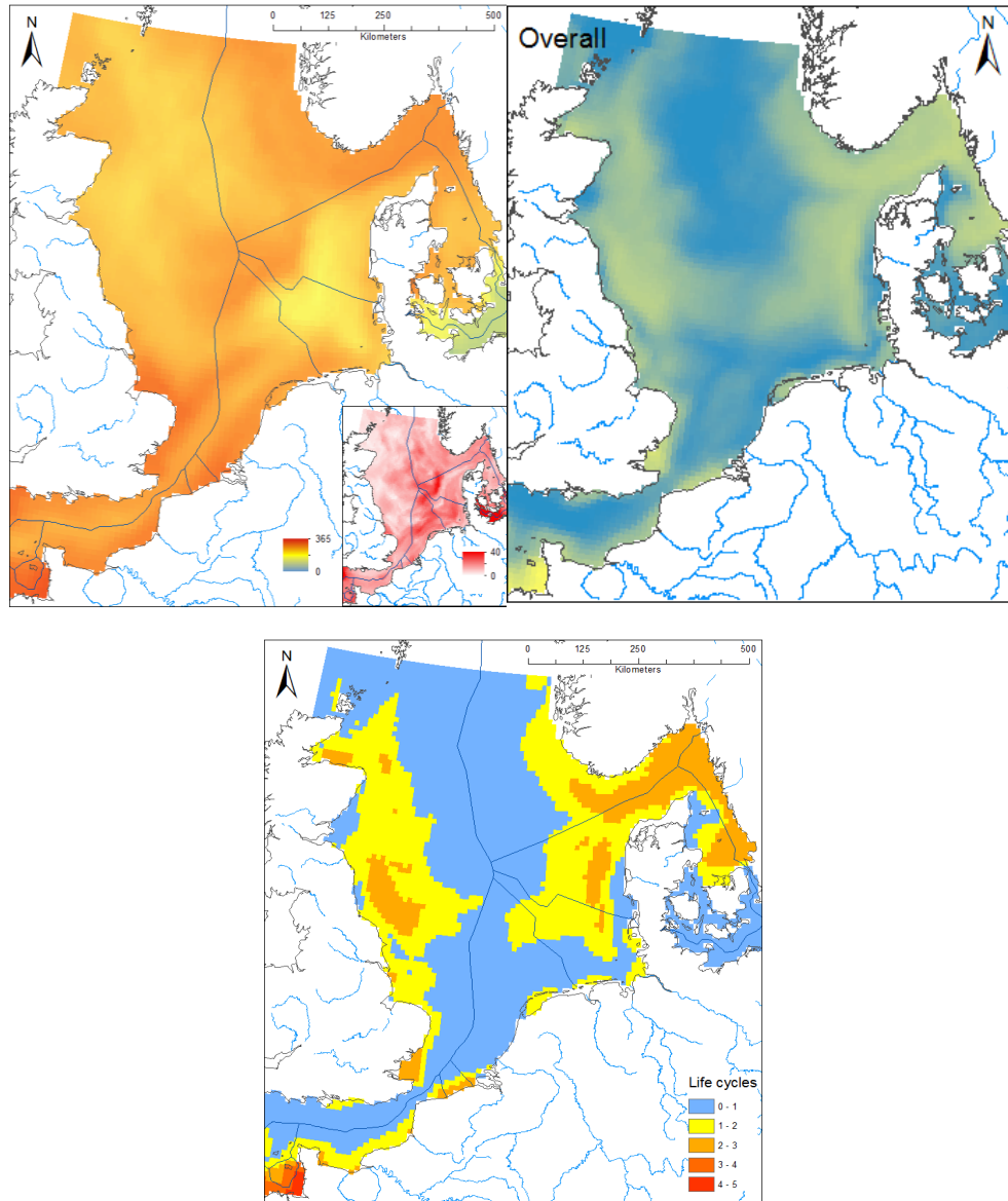
Figure 1. Maps showing the average (for 2005–2011) number of days per year suitable for survival of Mnemiopsis leidyi (top left) and reproduction (top right) as determined by temperature, salinity and adult food (mesozooplankton); and the number of reproductive cycles (bottom left) possible within the time window when conditions are suitable for Mnemiopsis leidyi reproduction, assuming a life cycle length of 40 days, as at 15°C.
