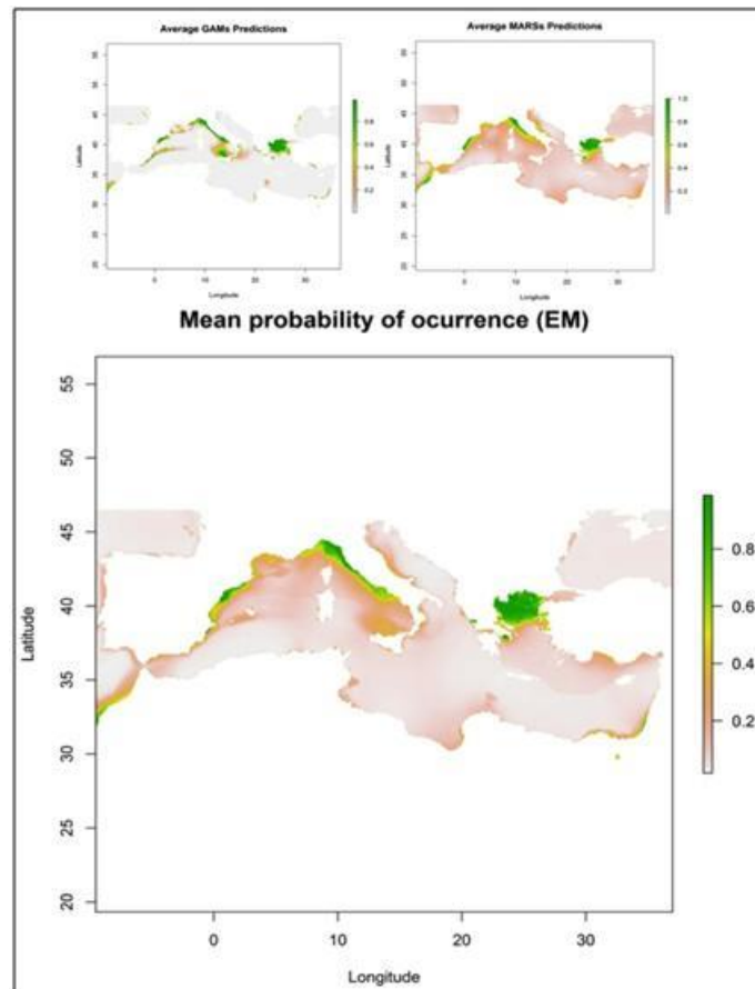
Figure 2. Suitable habitats for Mnemiopsis leidyi . Average prediction from GAM (upper-left panel) and MARS models (upper-right panel). Lower panel shows the ensemble forecasting for the potential distribution of M. leidyi in the Mediterranean Sea (Canepa et al. , 2013).
