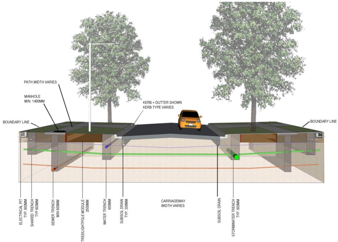
Figure 25-2 Typical Section
