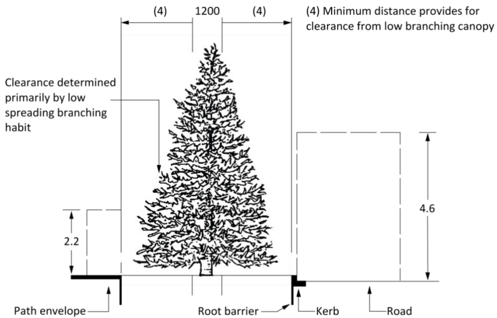
Figure 25-4 Tree shape categories clearance requirements – Category 3
