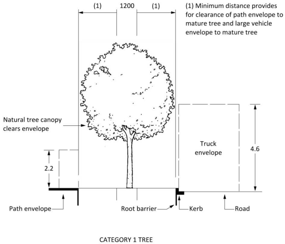
Figure 25-2 Tree shape categories clearance requirements – Category 1
