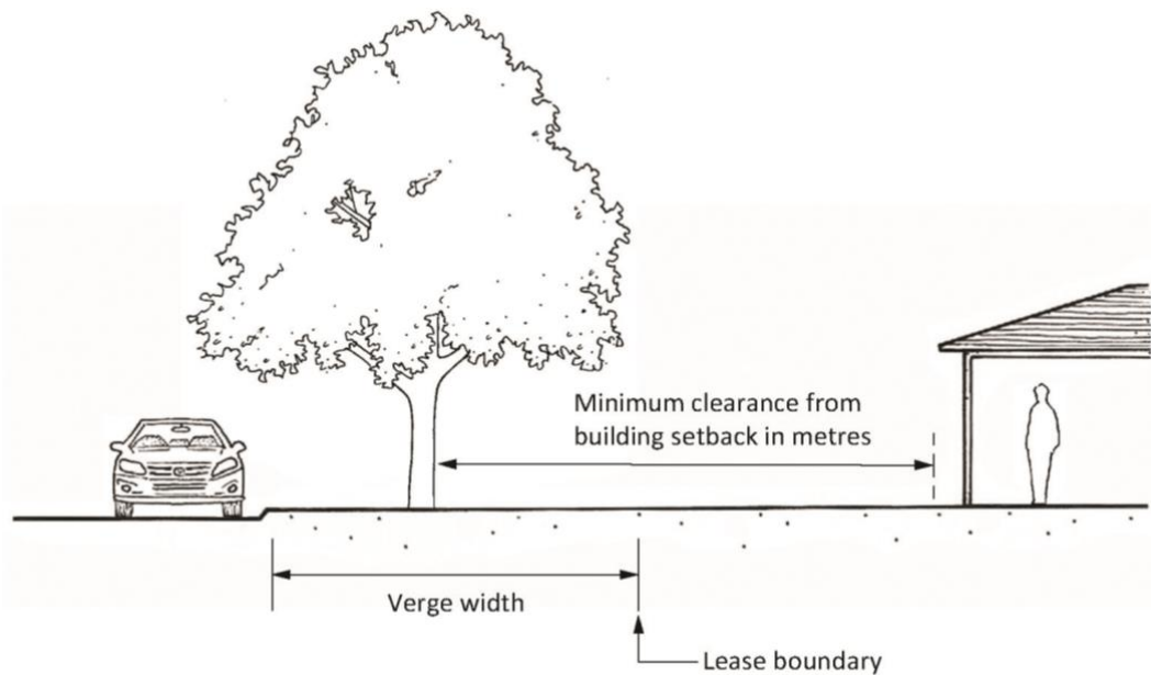
Figure 25-6 Minimum clearance from building setback
