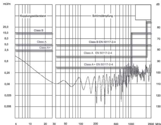
Messprotokoll | Measurement report (SAT KK 120-82)
