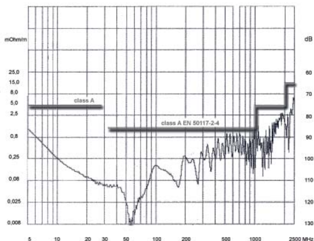
Messprotokoll | Measurement report (SAT KK 110-70)
