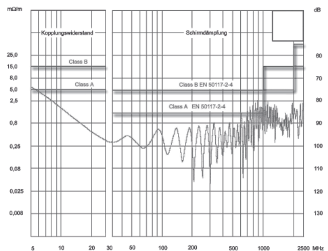
Messprotokoll | Measurement report (SAT KKS 100-68)
