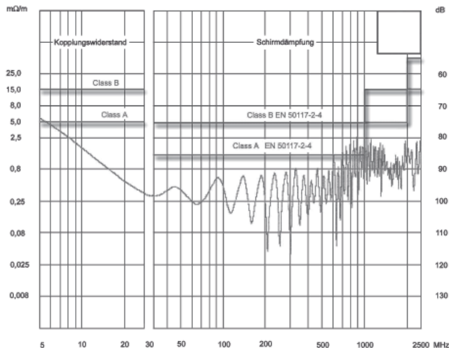
Messprotokoll | Measurement report (SAT KK 100-68)
