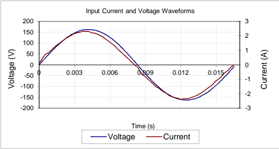
Input AC Current Waveform (ITHD = 1.89%, 50% Load)
